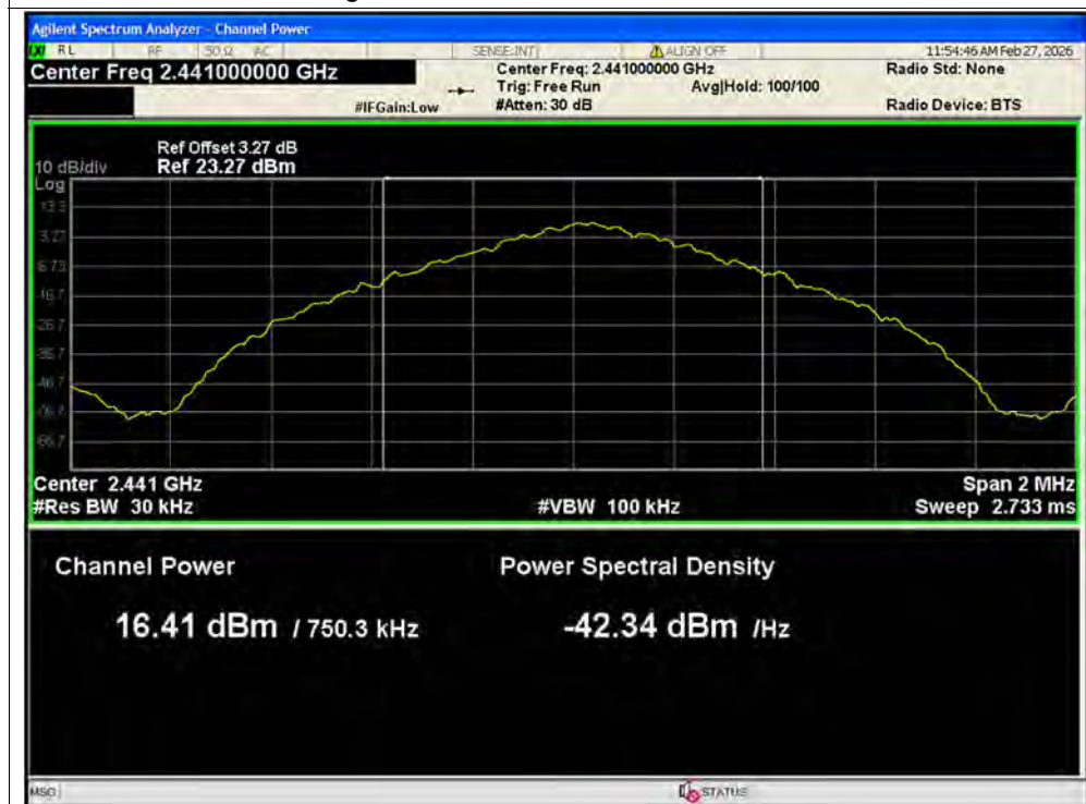
Average Power NVNT 1-DH5 2441MHz Ant1
