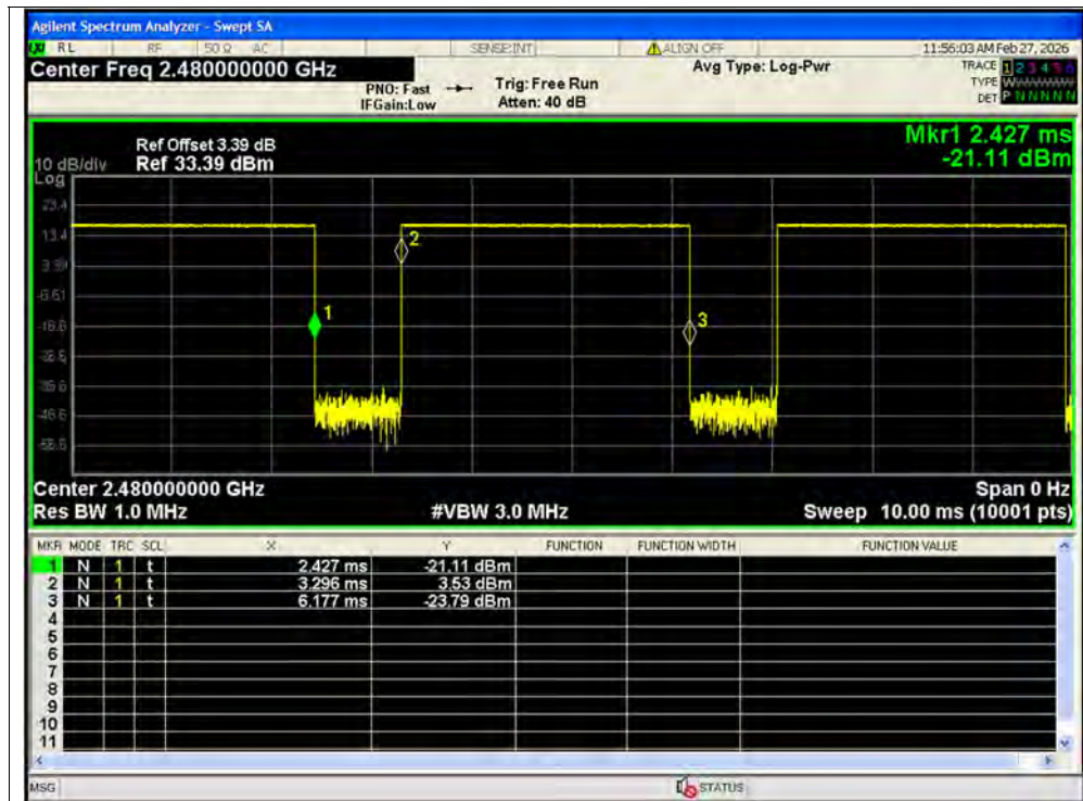
Duty Cycle NVNT 1-DH5 2480MHz Ant1
