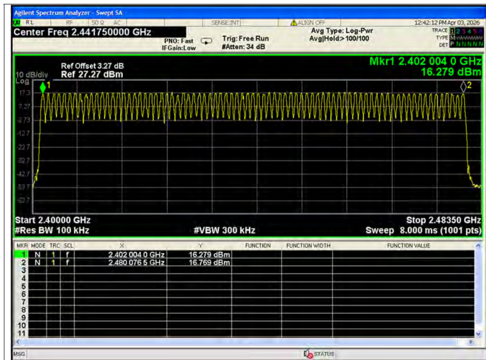
Hopping No. NVNT 1-DH5 2441MHz Ant1
