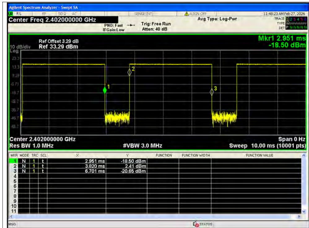
Duty Cycle NVNT 1-DH5 2402MHz Ant1
