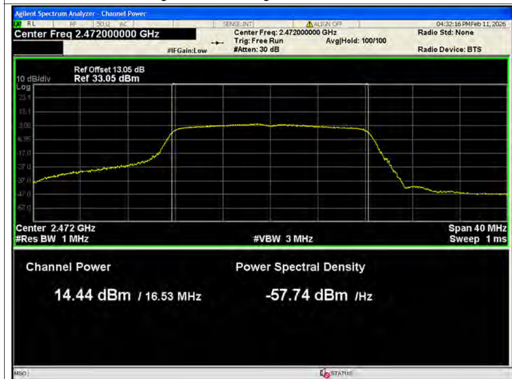
Average Power NVNT g 2472MHz Ant2 SISO
