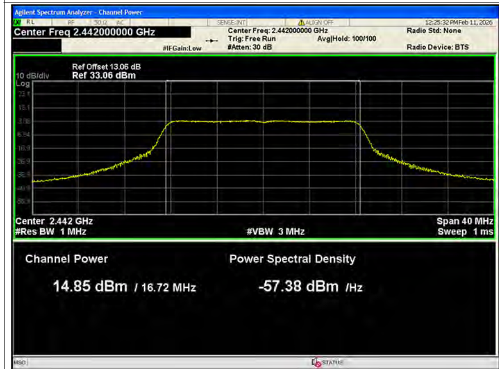
Average Power NVNT g 2442MHz Ant1 SISO
