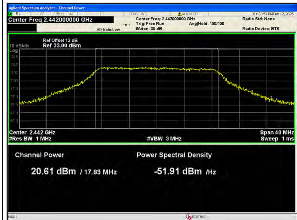
Peak Power NVNT n20 2442MHz Ant2 MIMO
