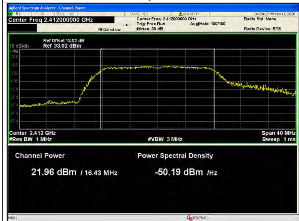
Peak Power NVNT g 2412MHz Ant2 SISO
