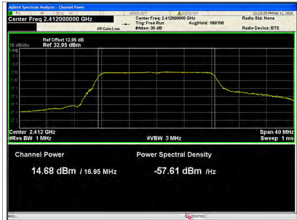
Average Power NVNT g 2412MHz Ant1 SISO
