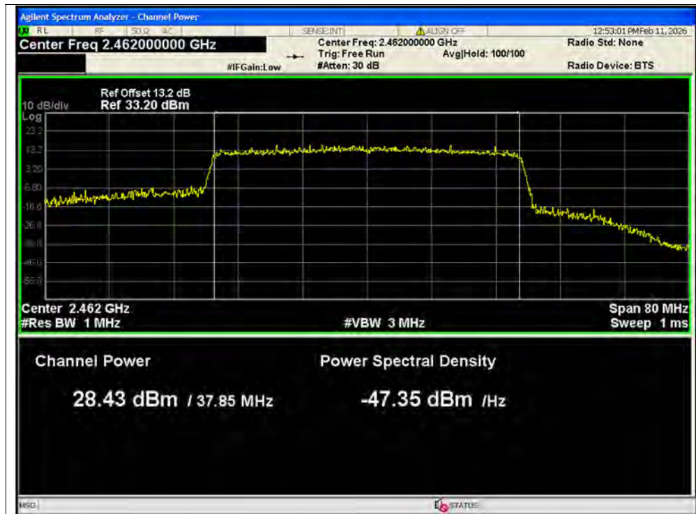
Peak Power NVNT ax40 2462MHz Ant1 SISO
