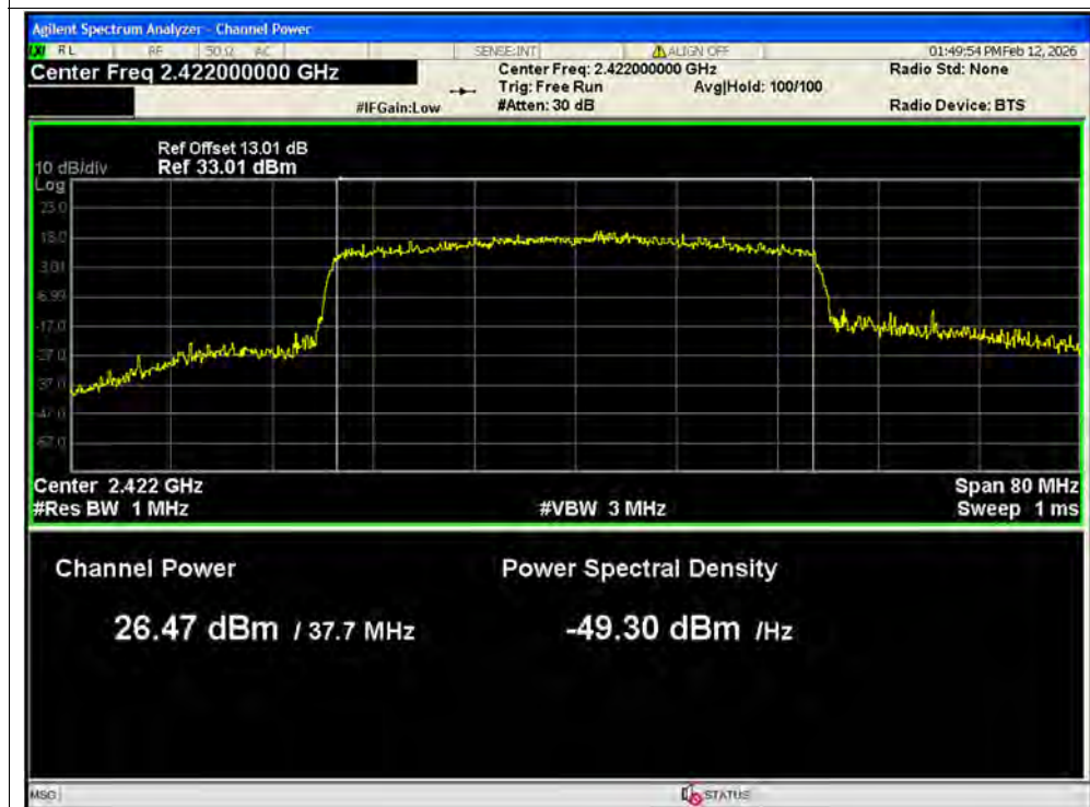
Peak Power NVNT ax40 2422MHz Ant2 MIMO
