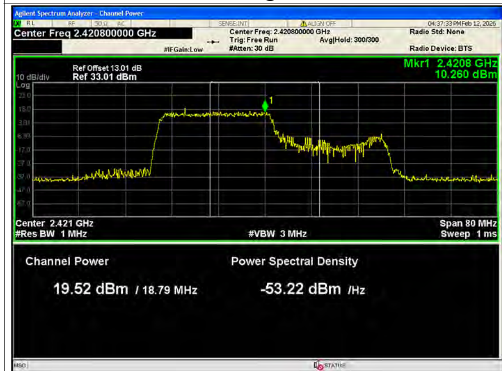
Peak Power NVNT ax40 242@61 2422MHz Ant2 MIMO
