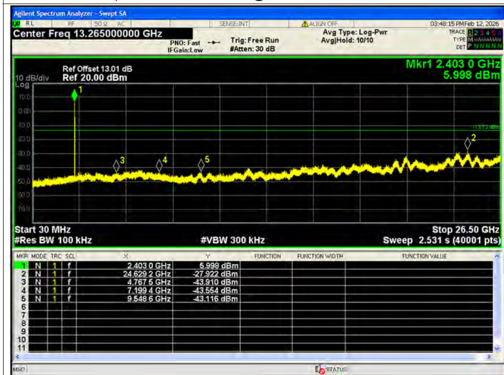
Tx. Spurious NVNT ax40 52@37 2422MHz Ant2 Emission SISO
