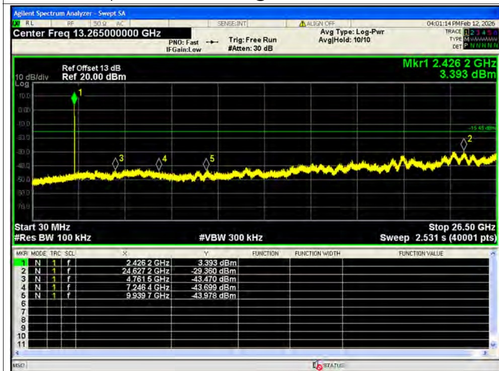
Tx. Spurious NVNT ax40 106@53 2442MHz Ant2 Emission SISO
