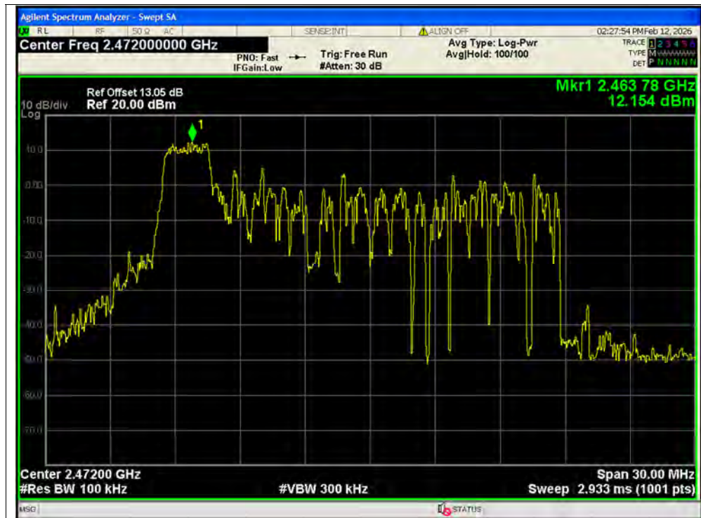
Band Edge NVNT ax20 26@0 2472MHz Ant2 Ref SISO
