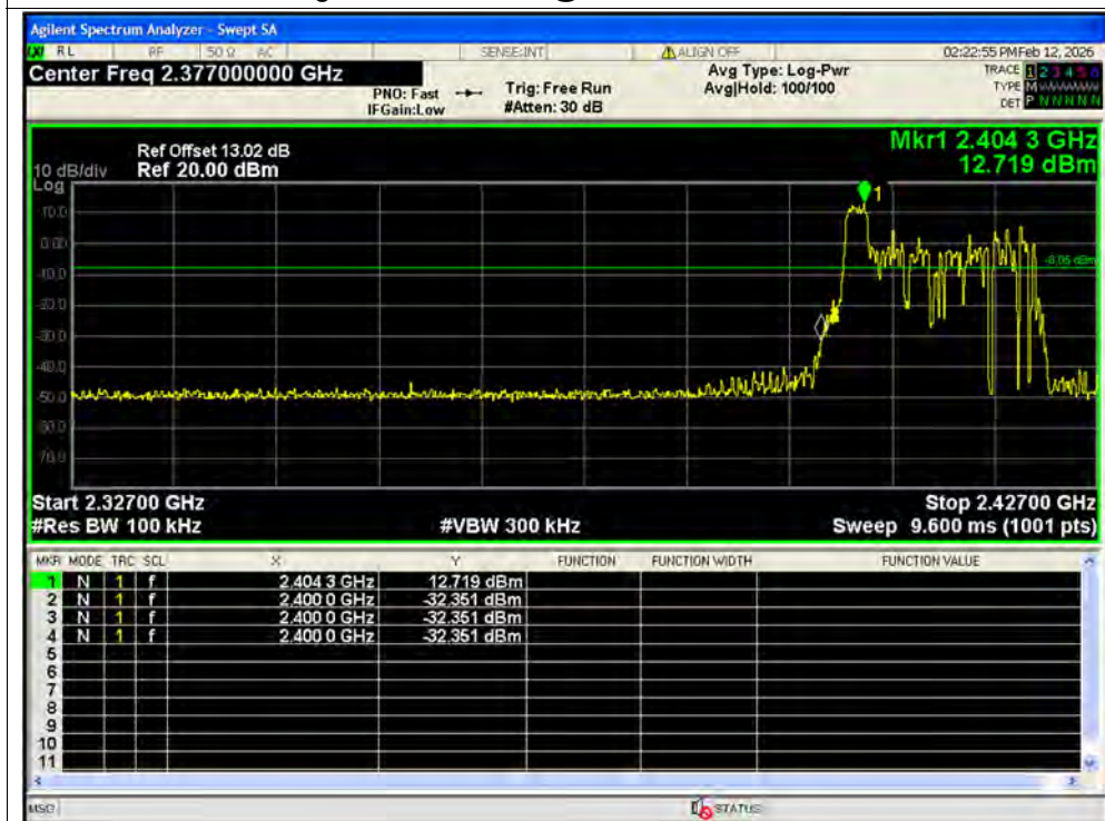
Band Edge NVNT ax20 26@0 2412MHz Ant2 Emission SISO
