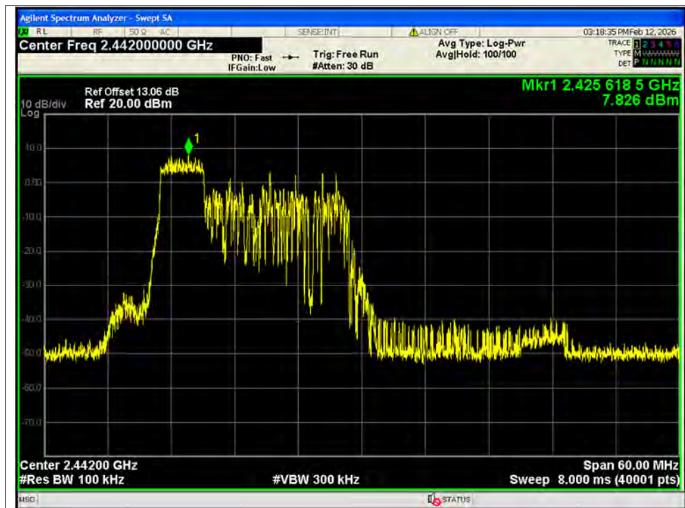
Tx. Spurious NVNT ax40 52@37 2442MHz Ant1 Ref SISO
