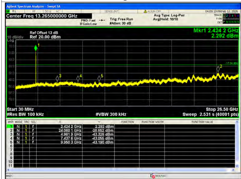
Tx. Spurious NVNT ax40 242@61 2442MHz Ant2 Emission SISO
