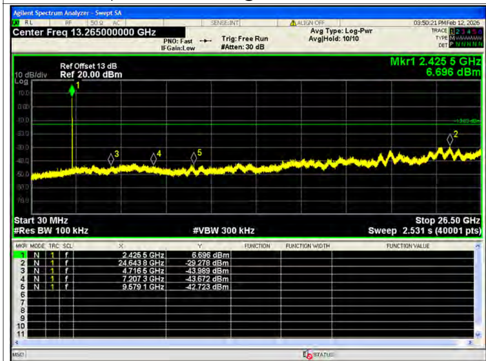
Tx. Spurious NVNT ax40 52@37 2442MHz Ant2 Emission SISO
