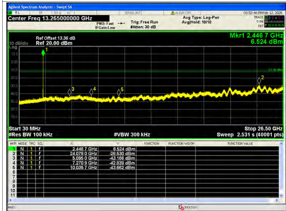
Tx. Spurious NVNT ax40 52@37 2462MHz Ant2 Emission SISO
