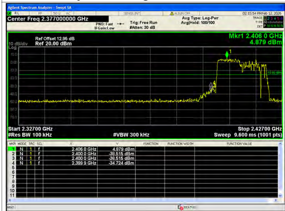
Band Edge NVNT ax20 106@53 2412MHz Ant1 Emission SISO
