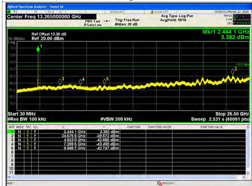
Tx. Spurious NVNT ax40 106@53 2462MHz Ant2 Emission SISO
