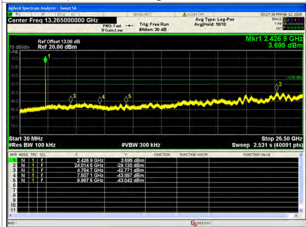
Tx. Spurious NVNT ax40 106@53 2442MHz Ant1 Emission SISO
