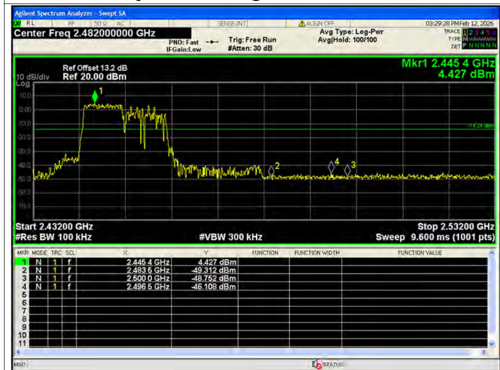
Band Edge NVNT ax40 106@53 2462MHz Ant1 Emission SISO
