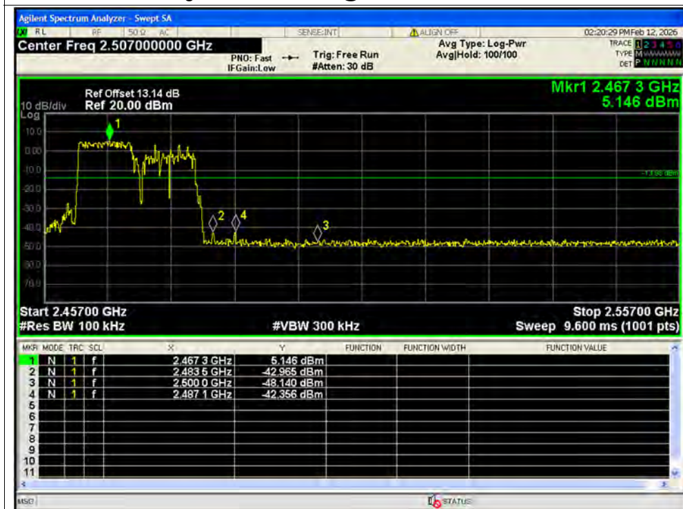
Band Edge NVNT ax20 106@53 2472MHz Ant1 Emission SISO
