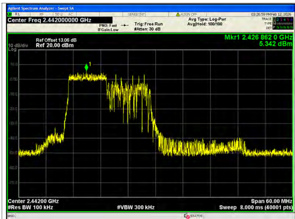
Tx. Spurious NVNT ax40 106@53 2442MHz Ant1 Ref SISO
