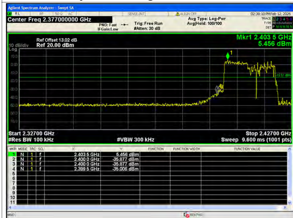
Band Edge NVNT ax20 106@53 2412MHz Ant2 Emission SISO
