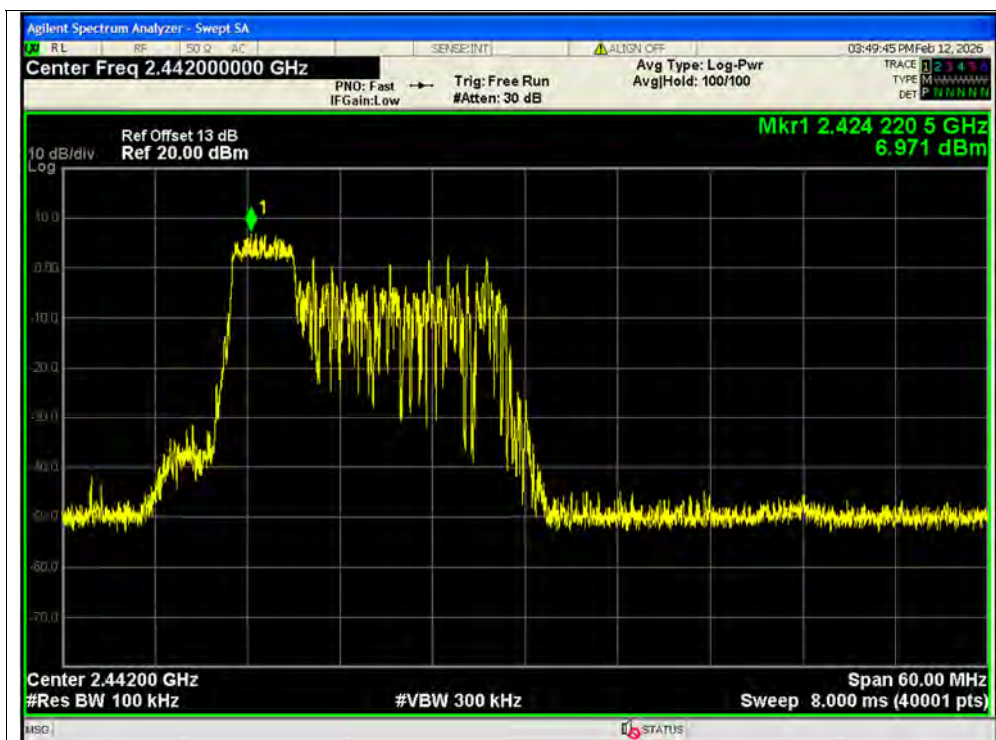
Tx. Spurious NVNT ax40 52@37 2442MHz Ant2 Ref SISO
