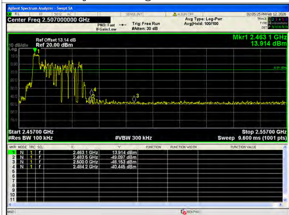
Band Edge NVNT ax20 26@0 2472MHz Ant1 Emission SISO
