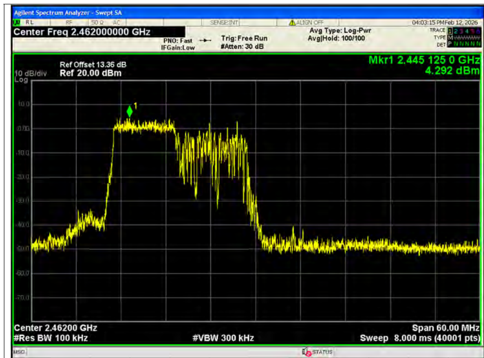
Tx. Spurious NVNT ax40 106@53 2462MHz Ant2 Ref SISO
