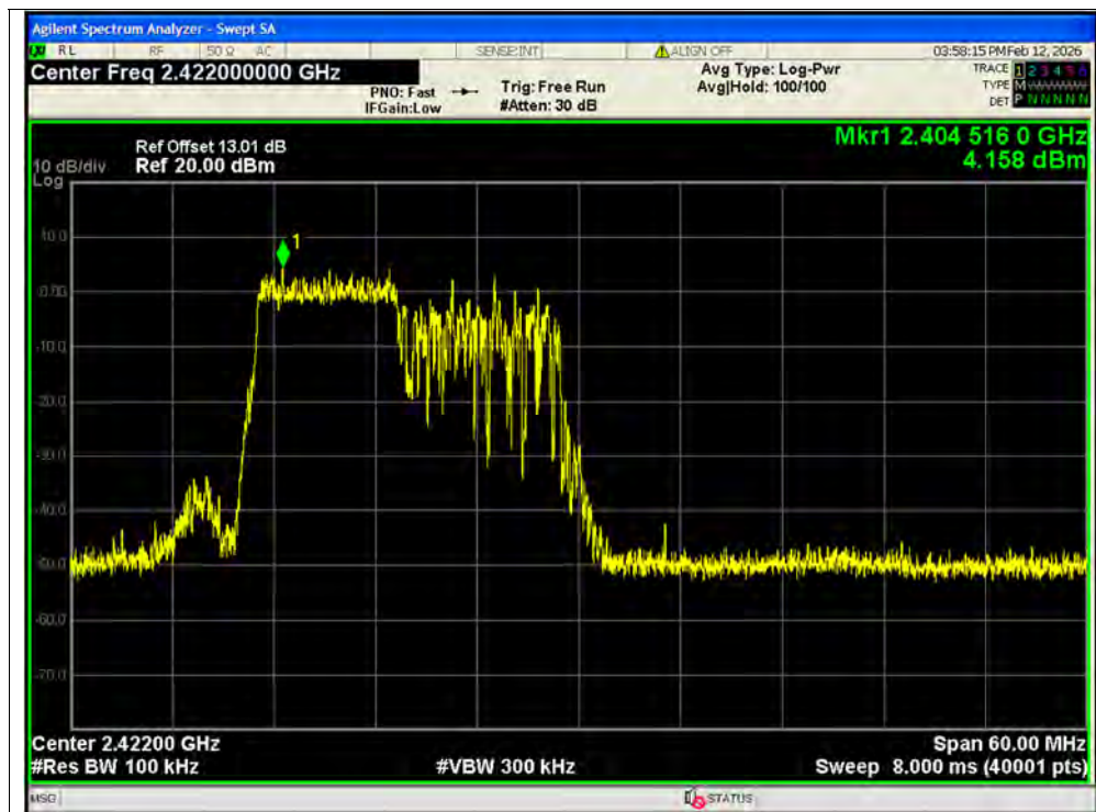
Tx. Spurious NVNT ax40 106@53 2422MHz Ant2 Ref SISO
