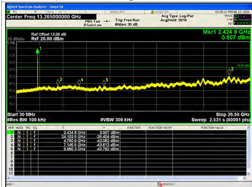
Tx. Spurious NVNT ax40 242@61 2442MHz Ant1 Emission SISO
