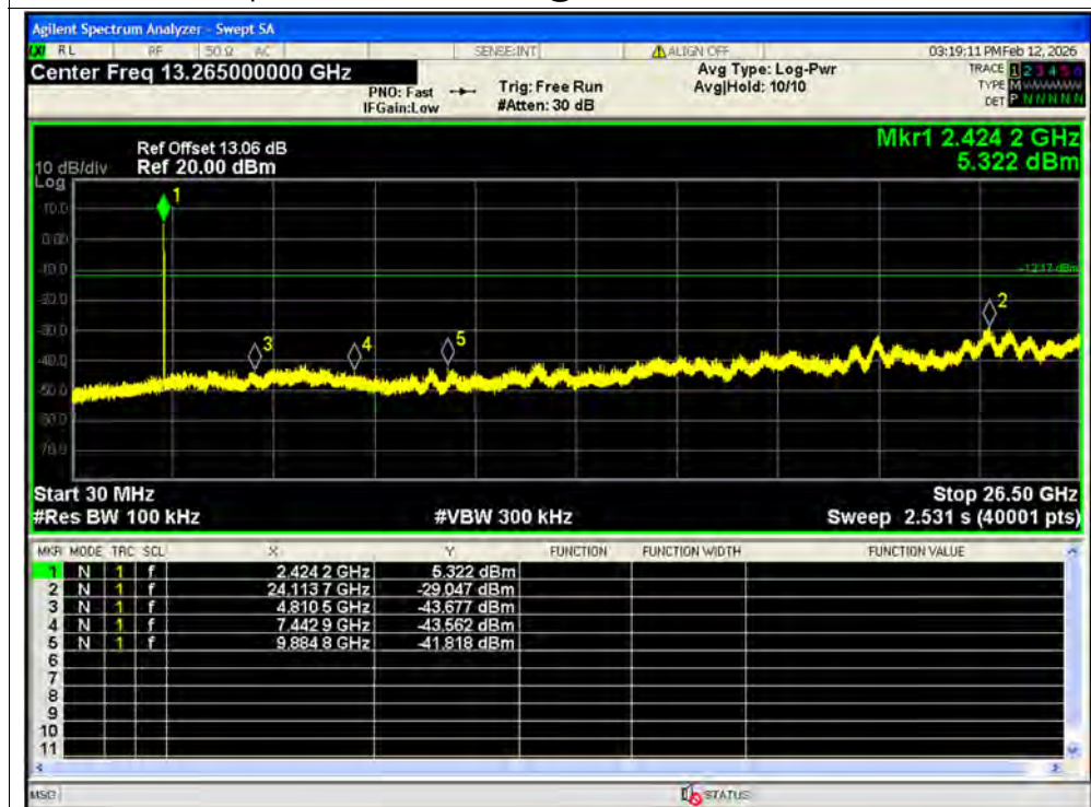
Tx. Spurious NVNT ax40 52@37 2442MHz Ant1 Emission SISO
