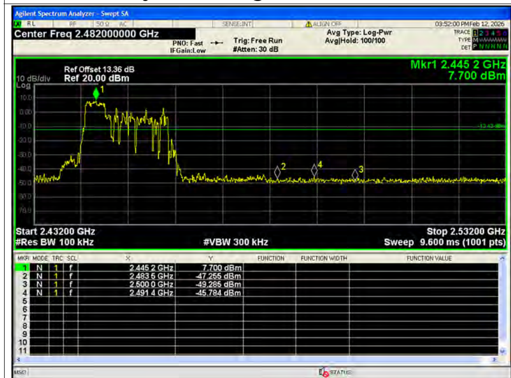
Band Edge NVNT ax40 52@37 2462MHz Ant2 Emission SISO
