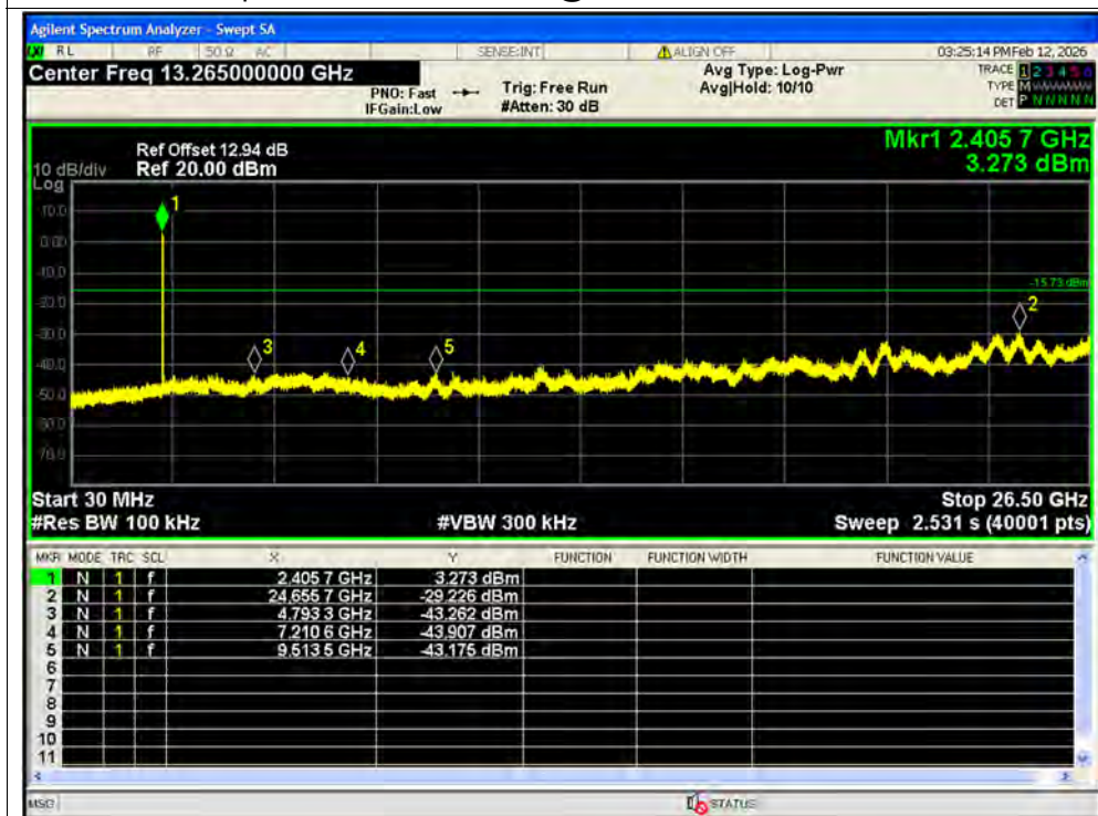
Tx. Spurious NVNT ax40 106@53 2422MHz Ant1 Emission SISO
