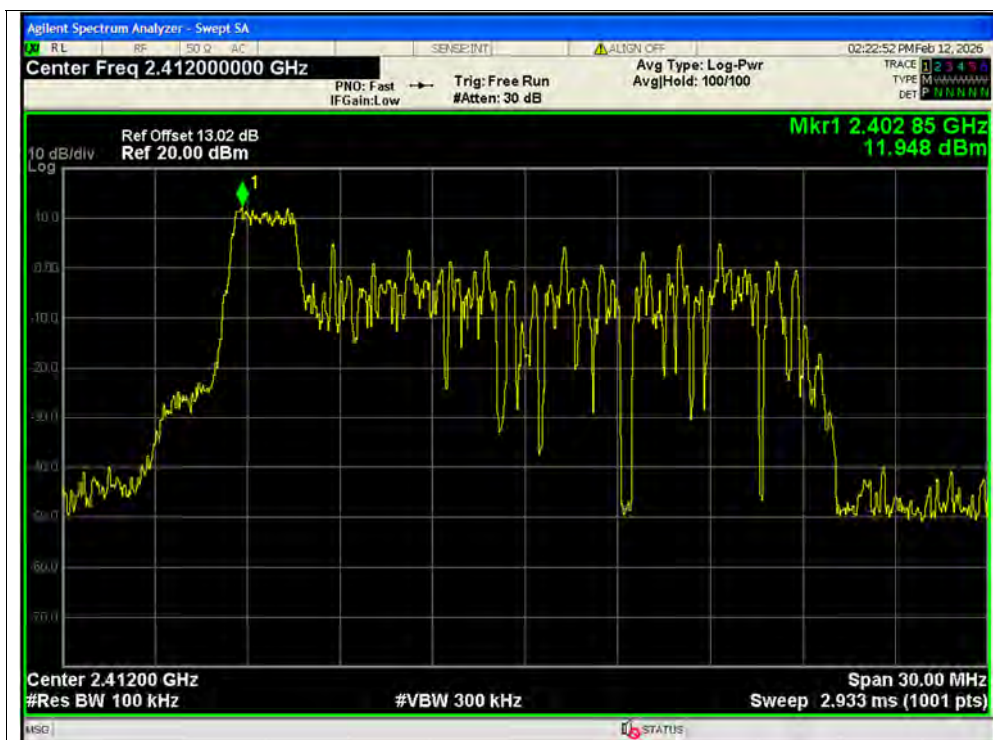
Band Edge NVNT ax20 26@0 2412MHz Ant2 Ref SISO
