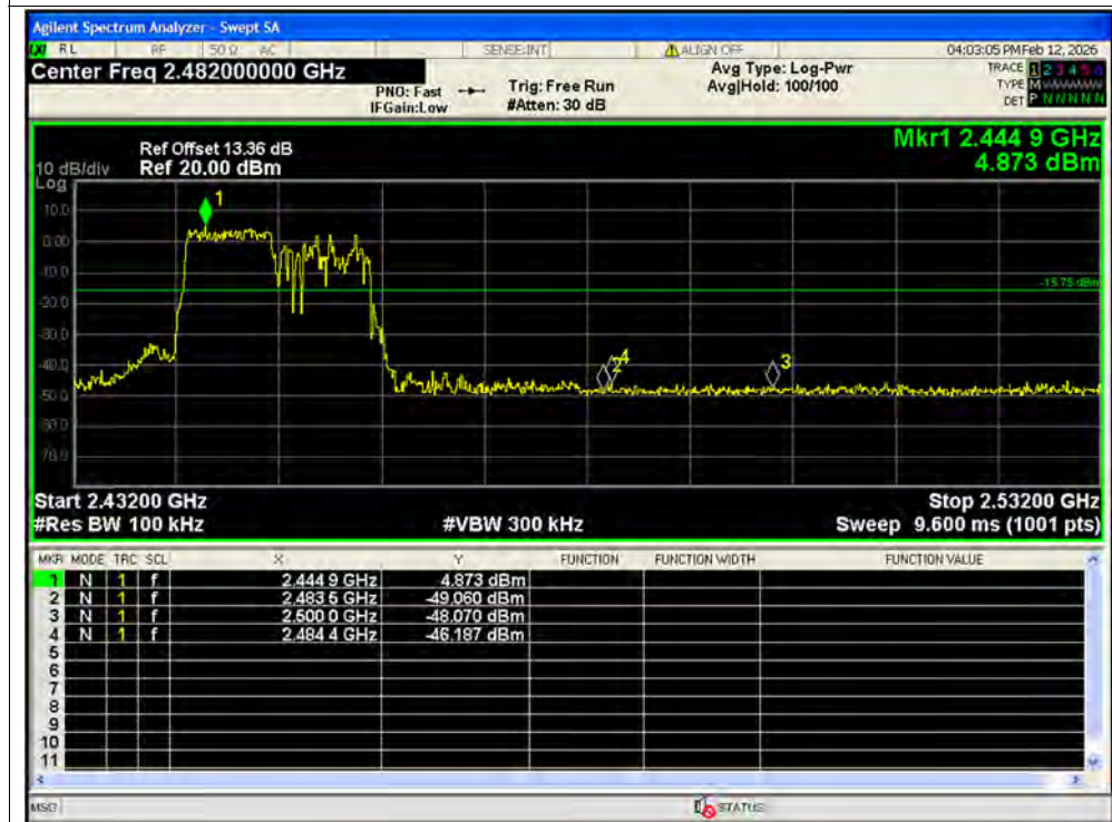
Band Edge NVNT ax40 106@53 2462MHz Ant2 Emission SISO
