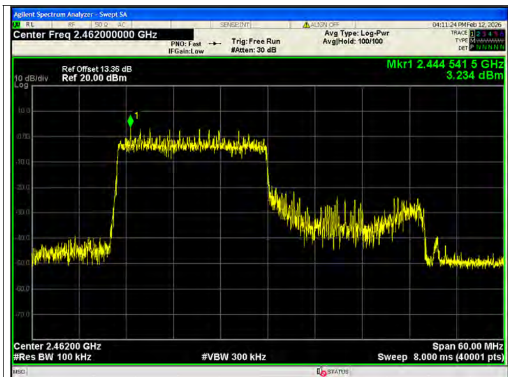
Tx. Spurious NVNT ax40 242@61 2462MHz Ant2 Ref SISO
