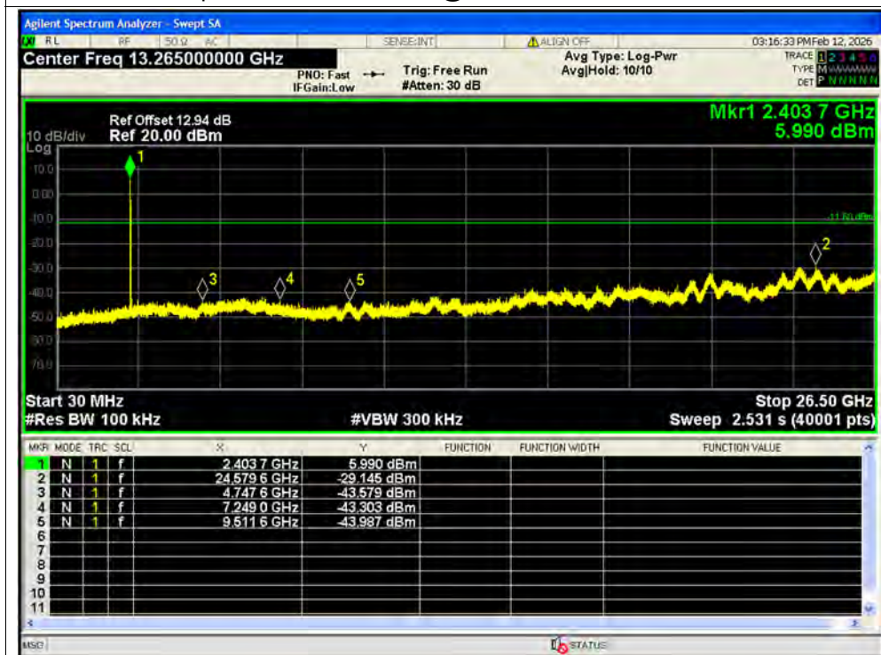
Tx. Spurious NVNT ax40 52@37 2422MHz Ant1 Emission SISO
