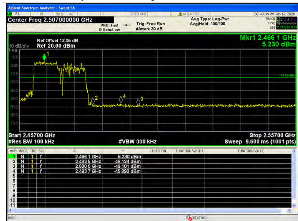
Band Edge NVNT ax20 106@53 2472MHz Ant2 Emission SISO
