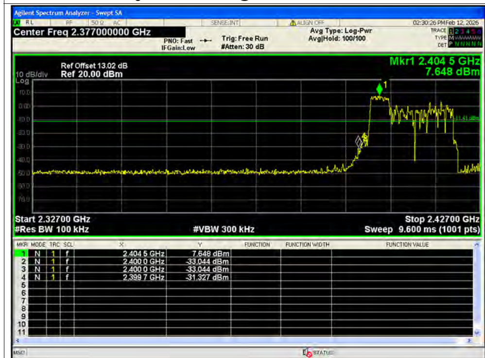
Band Edge NVNT ax20 52@37 2412MHz Ant2 Emission SISO
