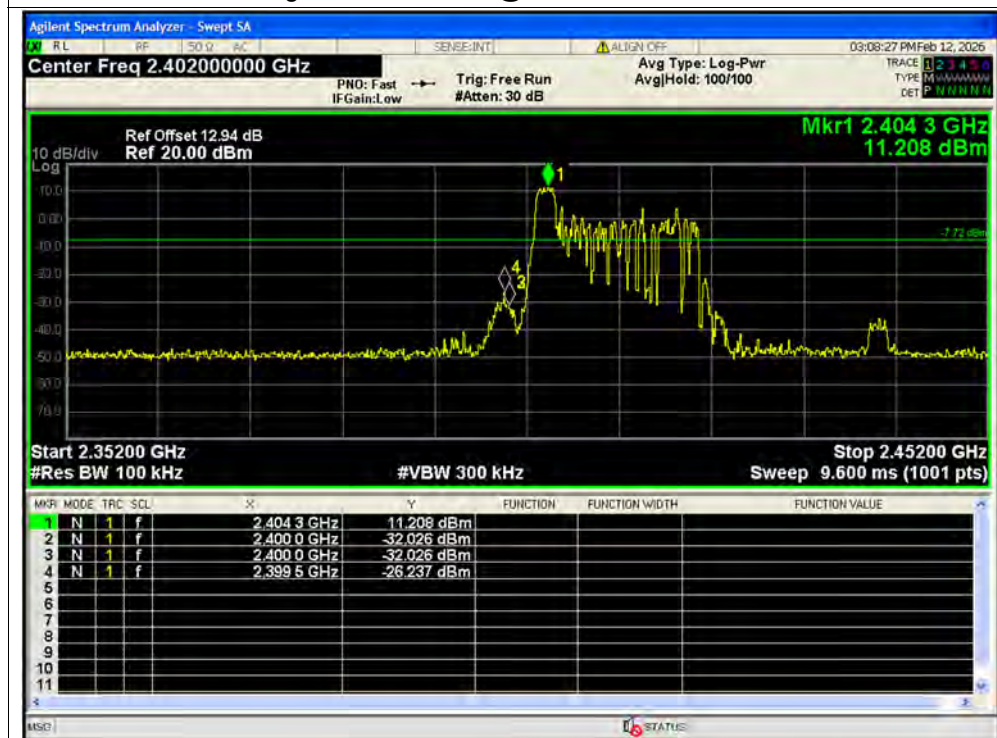
Band Edge NVNT ax40 26@0 2422MHz Ant1 Emission SISO
