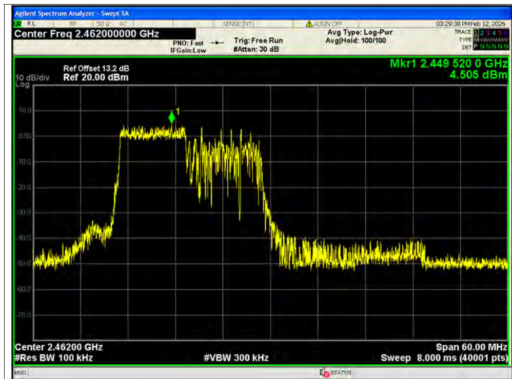
Tx. Spurious NVNT ax40 106@53 2462MHz Ant1 Ref SISO
