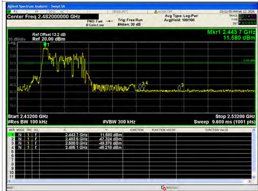
Band Edge NVNT ax40 26@0 2462MHz Ant1 Emission SISO
