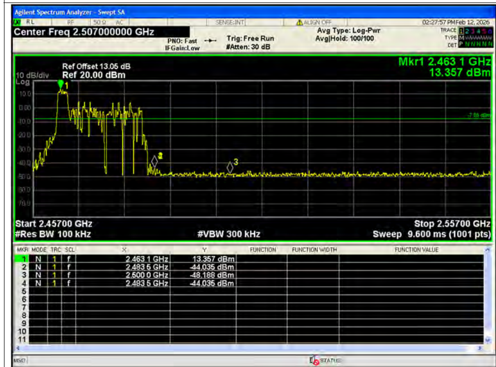
Band Edge NVNT ax20 26@0 2472MHz Ant2 Emission SISO
