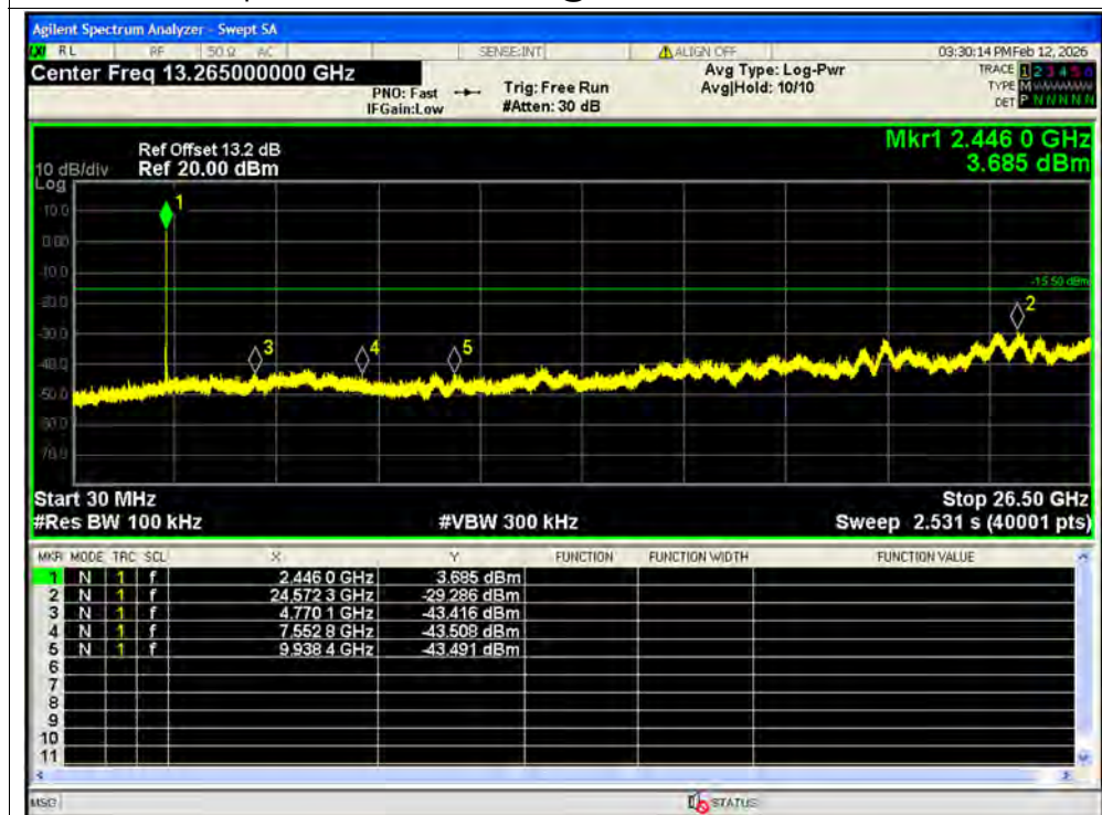
Tx. Spurious NVNT ax40 106@53 2462MHz Ant1 Emission SISO
