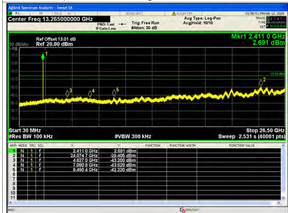
Tx. Spurious NVNT ax40 106@53 2422MHz Ant2 Emission SISO
