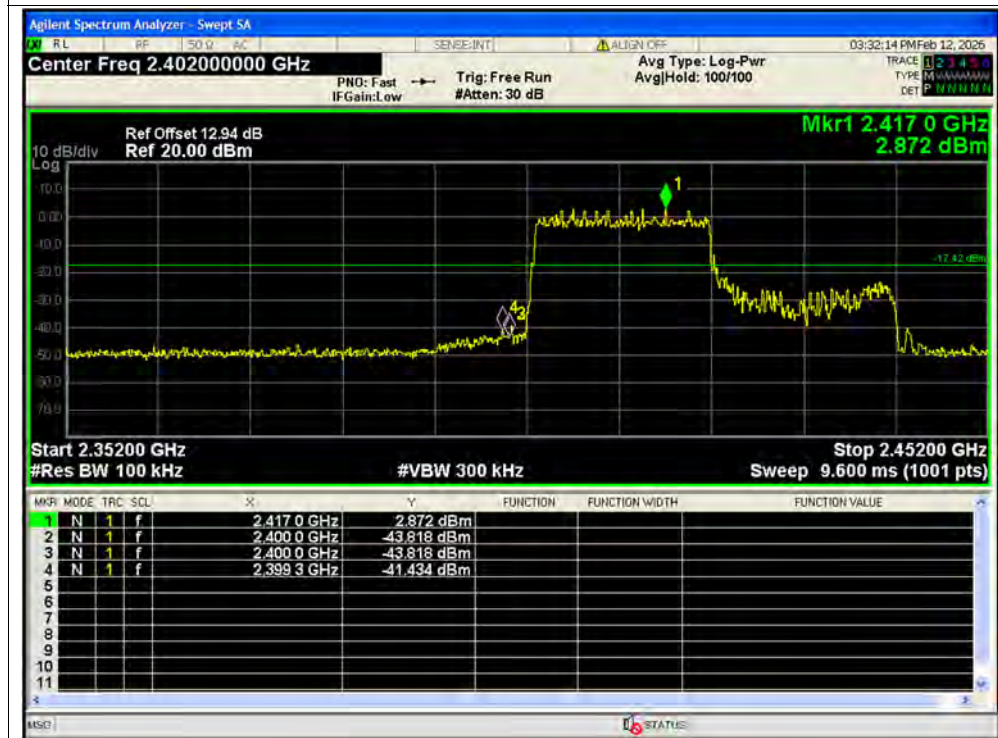
Band Edge NVNT ax40 242@61 2422MHz Ant1 Emission SISO
