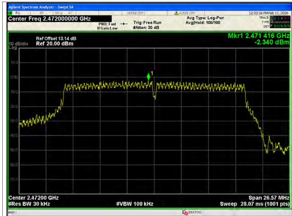
PSD NVNT n20 2472MHz Ant1 SISO
