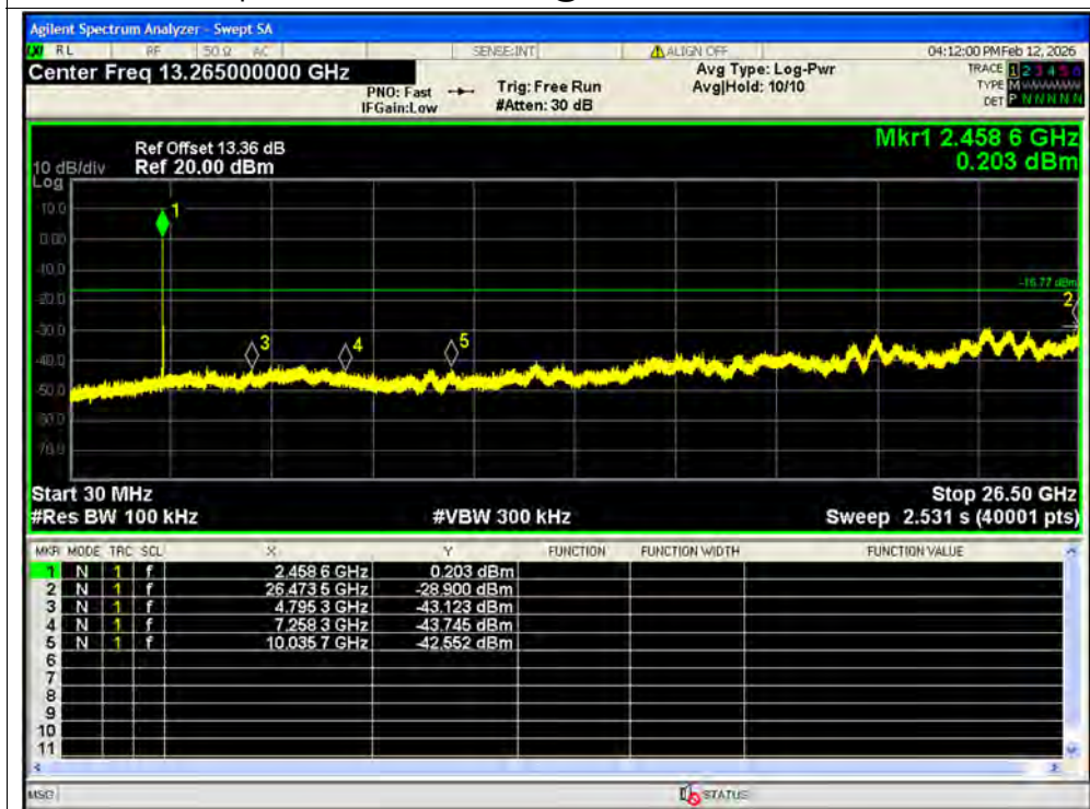
Tx. Spurious NVNT ax40 242@61 2462MHz Ant2 Emission SISO
