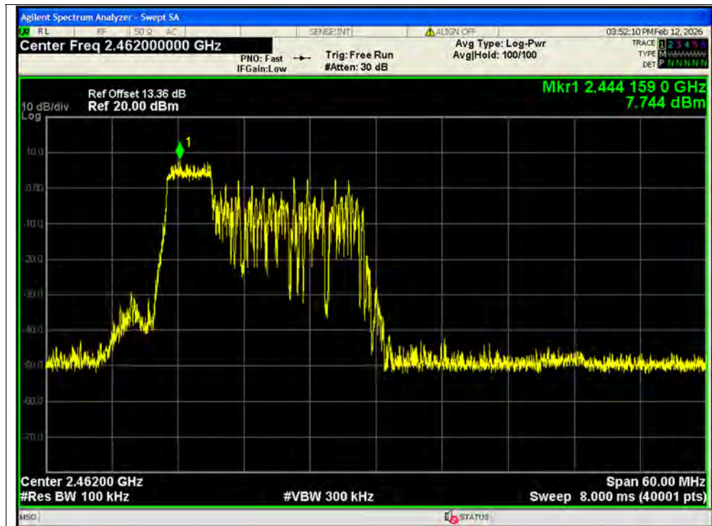
Tx. Spurious NVNT ax40 52@37 2462MHz Ant2 Ref SISO
