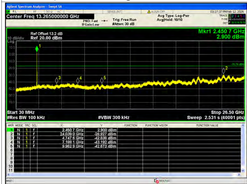
Tx. Spurious NVNT ax40 242@61 2462MHz Ant1 Emission SISO
