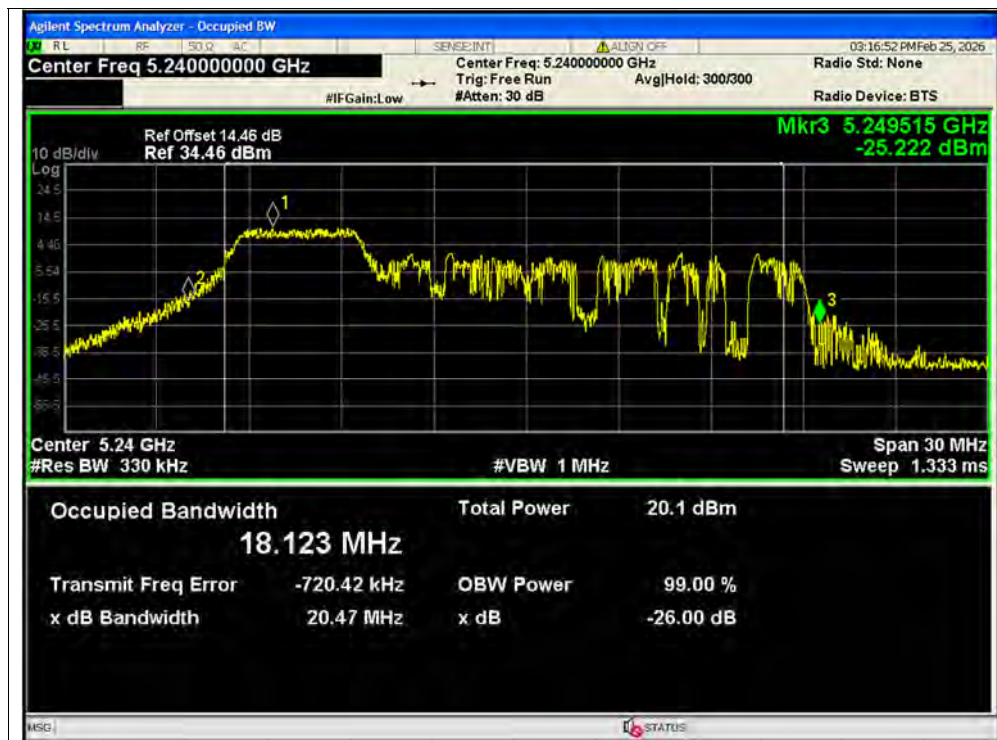
-26dB Bandwidth NVNT ax20 52@1 5240MHz Ant1 MIMO
