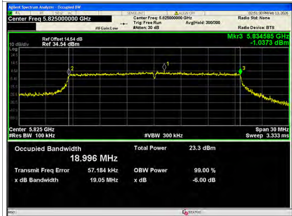
-6dB Bandwidth NVNT ax20 5825MHz Ant2 SISO
