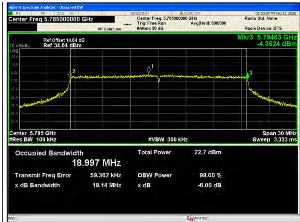
-6dB Bandwidth NVNT ax20 5785MHz Ant2 SISO
