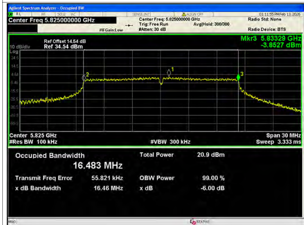
-6dB Bandwidth NVNT a 5825MHz Ant2 SISO
