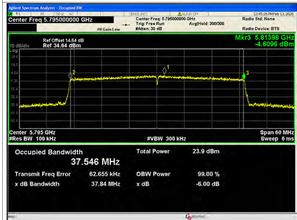
-6dB Bandwidth NVNT ax40 5795MHz Ant1 SISO
