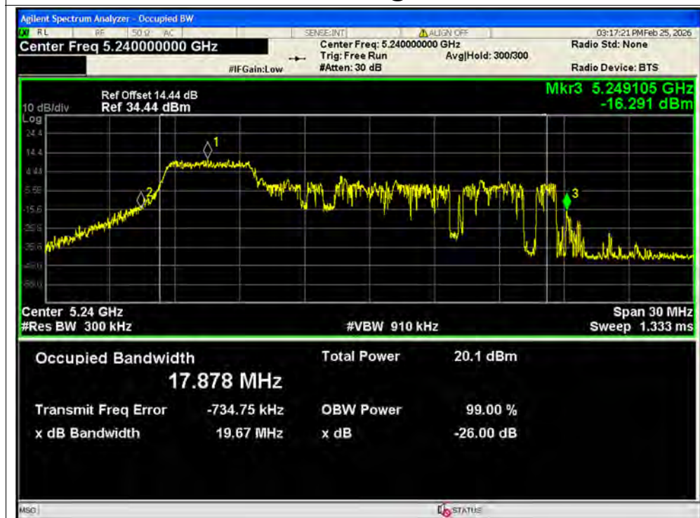
-26dB Bandwidth NVNT ax20 52@1 5240MHz Ant2 MIMO
