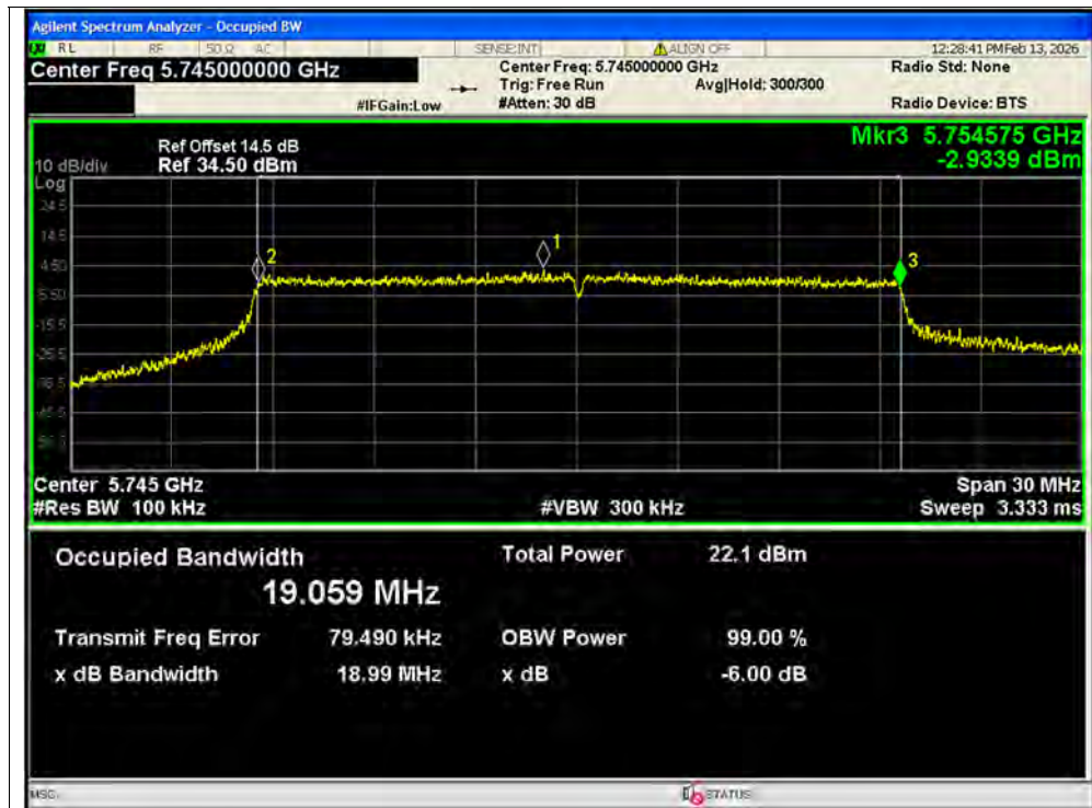
-6dB Bandwidth NVNT ax20 5745MHz Ant1 SISO
