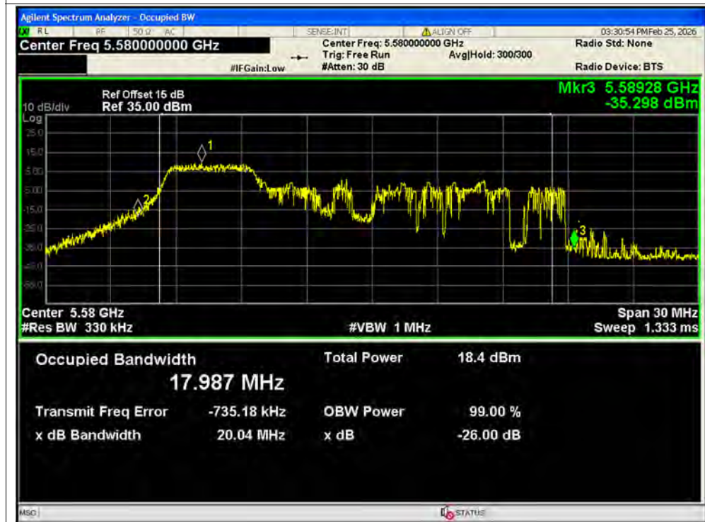
-26dB Bandwidth NVNT ax20 52@1 5580MHz Ant2 MIMO
