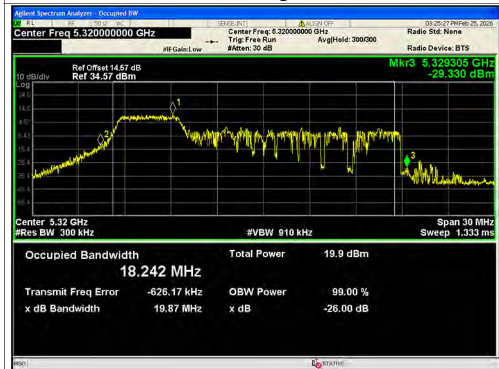
-26dB Bandwidth NVNT ax20 52@1 5320MHz Ant2 MIMO
