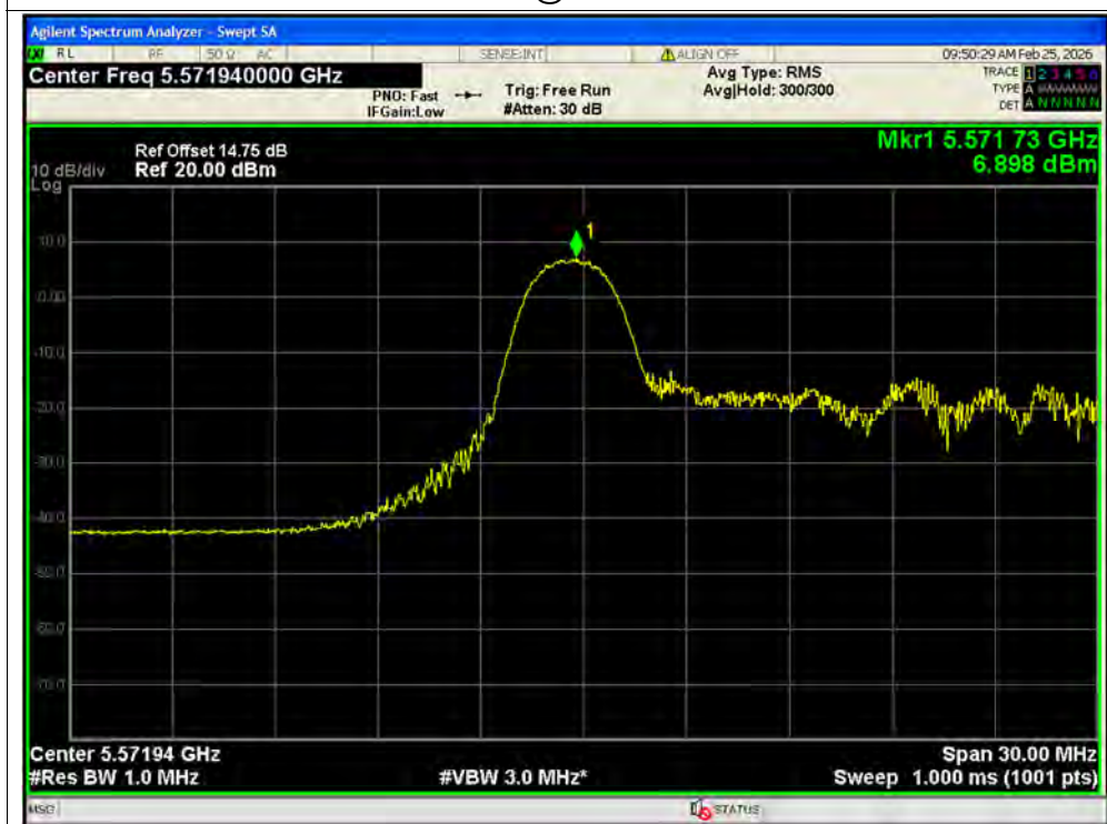
PSD NVNT ax20 26@1 5580MHz Ant1 SISO
