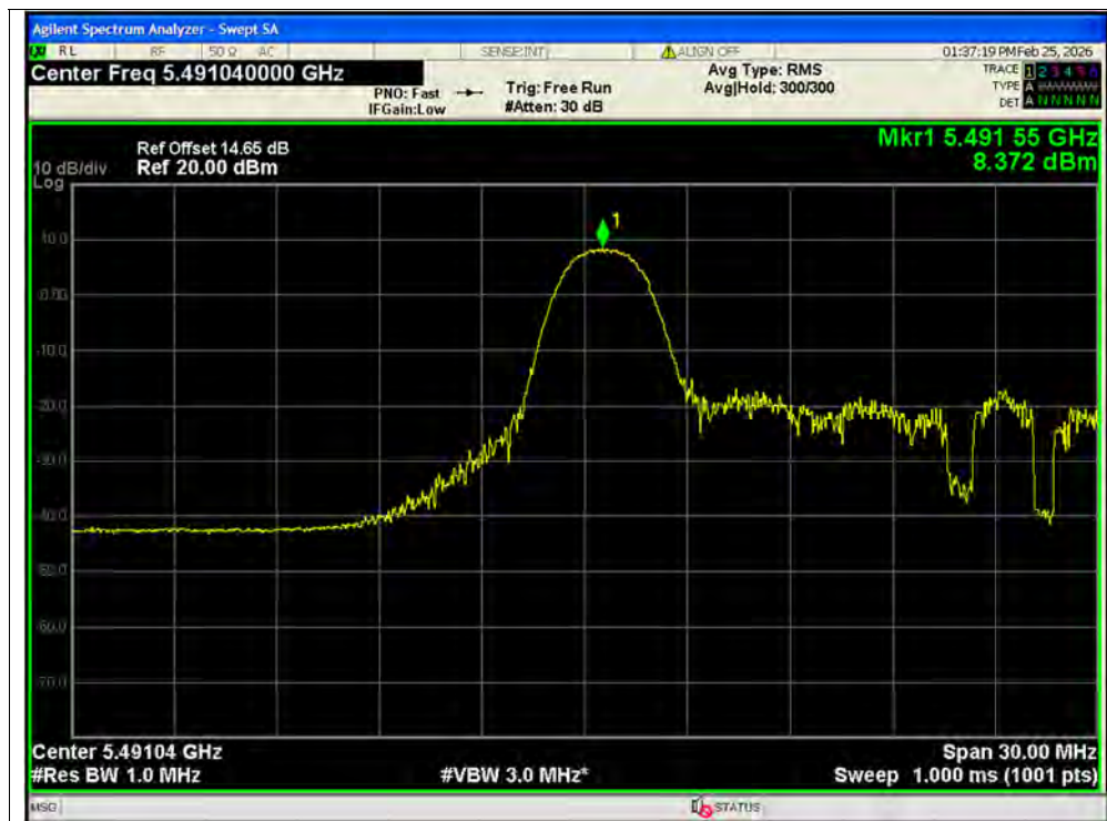
PSD NVNT ax20 26@1 5500MHz Ant2 SISO
