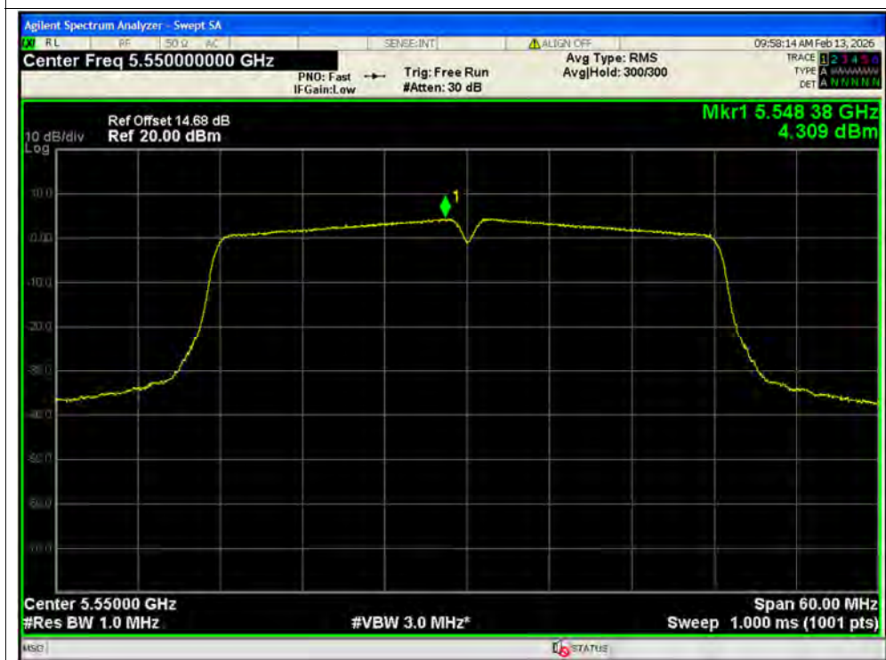
PSD NVNT ac40 5550MHz Ant1 SISO
