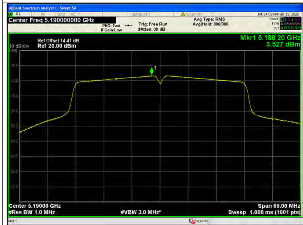
PSD NVNT ac40 5190MHz Ant2 MIMO
