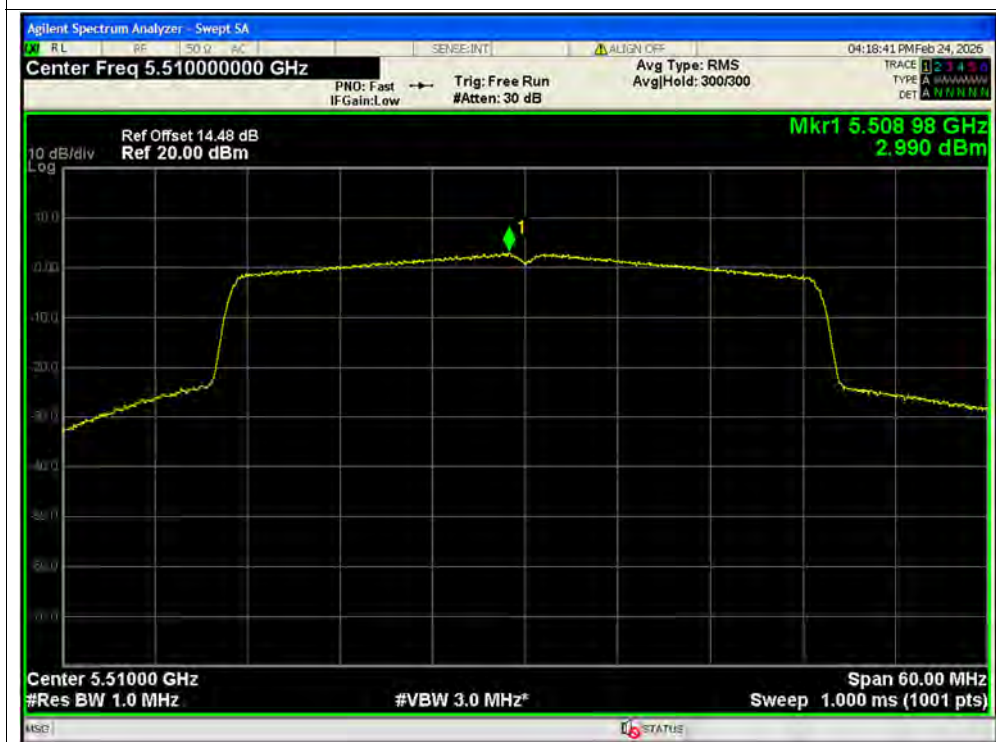
PSD NVNT ax40 5510MHz Ant2 MIMO
