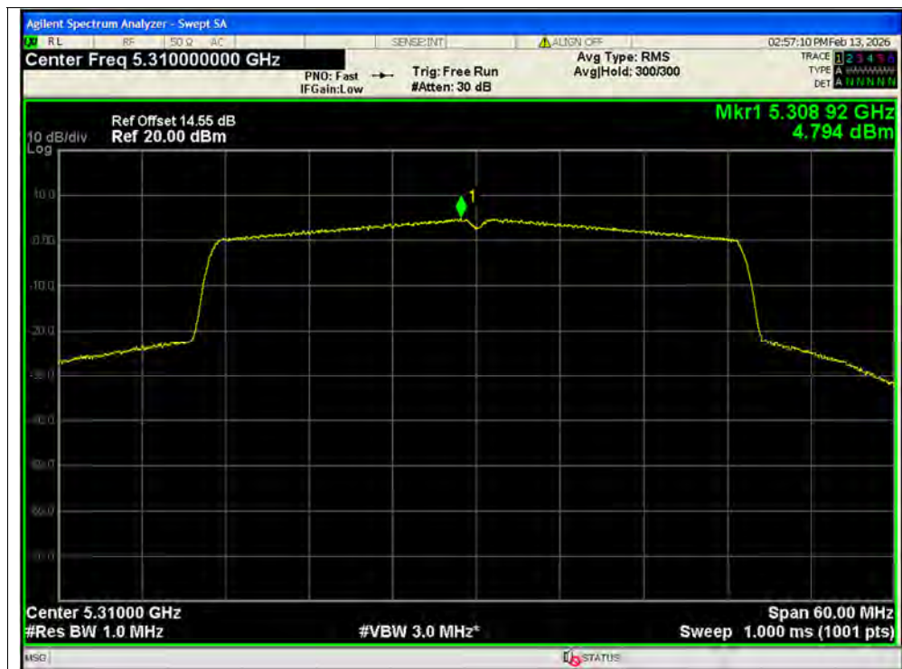
PSD NVNT ax40 5310MHz Ant2 SISO
