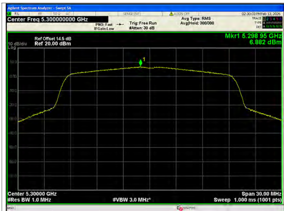
PSD NVNT ax20 5300MHz Ant2 SISO
