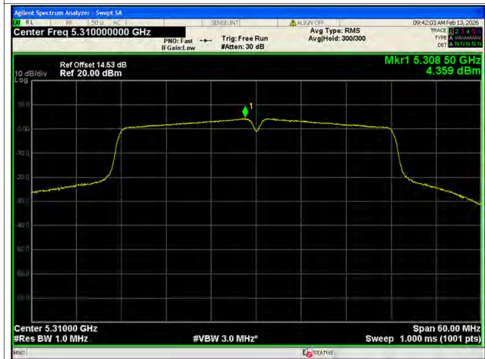
PSD NVNT ac40 5310MHz Ant1 SISO
