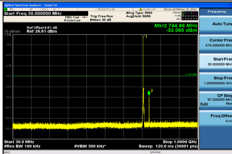
Band12-1.4MHz-16QAM-23173-1RB#0-30~1000MHz
