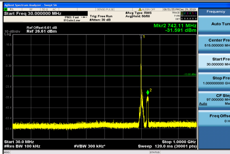
Band12-10MHz-QPSK-23130-1RB#0-30~1000MHz
