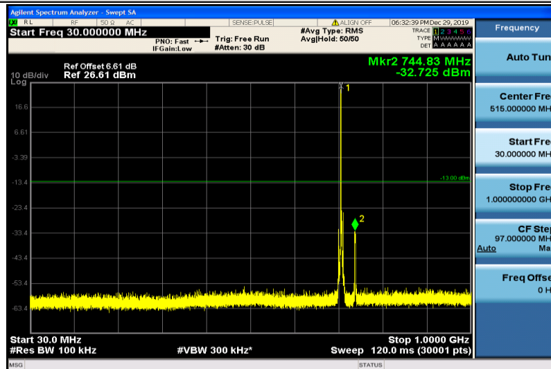
Band12-3MHz-16QAM-23165-1RB#0-30~1000MHz
