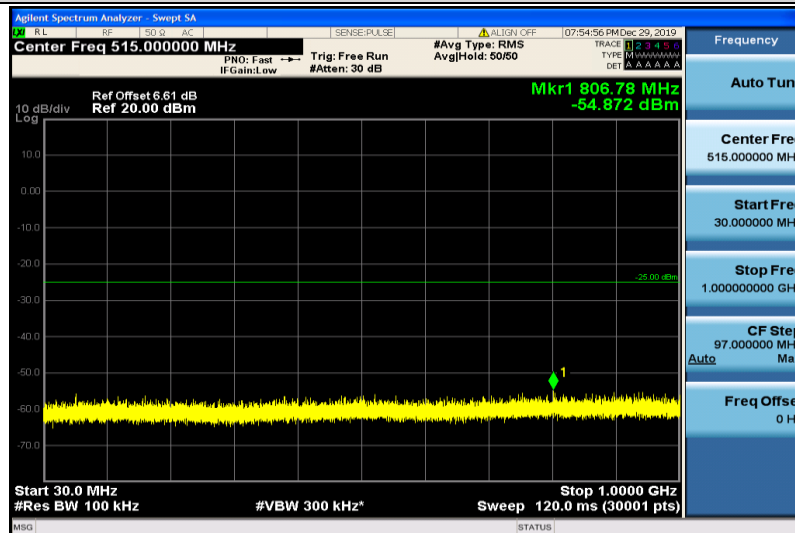
Band41-15MHz-QPSK-41165-1RB#0-30~1000MHz
