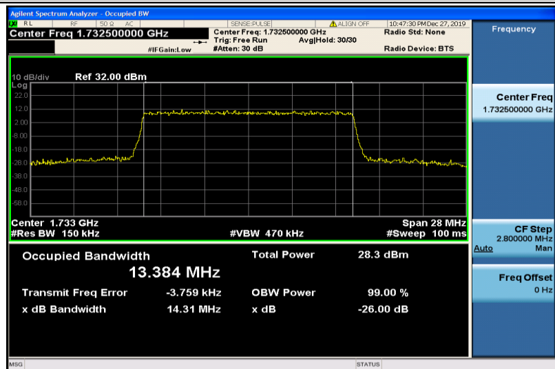
Band4-15MHz-16QAM-20175-75RB#0-13.384
