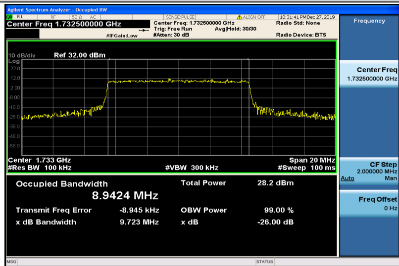
Band4-10MHz-16QAM-20175-50RB#0-8.9424
