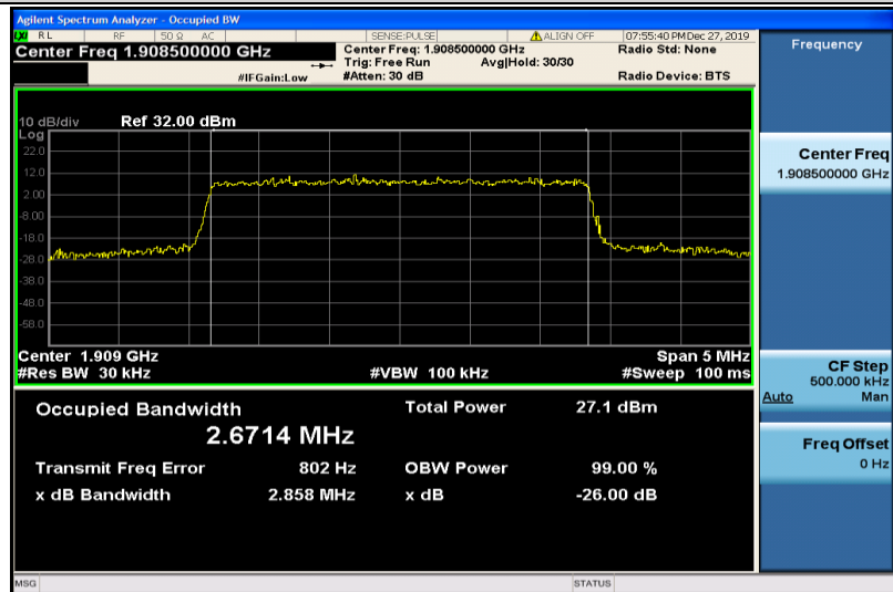
Band2-3MHz-16QAM-19185-15RB#0-2.6714
