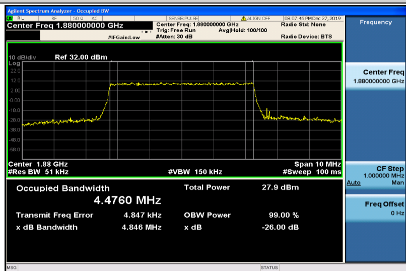
Band2-5MHz-16QAM-18900-25RB#0-4.4760
