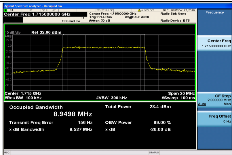
Band4-10MHz-16QAM-20000-50RB#0-8.9498
