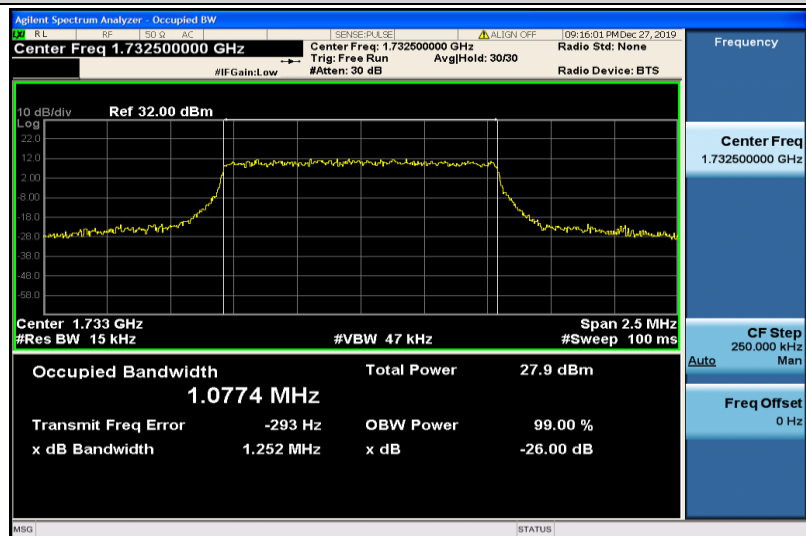
Band4-1.4MHz-QPSK-20175-6RB#0-1.0774
