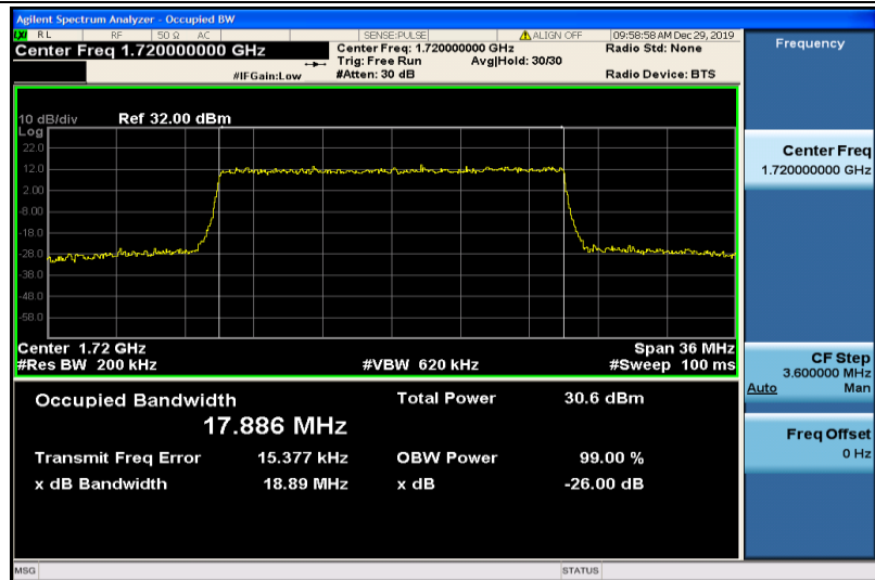
Band4-20MHz-QPSK-20050-100RB#0-17.886
