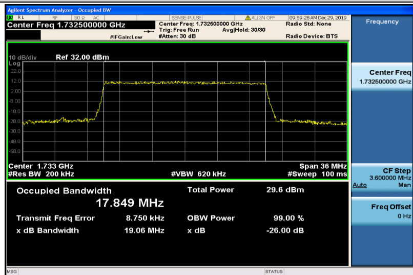
Band4-20MHz-16QAM-20175-100RB#0-17.849
