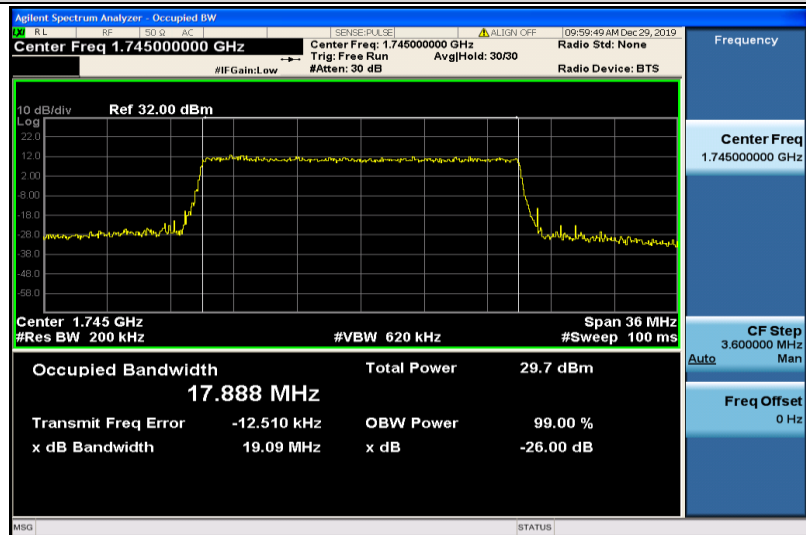
Band4-20MHz-16QAM-20300-100RB#0-17.888
