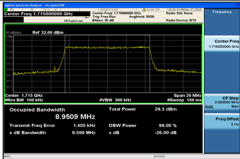
Band4-10MHz-QPSK-20000-50RB#0-8.9509
