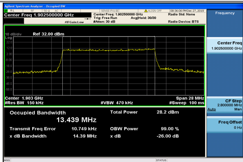
Band2-15MHz-16QAM-19125-75RB#0-13.439
