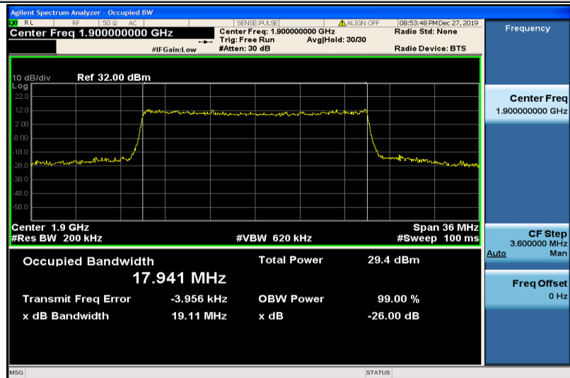
Band2-20MHz-QPSK-19100-100RB#0-17.941
