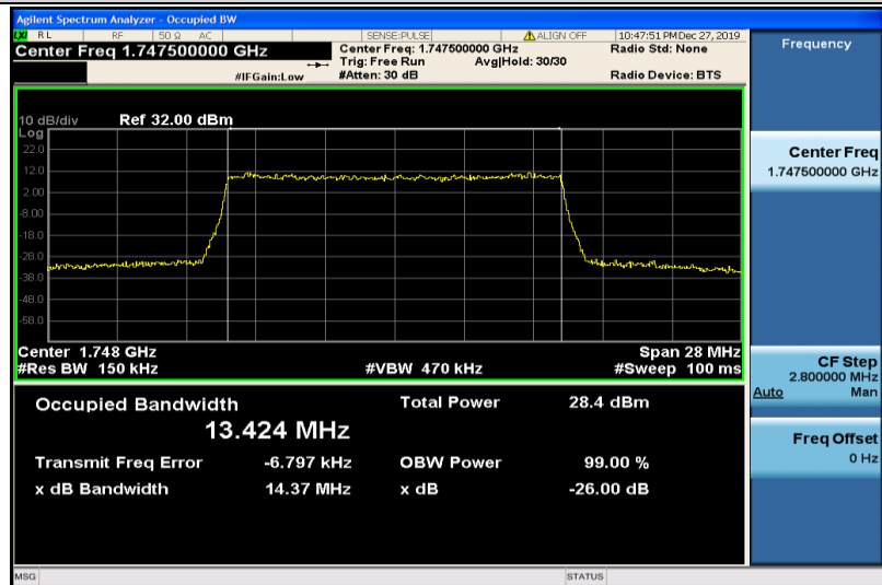
Band4-15MHz-16QAM-20325-75RB#0-13.424
