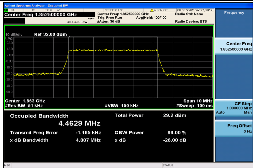
Band2-5MHz-QPSK-18625-25RB#0-4.4629
