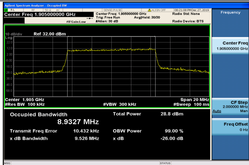
Band2-10MHz-QPSK-19150-50RB#0-8.9327
