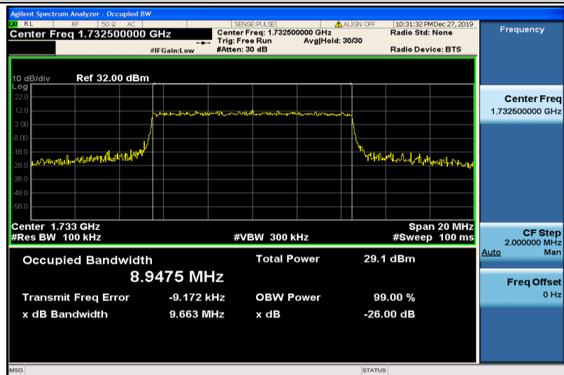
Band4-10MHz-QPSK-20175-50RB#0-8.9475
