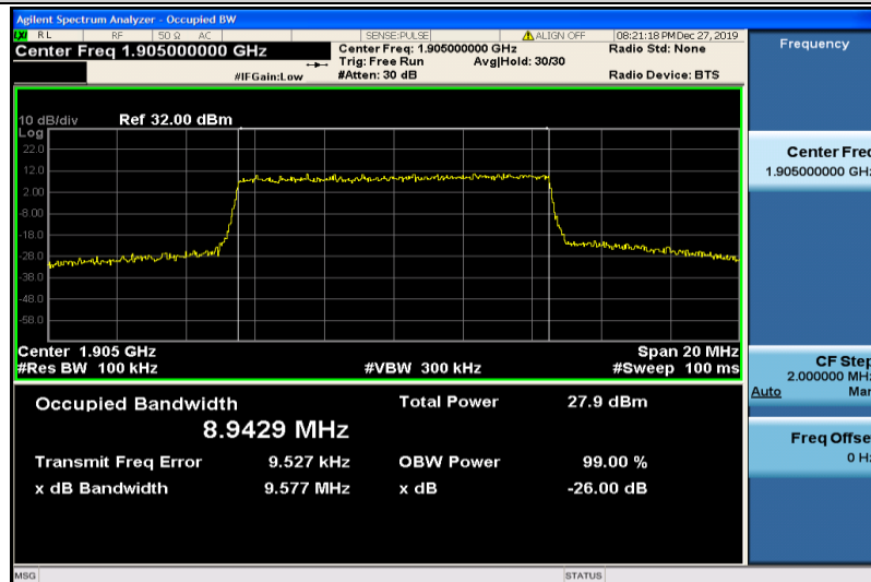
Band2-10MHz-16QAM-19150-50RB#0-8.9429
