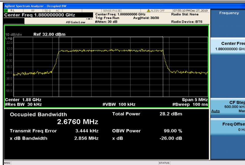
Band2-3MHz-QPSK-18900-15RB#0-2.6760
