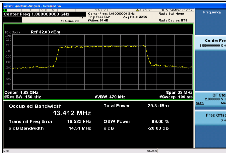
Band2-15MHz-QPSK-18900-75RB#0-13.412
