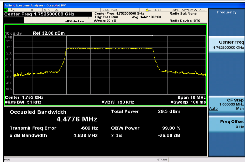
Band4-5MHz-QPSK-20375-25RB#0-4.4776
