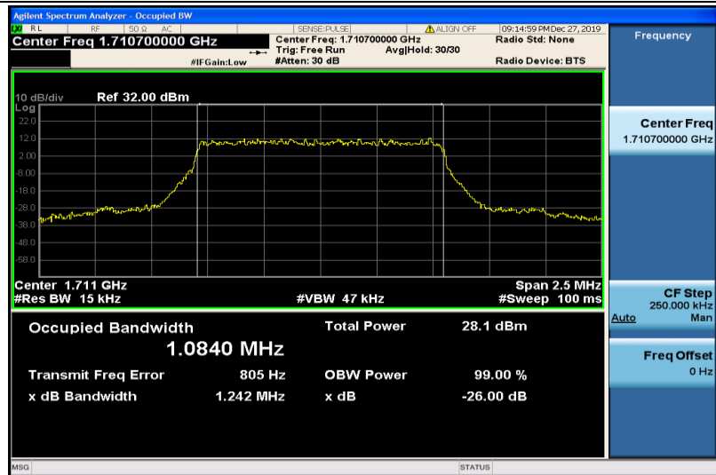
Band4-1.4MHz-QPSK-19957-6RB#0-1.0840
