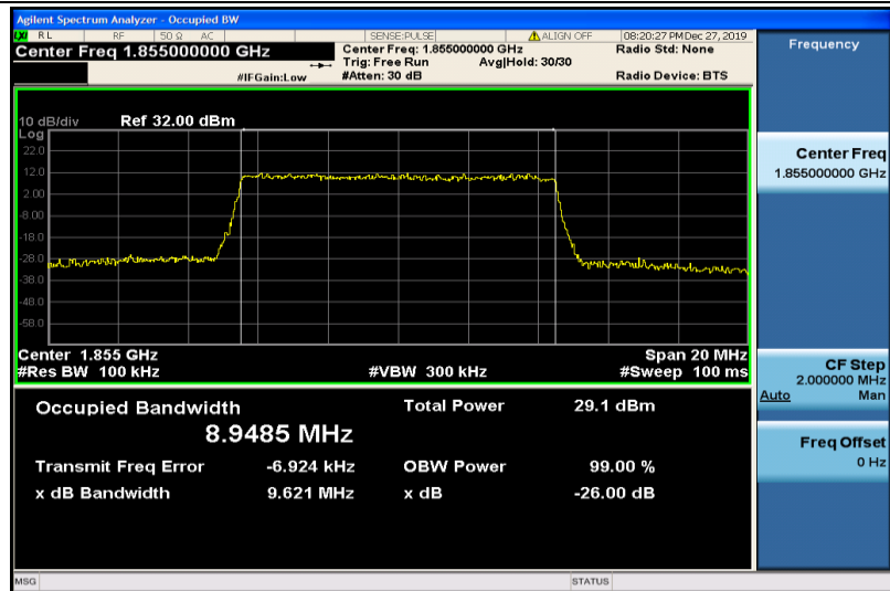
Band2-10MHz-QPSK-18650-50RB#0-8.9485
