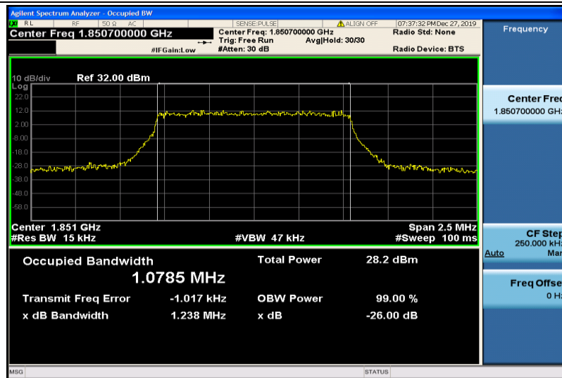
Band2-1.4MHz-QPSK-18607-6RB#0-1.0785
