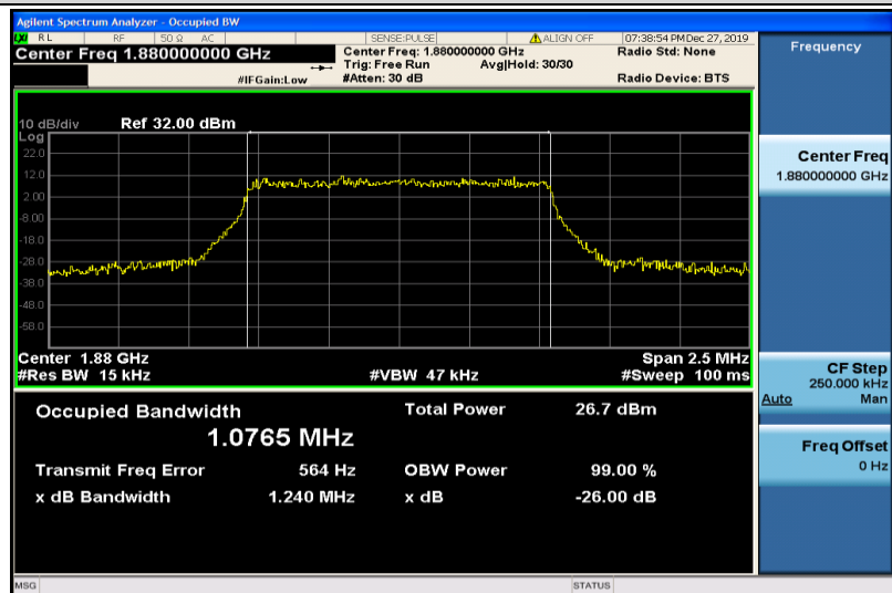
Band2-1.4MHz-16QAM-18900-6RB#0-1.0765
