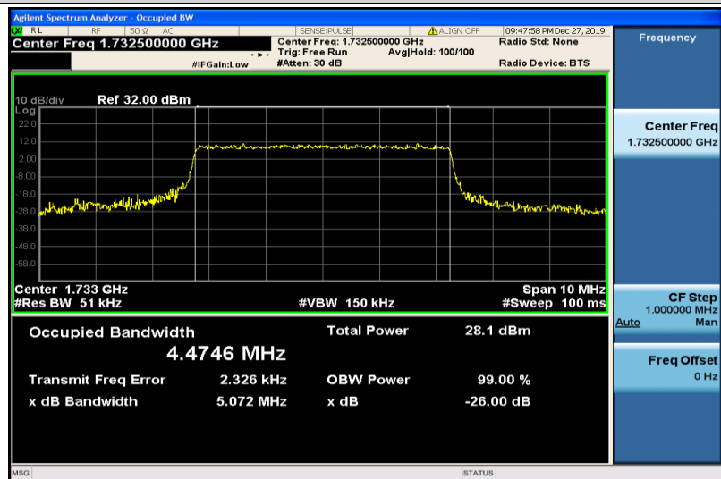
Band4-5MHz-16QAM-20175-25RB#0-4.4746
