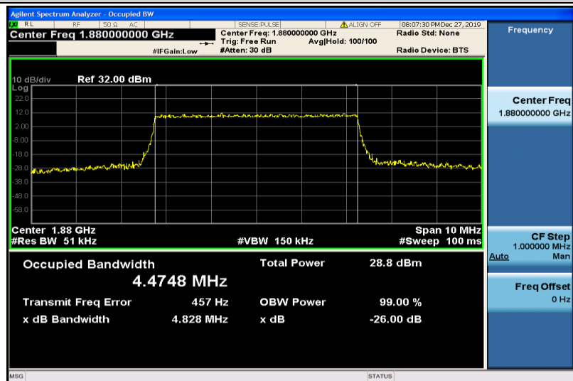
Band2-5MHz-QPSK-18900-25RB#0-4.4748
