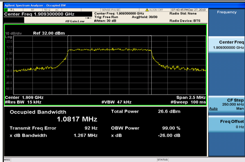
Band2-1.4MHz-16QAM-19193-6RB#0-1.0817
