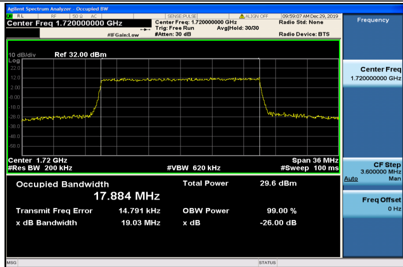
Band4-20MHz-16QAM-20050-100RB#0-17.884
