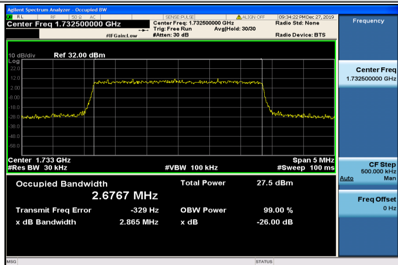
Band4-3MHz-16QAM-20175-15RB#0-2.6767
