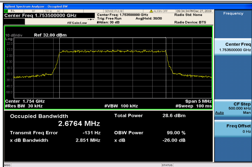
Band4-3MHz-QPSK-20385-15RB#0-2.6764
