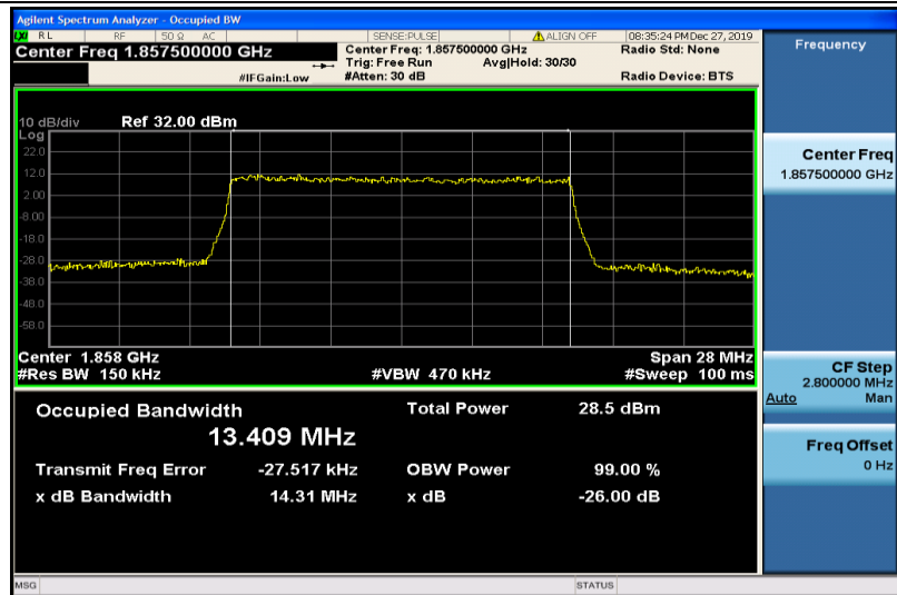
Band2-15MHz-16QAM-18675-75RB#0-13.409
