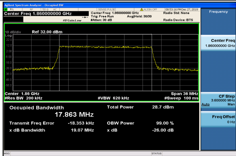
Band2-20MHz-16QAM-18700-100RB#0-17.863
