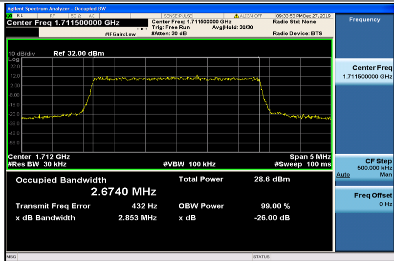
Band4-3MHz-QPSK-19965-15RB#0-2.6740
