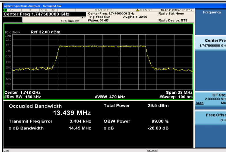
Band4-15MHz-QPSK-20325-75RB#0-13.439
