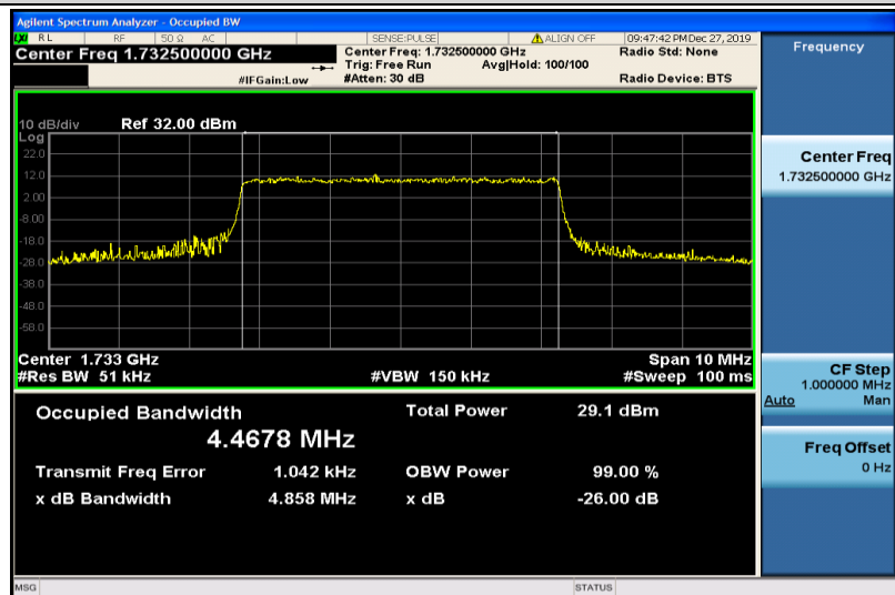
Band4-5MHz-QPSK-17325-25RB#0-4.4678
