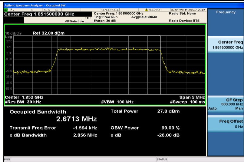
Band2-3MHz-16QAM-18615-15RB#0-2.6713
