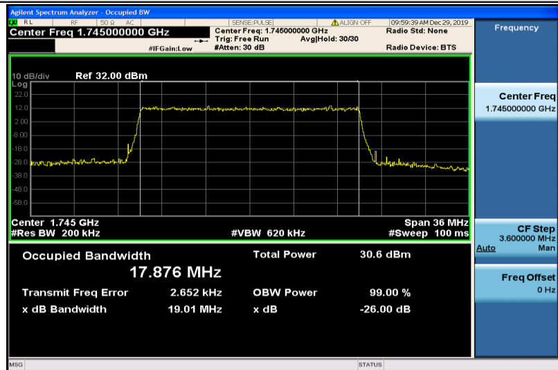
Band4-20MHz-QPSK-20300-100RB#0-17.876
