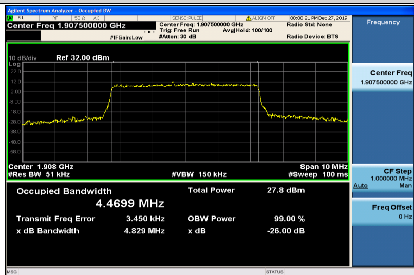
Band2-5MHz-16QAM-19175-25RB#0-4.4699
