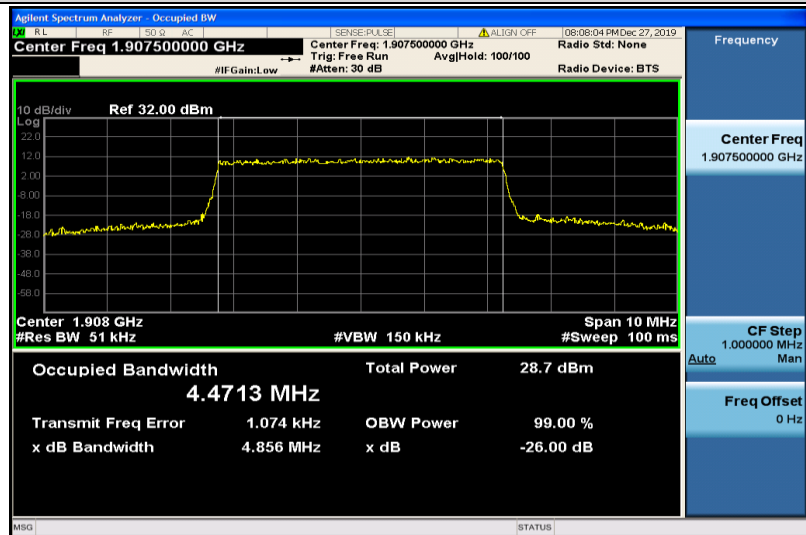
Band2-5MHz-QPSK-19175-25RB#0-4.4713
