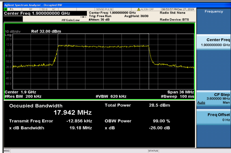
Band2-20MHz-16QAM-19100-100RB#0-17.942
