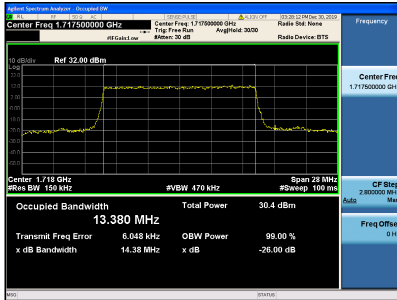
Band4-15MHz-QPSK-20025-75RB#0-13.380
