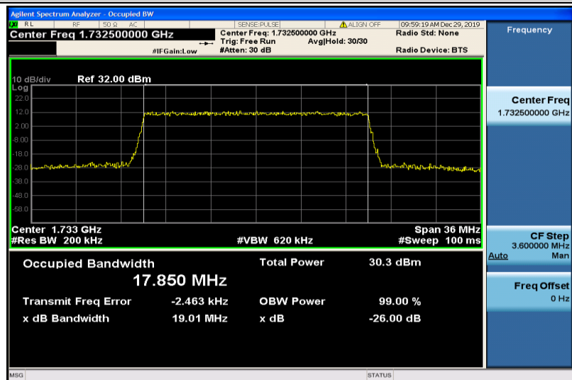
Band4-20MHz-QPSK-20175-100RB#0-17.850
