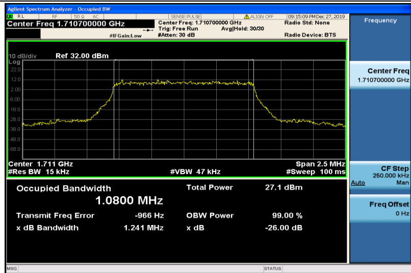
Band4-1.4MHz-16QAM-19957-6RB#0-1.0800
