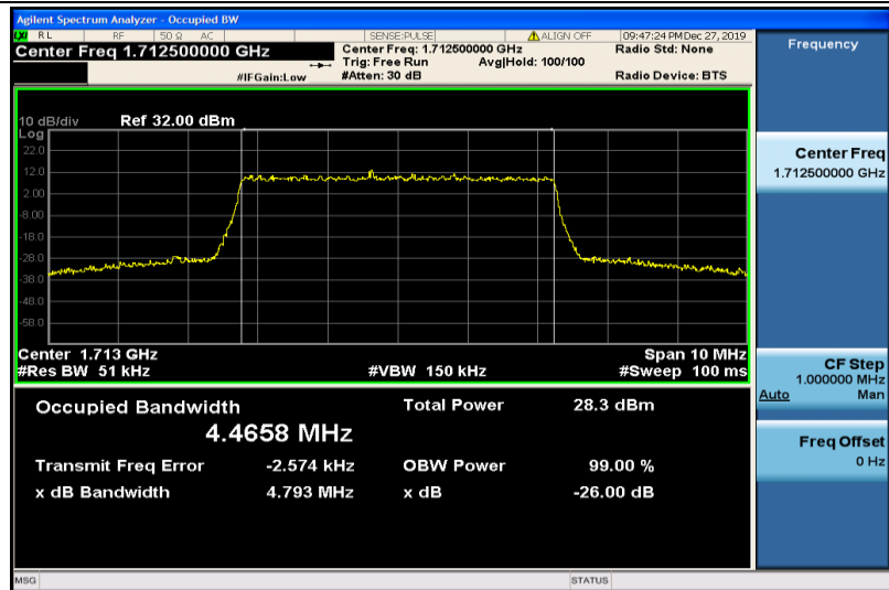
Band4-5MHz-16QAM-19975-25RB#0-4.4658
