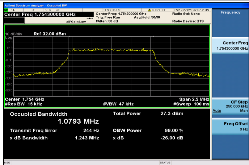
Band4-1.4MHz-16QAM-20393-6RB#0-1.0793
