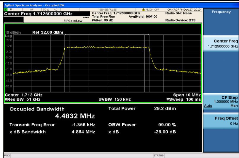
Band4-5MHz-QPSK-19975-25RB#0-4.4832
