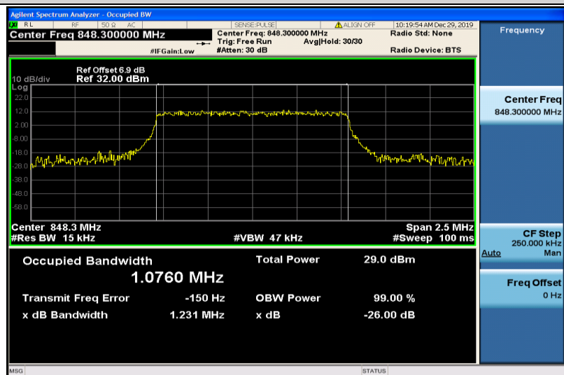
Band5-1.4MHz-QPSK-20643-6RB#0-1.0760
