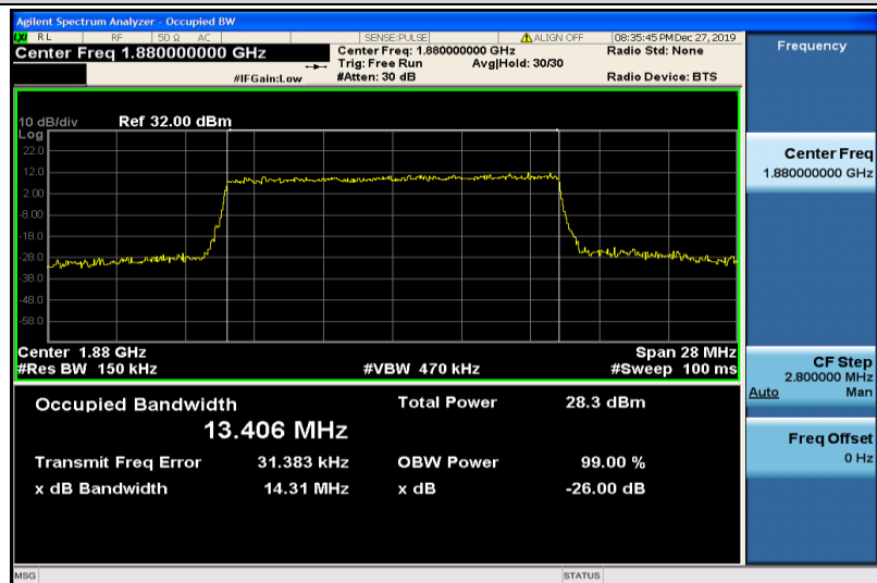
Band2-15MHz-16QAM-18900-75RB#0-13.406
