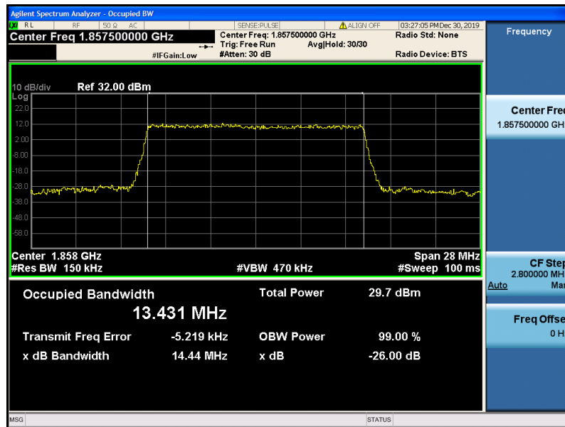
Band2-15MHz-QPSK-18675-75RB#0-13.431
