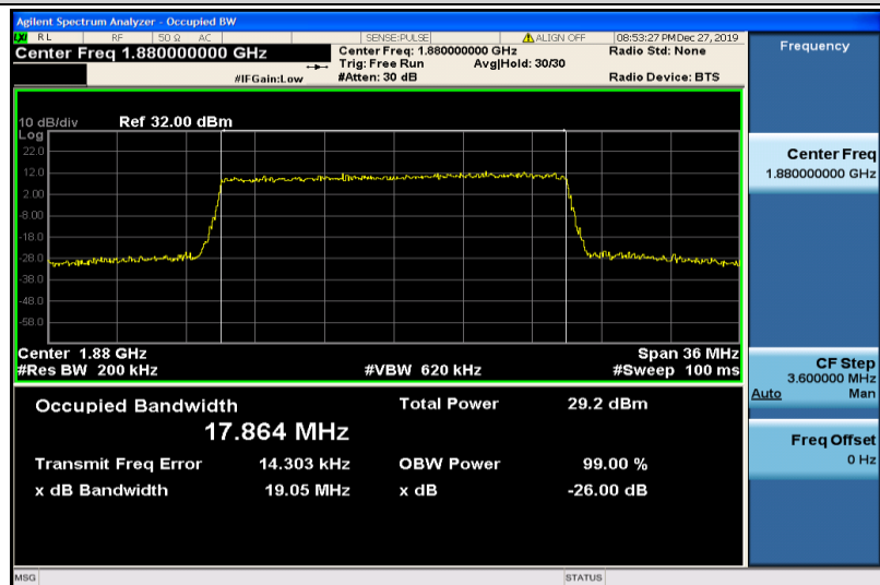
Band2-20MHz-QPSK-18900-100RB#0-17.864
