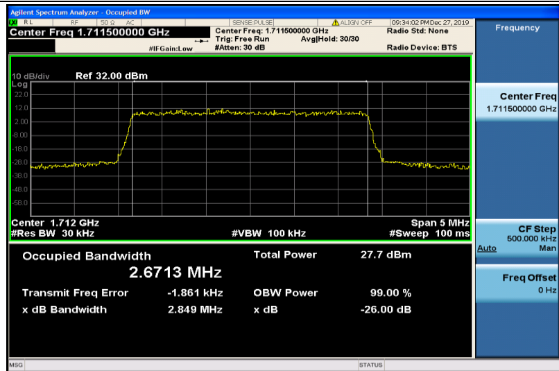
Band4-3MHz-16QAM-19965-15RB#0-2.6713
