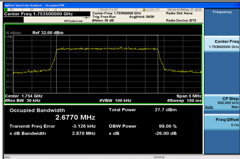
Band4-3MHz-16QAM-20385-15RB#0-2.6770
