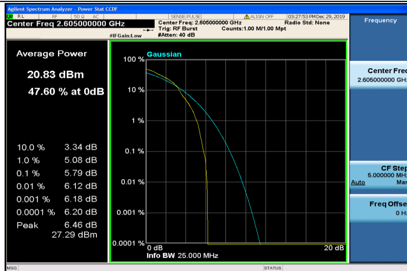
Band41-20MHz-16QAM-40740-1RB#0
