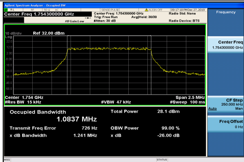
Band4-1.4MHz-QPSK-20393-6RB#0-1.0837
