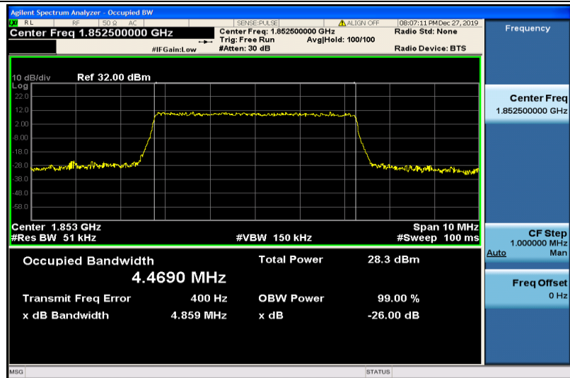
Band2-5MHz-16QAM-18625-25RB#0-4.4690
