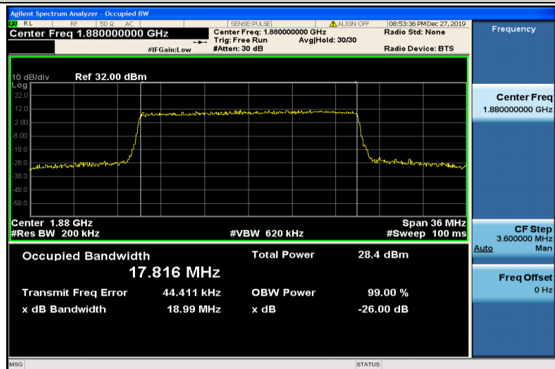
Band2-20MHz-16QAM-18900-100RB#0-17.816
