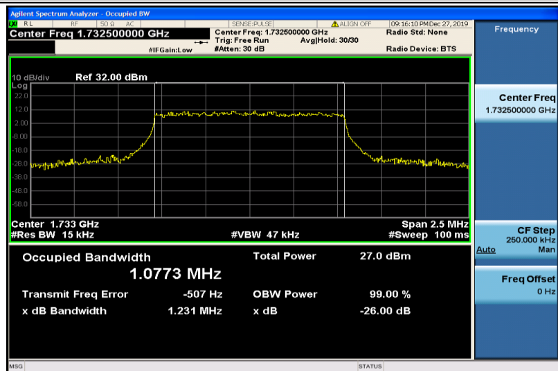
Band4-1.4MHz-16QAM-20175-6RB#0-1.0773
