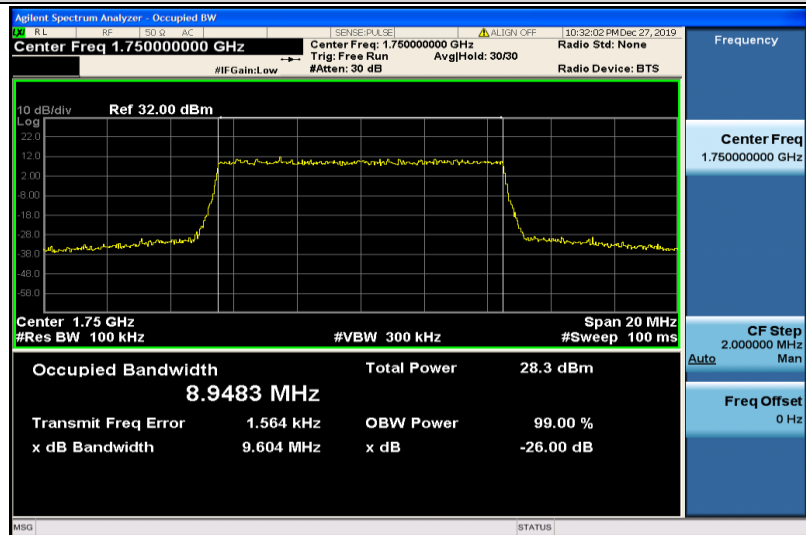
Band4-10MHz-16QAM-20350-50RB#0-8.9483
