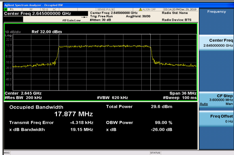
Band41-20MHz-16QAM-41140-100RB#0-17.877
