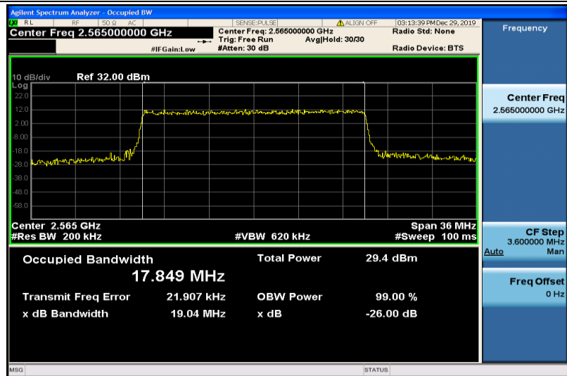
Band41-20MHz-16QAM-40340-100RB#0-17.849
