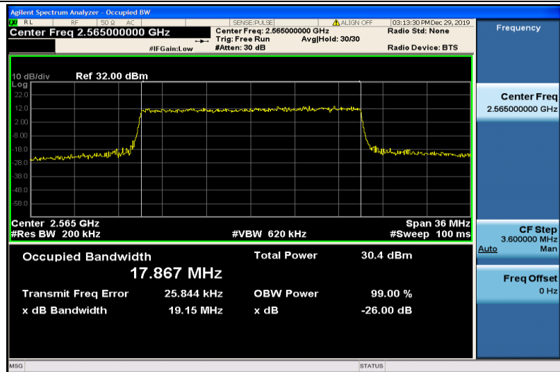
Band41-20MHz-QPSK-40340-100RB#0-17.867
