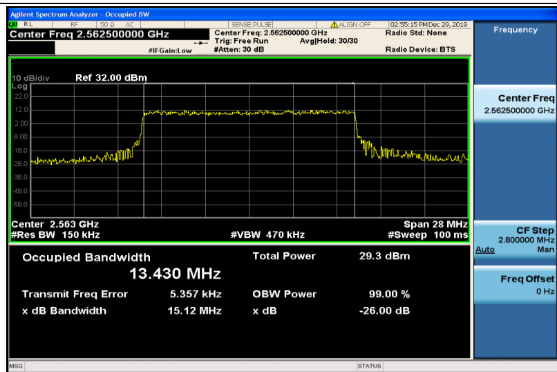
Band41-15MHz-16QAM-40315-75RB#0-13.430
