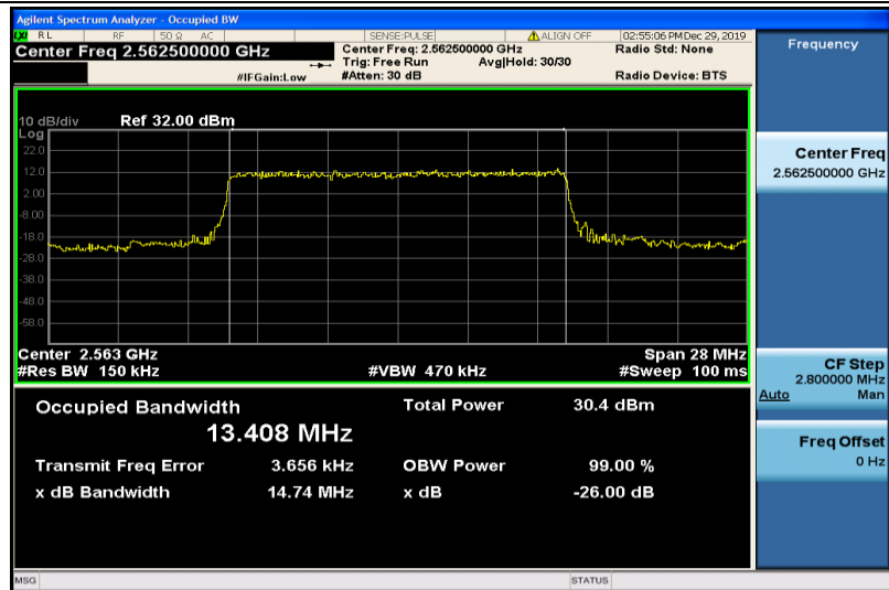
Band41-15MHz-QPSK-40315-75RB#0-13.408
