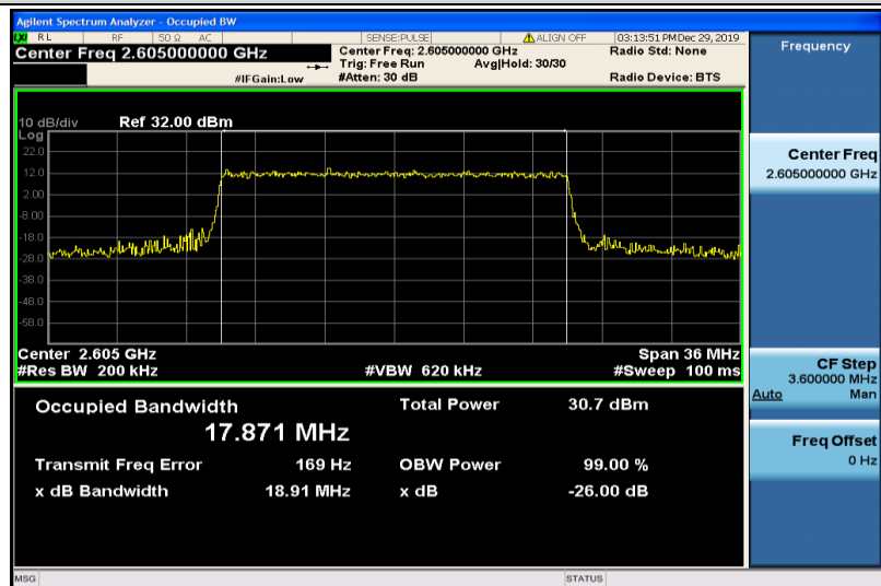
Band41-20MHz-QPSK-40740-100RB#0-17.871
