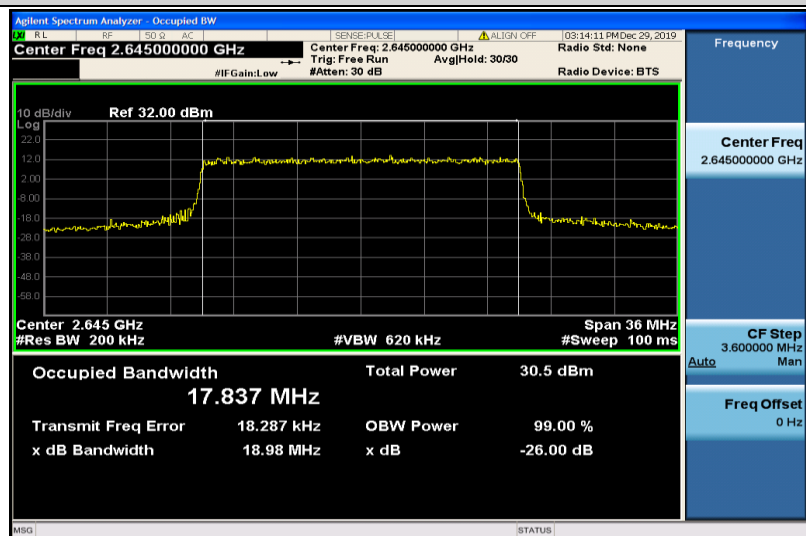
Band41-20MHz-QPSK-41140-100RB#0-17.837
