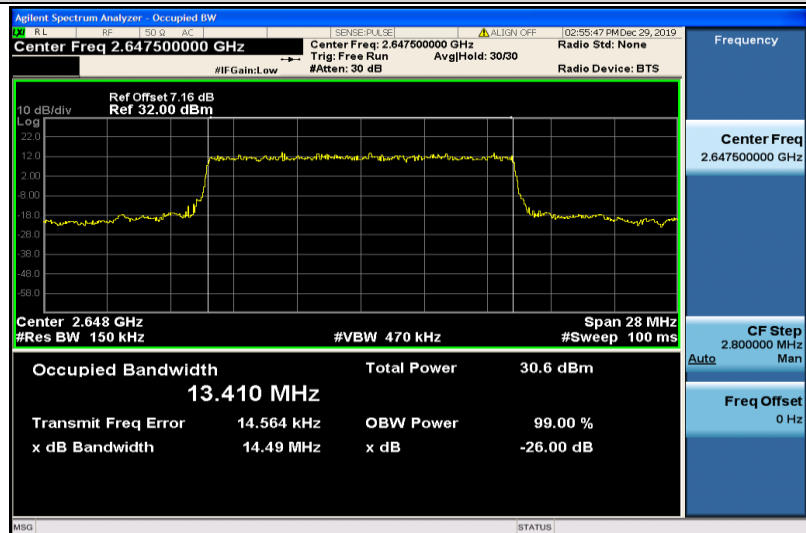
Band41-15MHz-QPSK-41165-75RB#0-13.410
