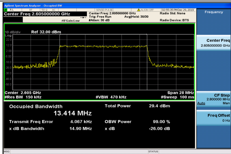
Band41-15MHz-16QAM-40740-75RB#0-13.414
