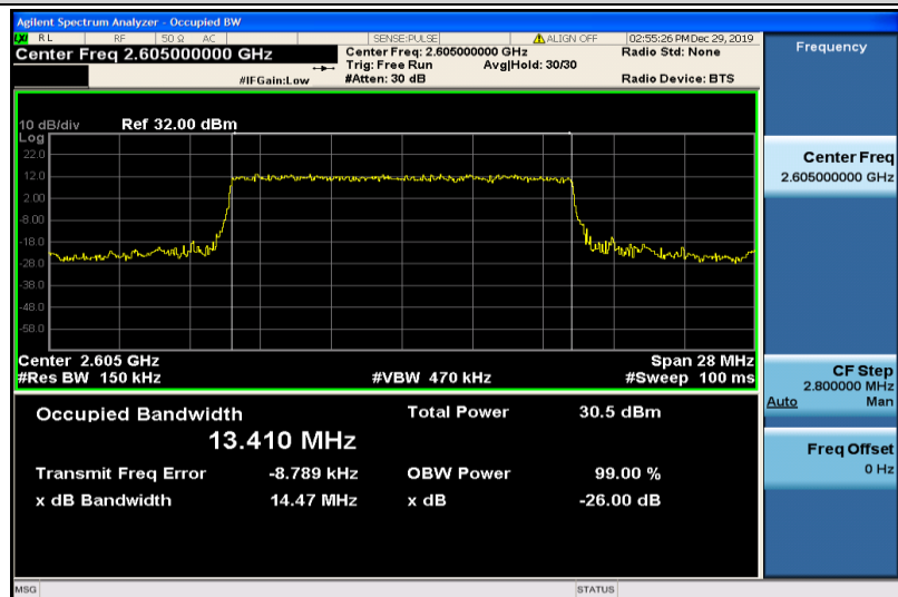
Band41-15MHz-QPSK-40740-75RB#0-13.410
