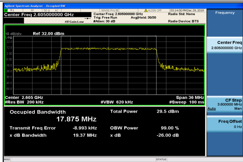
Band41-20MHz-16QAM-40740-100RB#0-17.875
