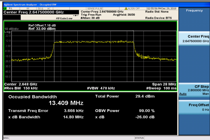
Band41-15MHz-16QAM-41165-75RB#0-13.409
