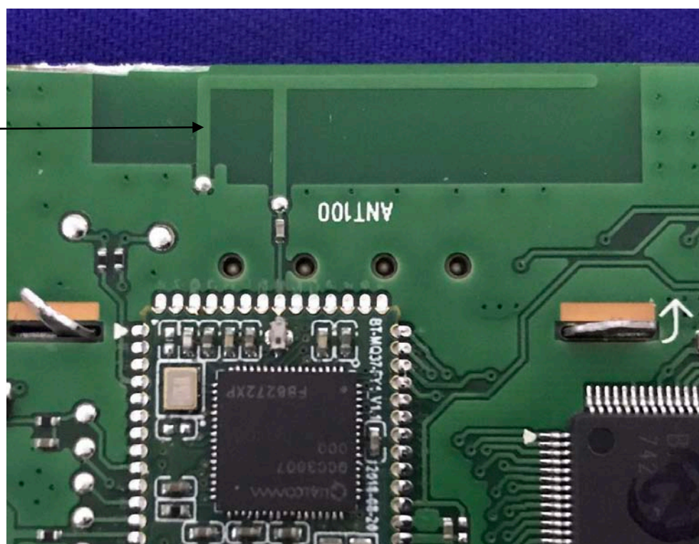
Bluetooth Antenna
