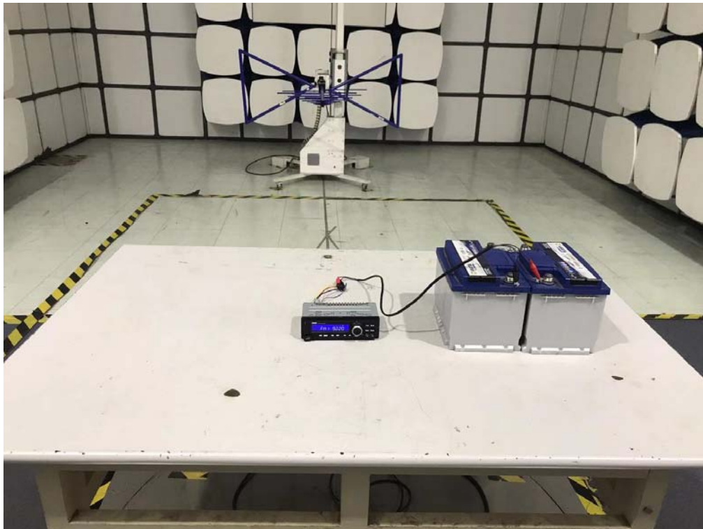
Radiated test:30-1000MHz
