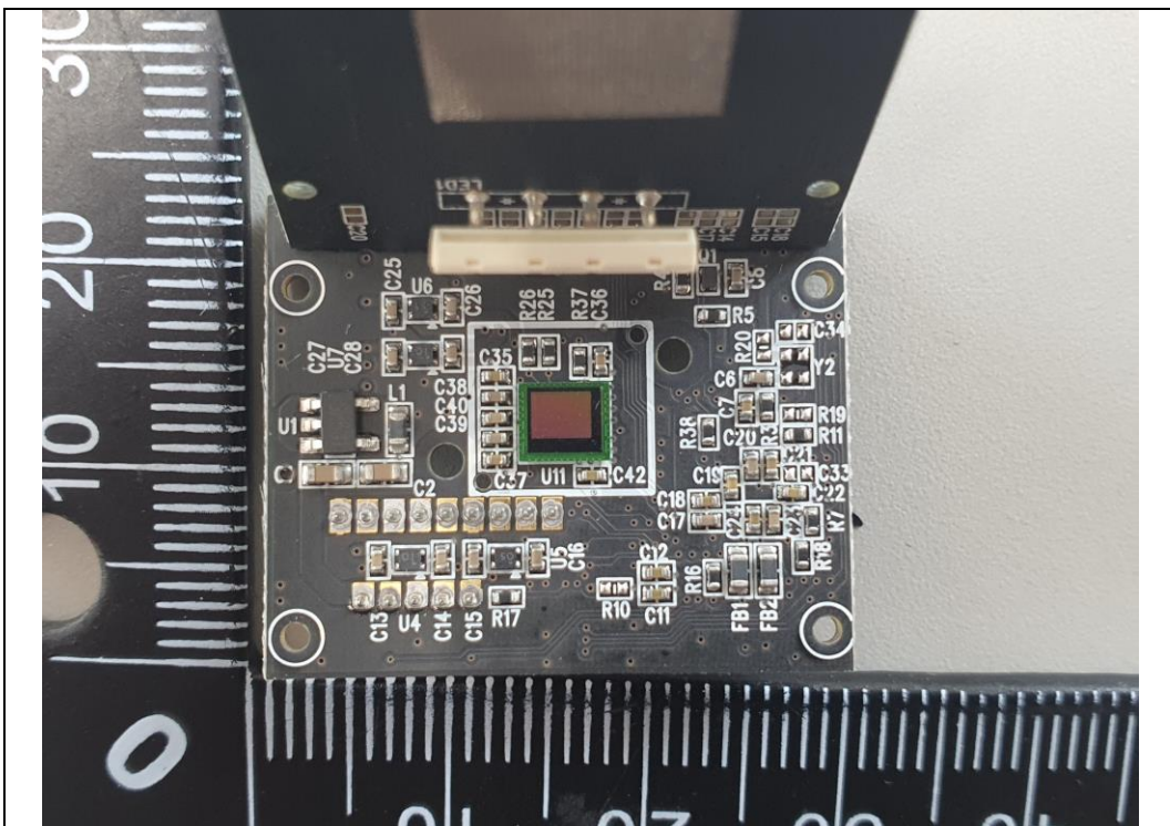
Sensor Board Rear
