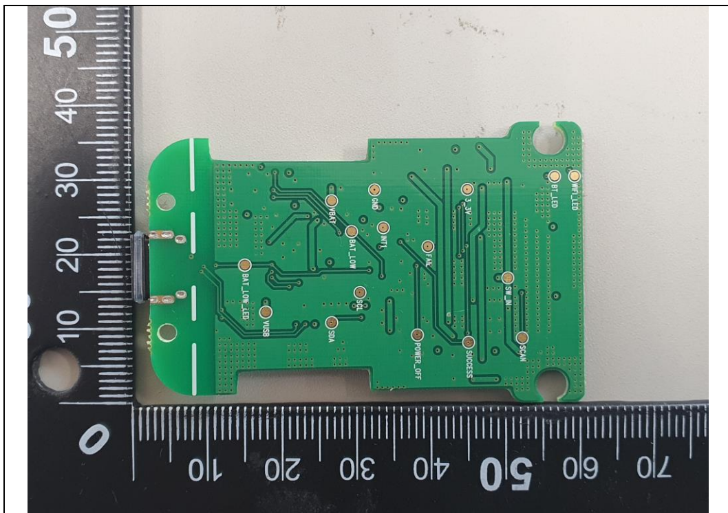
IO Board Rear
