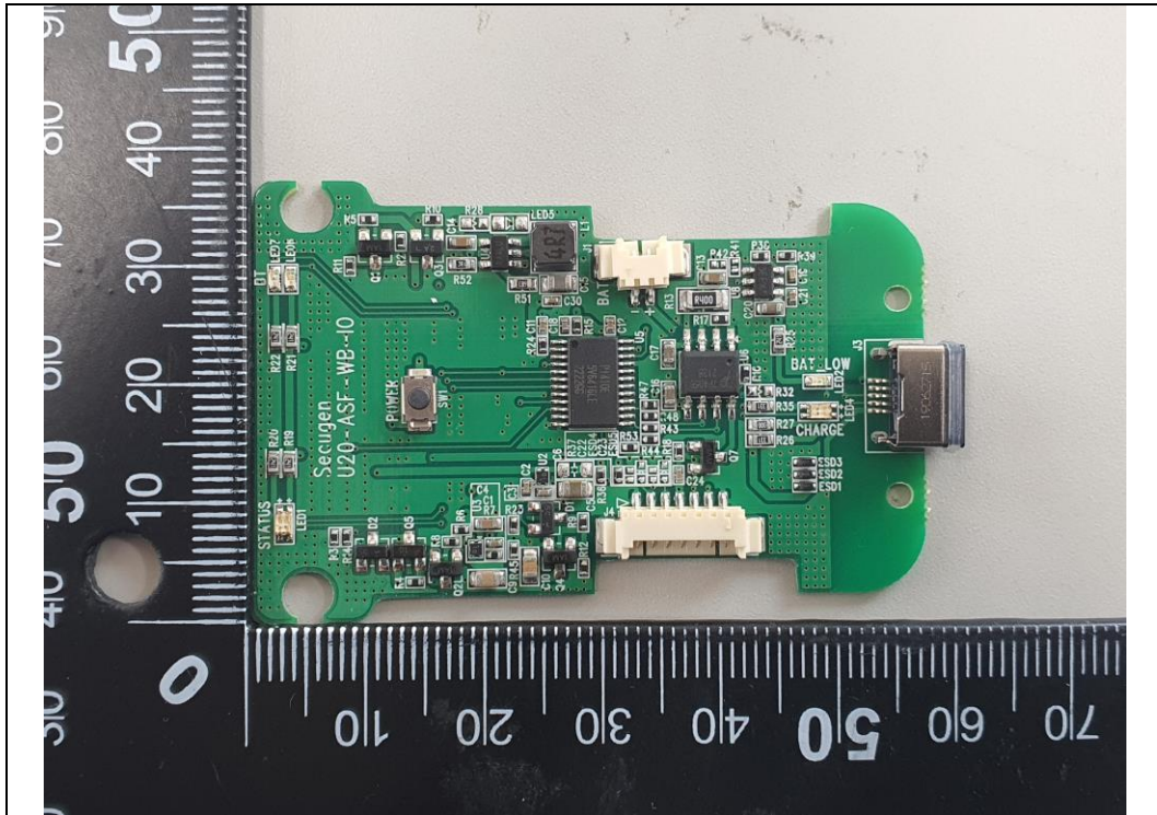
IO Board Front
