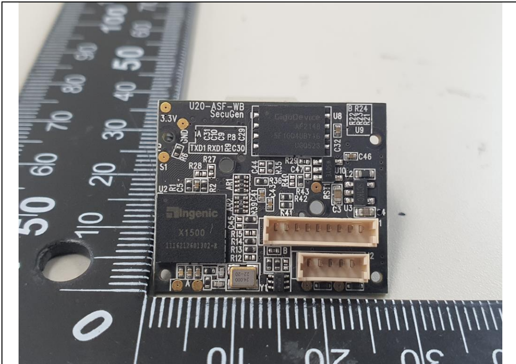
Sensor Board Front
