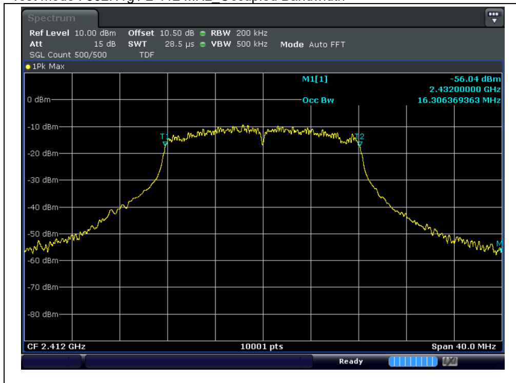
Test mode : 802.11g / 2 412 MHz_Occupied Bandwidth
