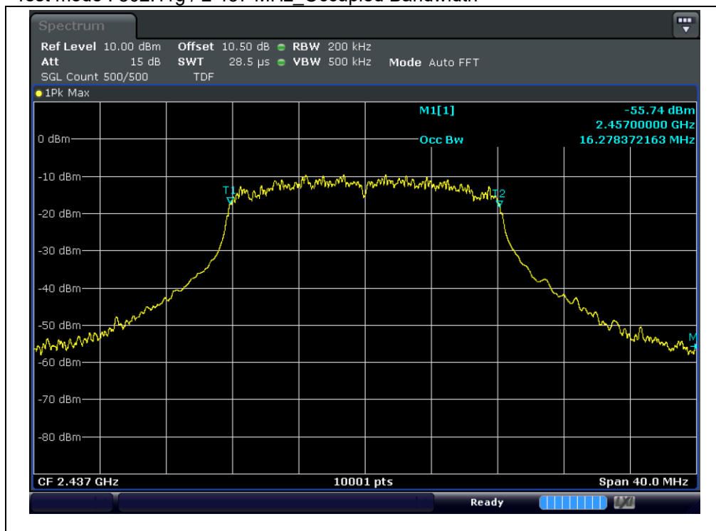
Test mode : 802.11g / 2 437 MHz_Occupied Bandwidth
