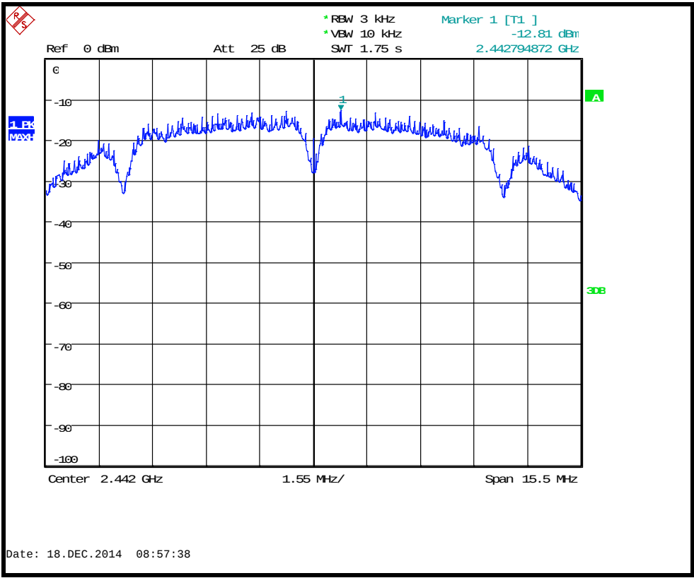
Conducted power spectral density 2442MHz 1Mb/s
