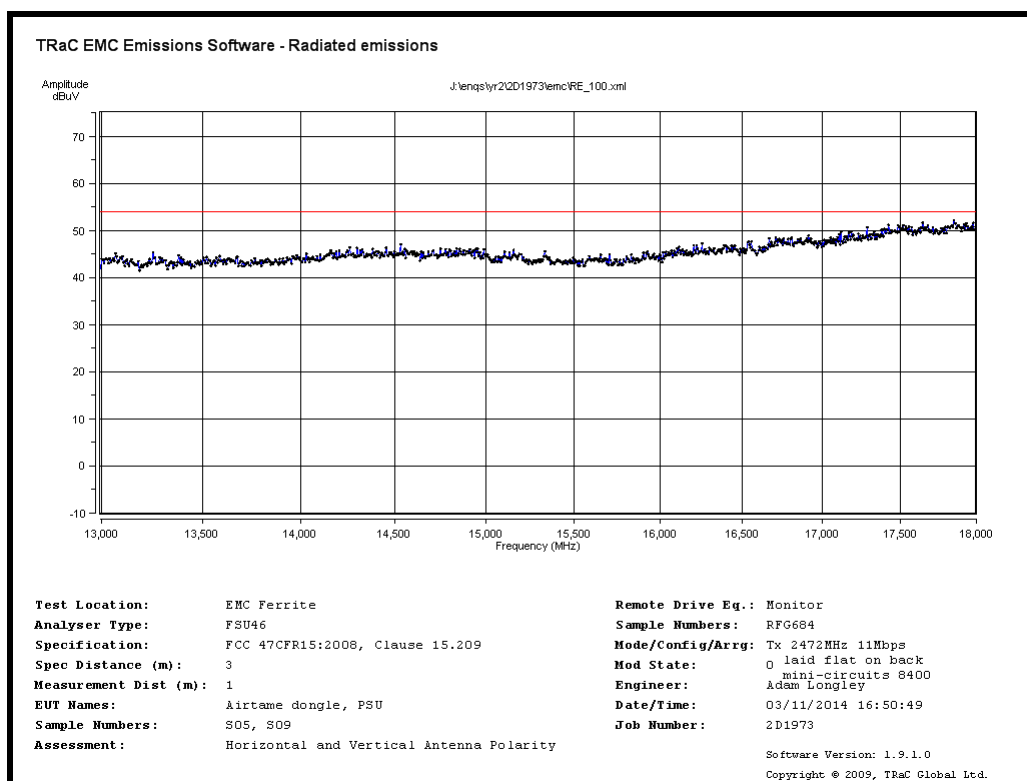
Radiated Spurious emissions 13GHz to 18GHz – 2472MHz 11Mb/s
