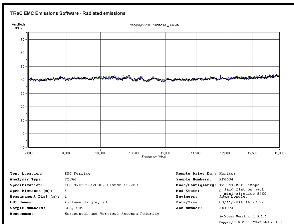
Radiated Spurious emissions 9GHz to 13GHz – 2442MHz 54Mb/s
