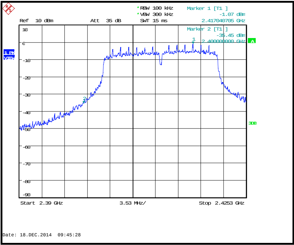
Conducted Lower Band Edge 2412MHz MCS0
