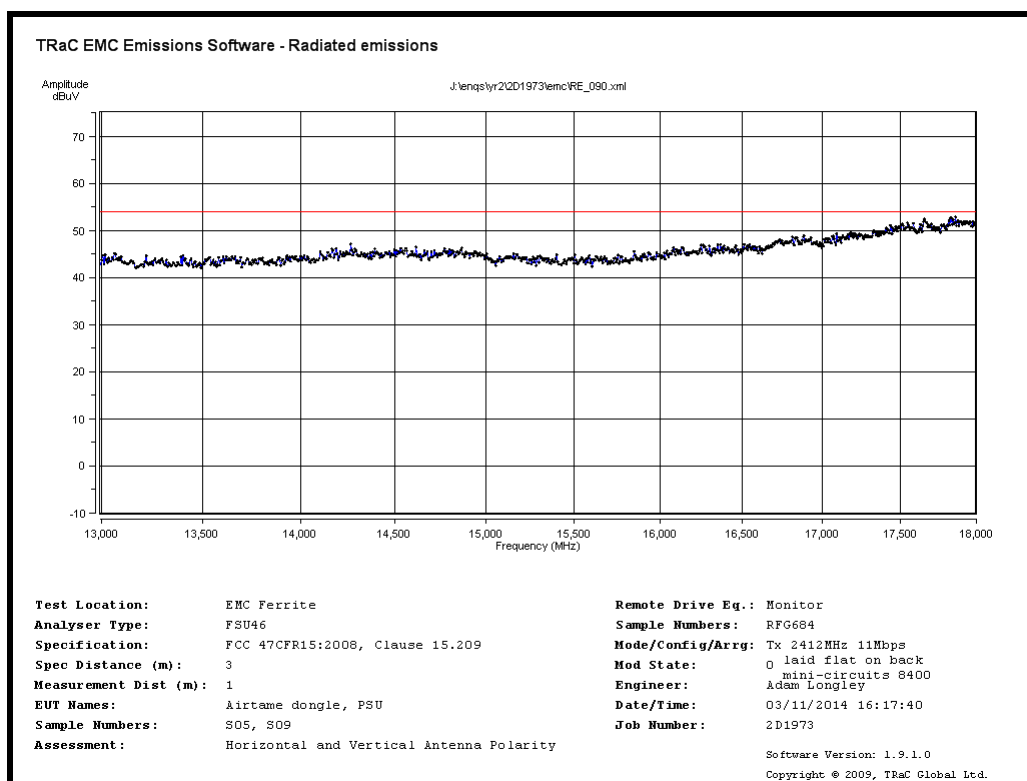
Radiated Spurious emissions 13GHz to 18GHz – 2412MHz 11Mb/s
