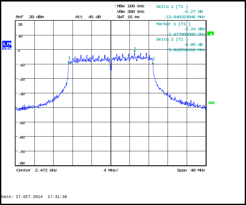
6dB Bandwidth 2472MHz MCS6
