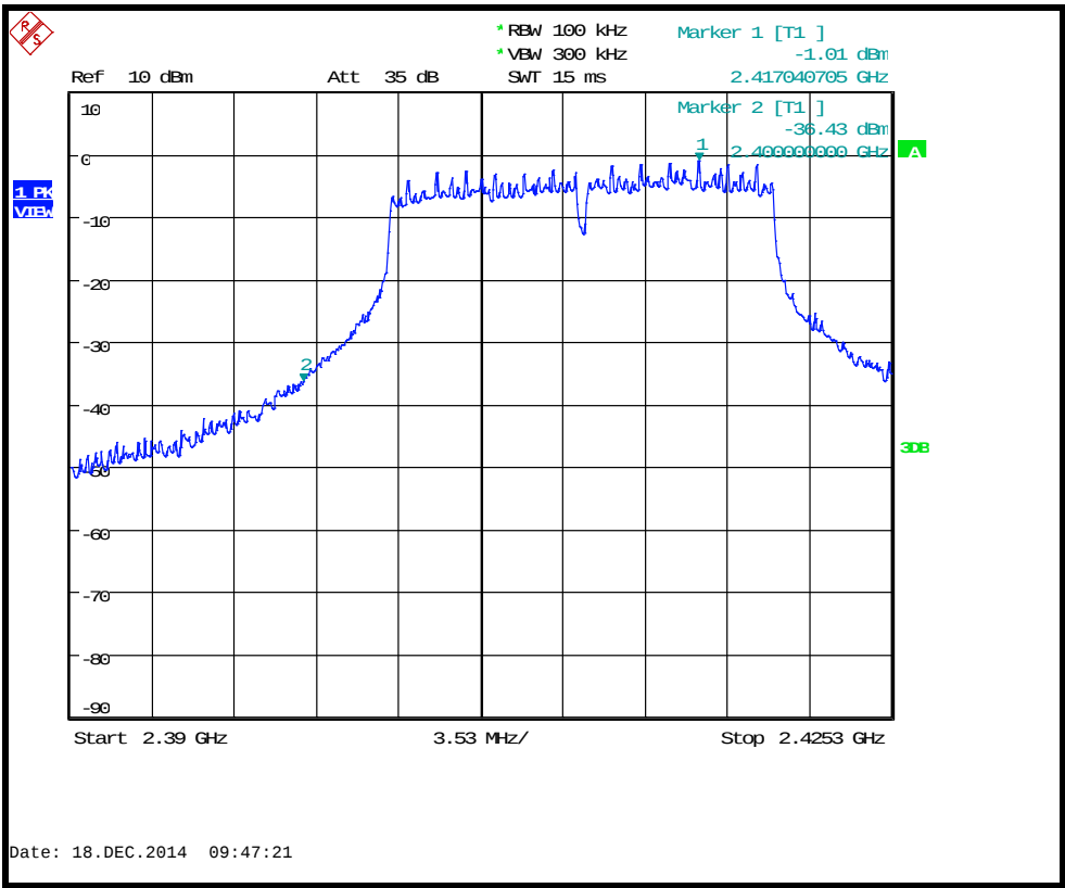
Conducted Lower Band Edge 2412MHz 54Mb/s
