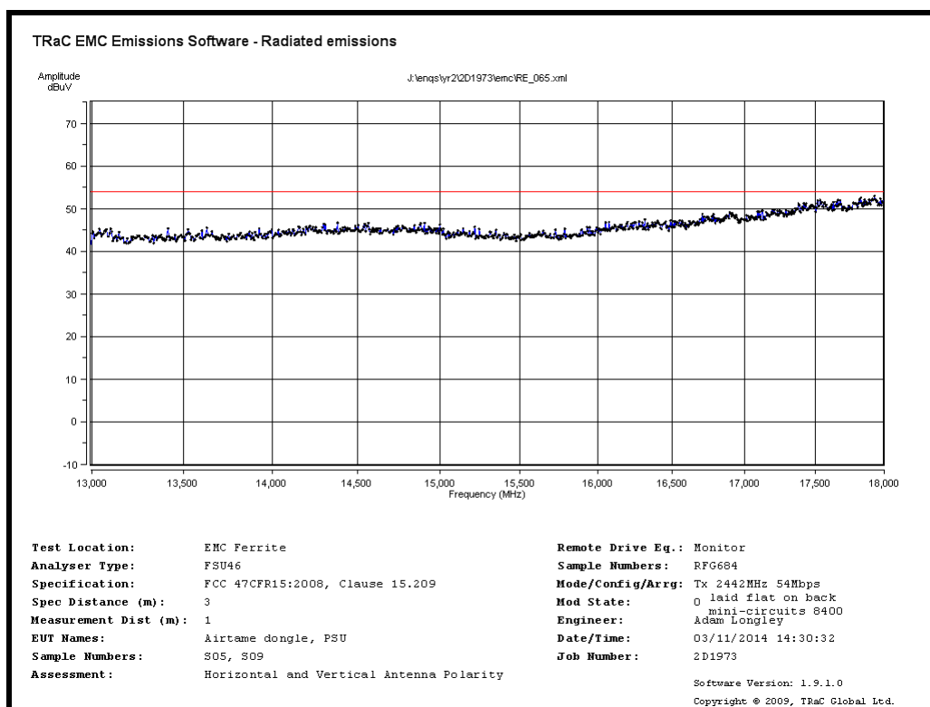
Radiated Spurious emissions 13GHz to 18GHz – 2442MHz 54Mb/s
