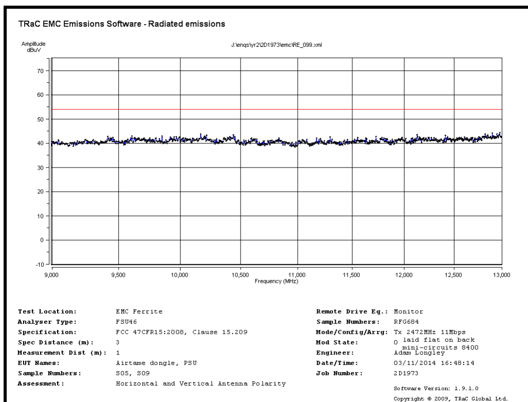
Radiated Spurious emissions 9GHz to 13GHz – 2472MHz 11Mb/s
