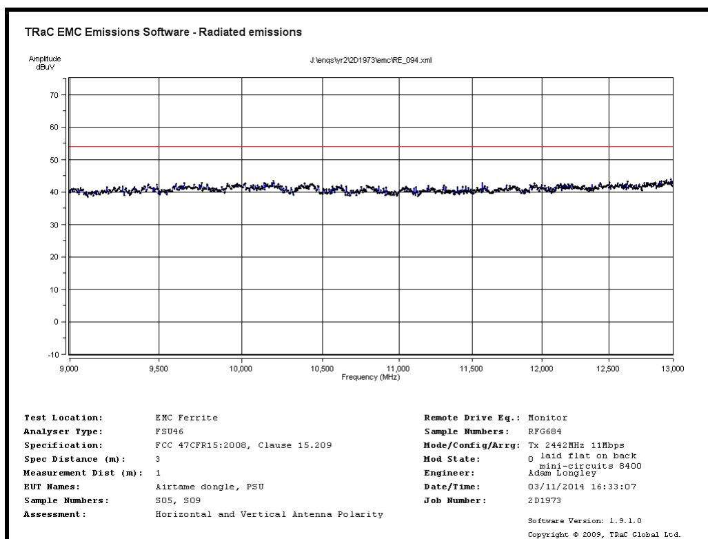
Radiated Spurious emissions 9GHz to 13GHz – 2442MHz 11Mb/s
