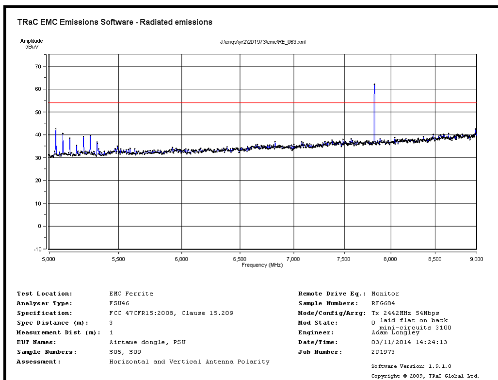
Radiated Spurious emissions 5GHz to 9GHz – 2442MHz 54Mb/s
