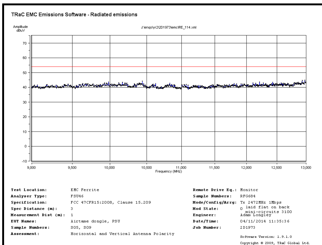
Radiated Spurious emissions 9GHz to 13GHz – 2472MHz 1Mb/s
