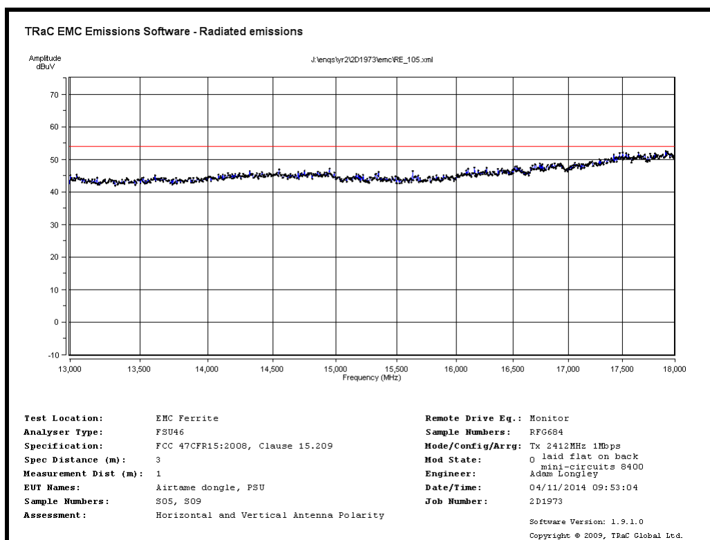
Radiated Spurious emissions 13GHz to 18GHz – 2412MHz 1Mb/s
