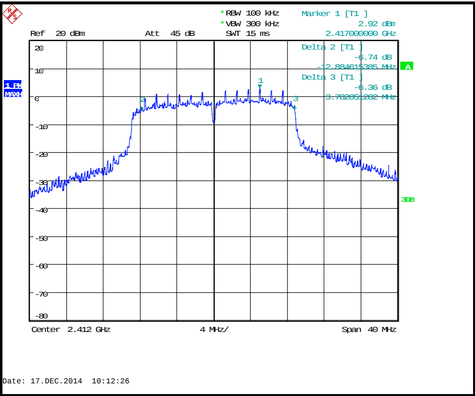
6dB Bandwidth 2412MHz MCS0
