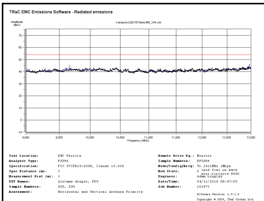
Radiated Spurious emissions 9GHz to 13GHz – 2412MHz 1Mb/s
