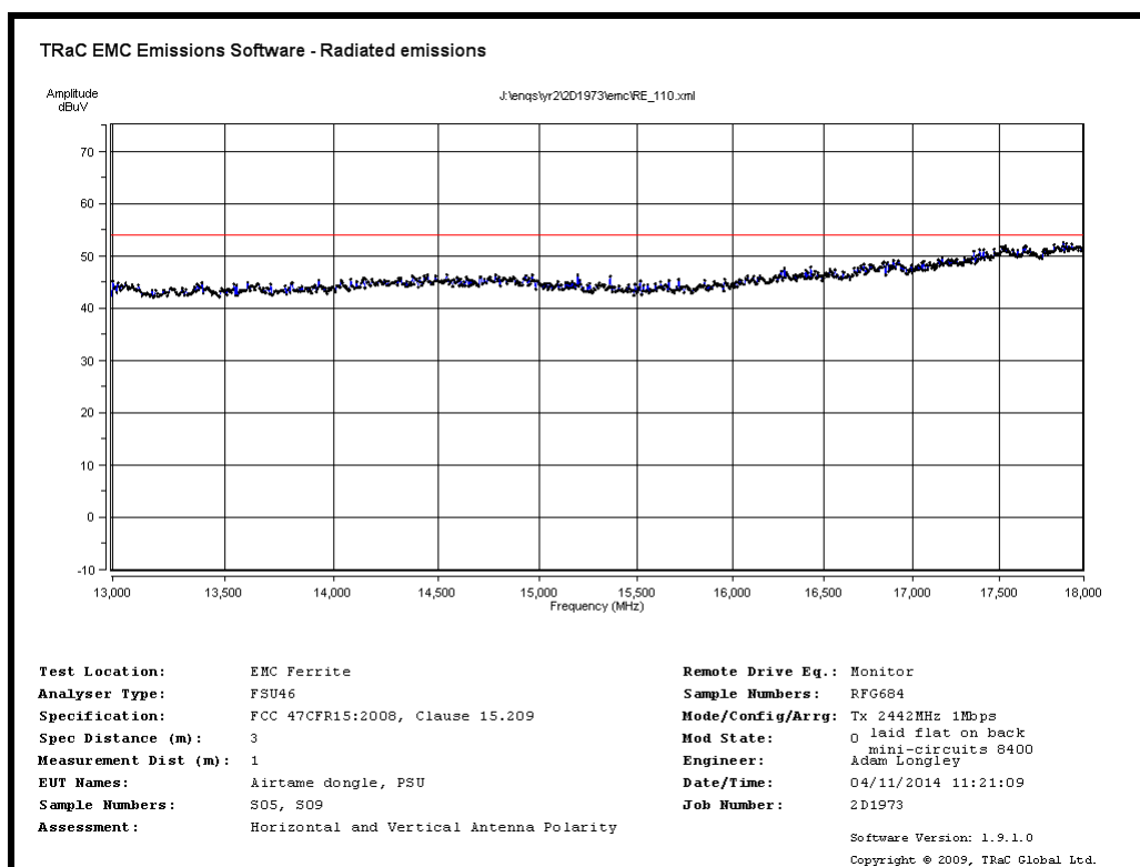
Radiated Spurious emissions 13GHz to 18GHz – 2442MHz 1Mb/s
