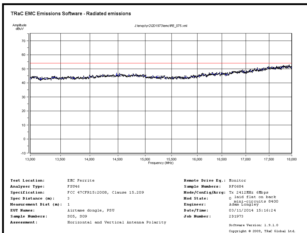
Radiated Spurious emissions 13GHz to 18GHz – 2412MHz 6Mb/s
