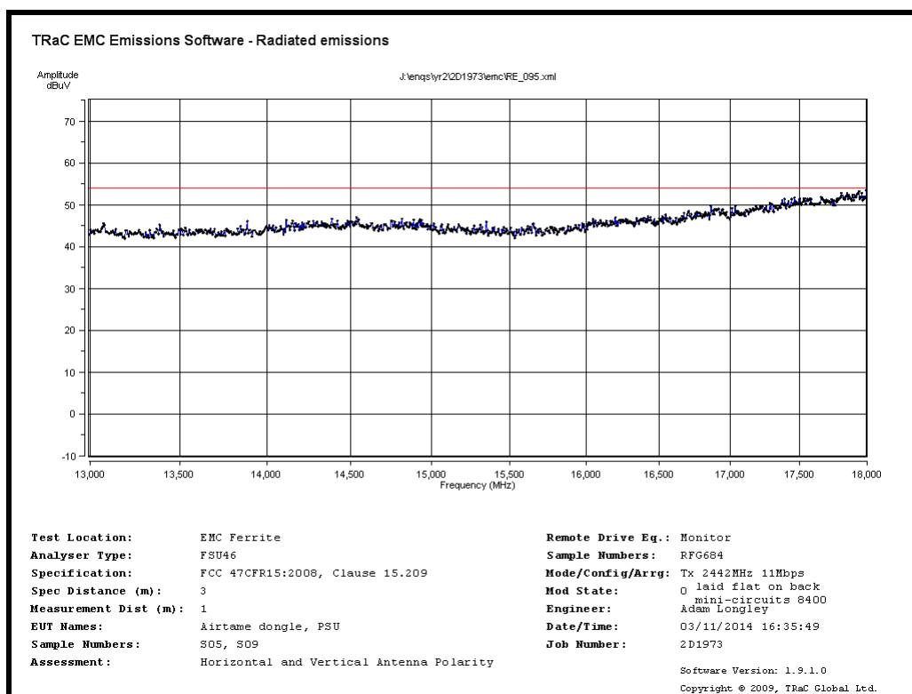
Radiated Spurious emissions 13GHz to 18GHz – 2442MHz 11Mb/s
