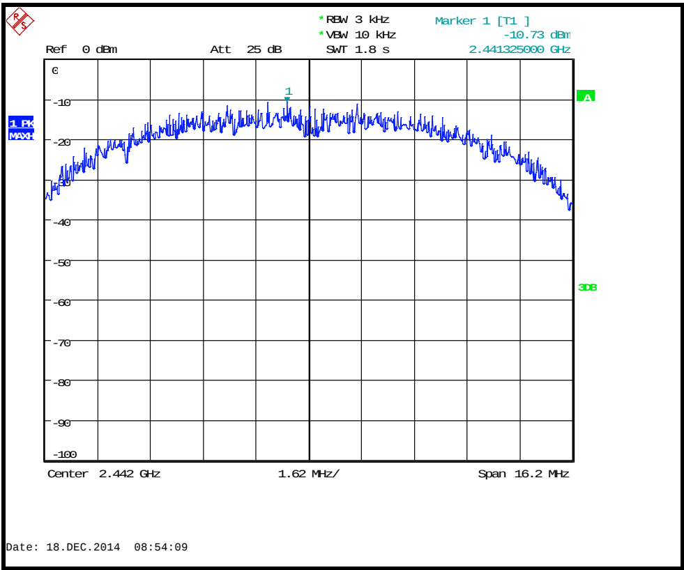
Conducted power spectral density 2442MHz 11Mb/s
