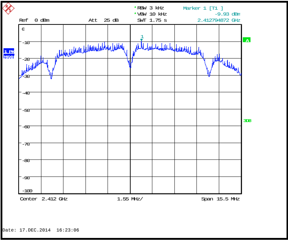
Conducted power spectral density 2412MHz 1Mb/s
