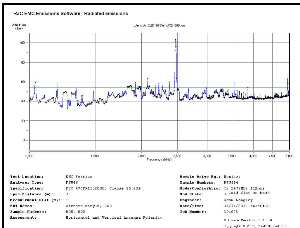
Radiated Spurious emissions 1GHz to 5GHz – 2472MHz 11Mb/s
