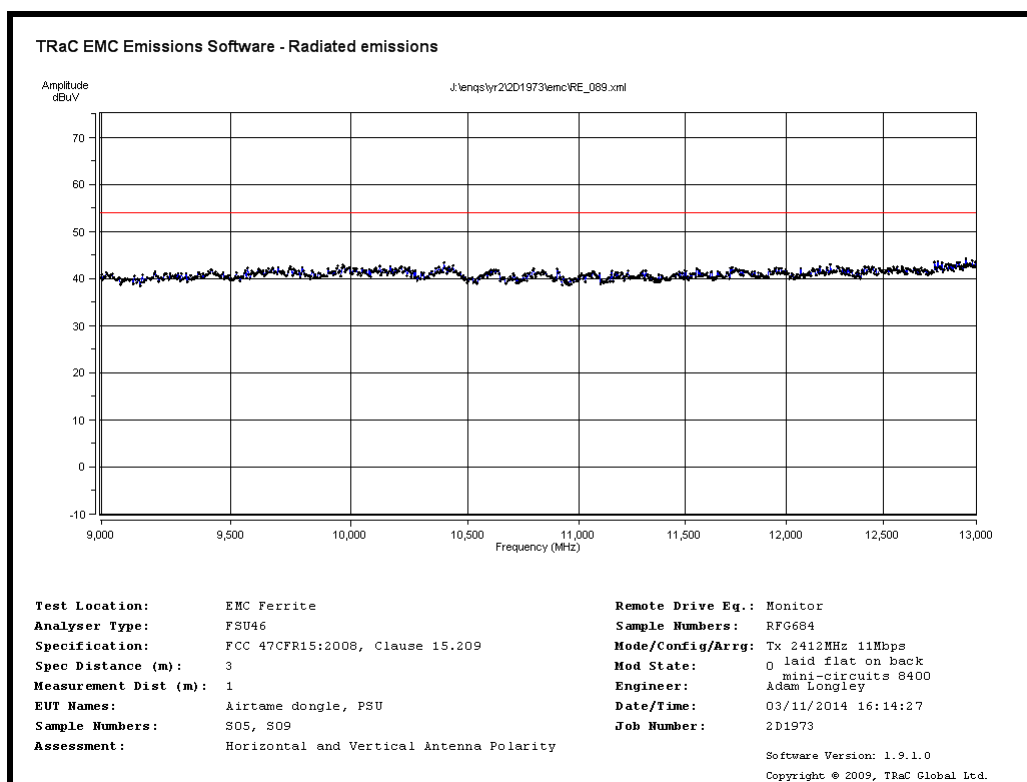
Radiated Spurious emissions 9GHz to 13GHz – 2412MHz 11Mb/s
