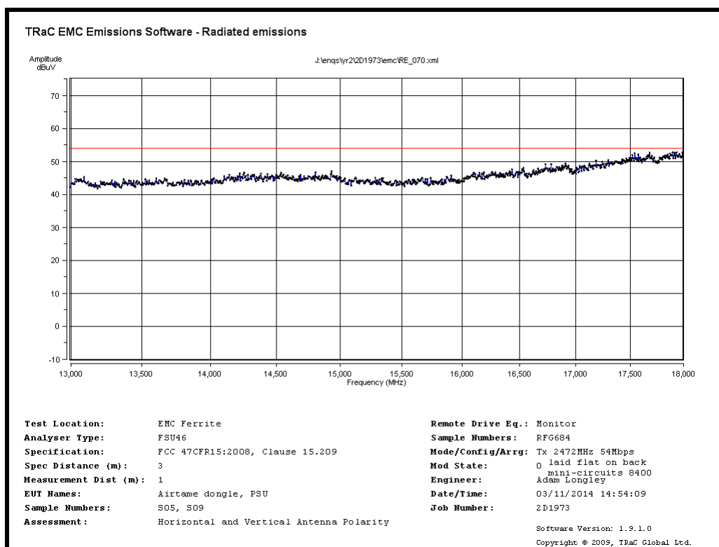
Radiated Spurious emissions 13GHz to 18GHz – 2472MHz 54Mb/s
