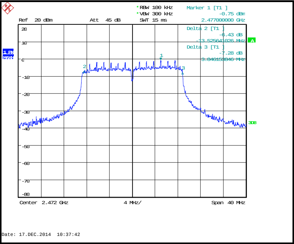
6dB Bandwidth 2472MHz MCS0
