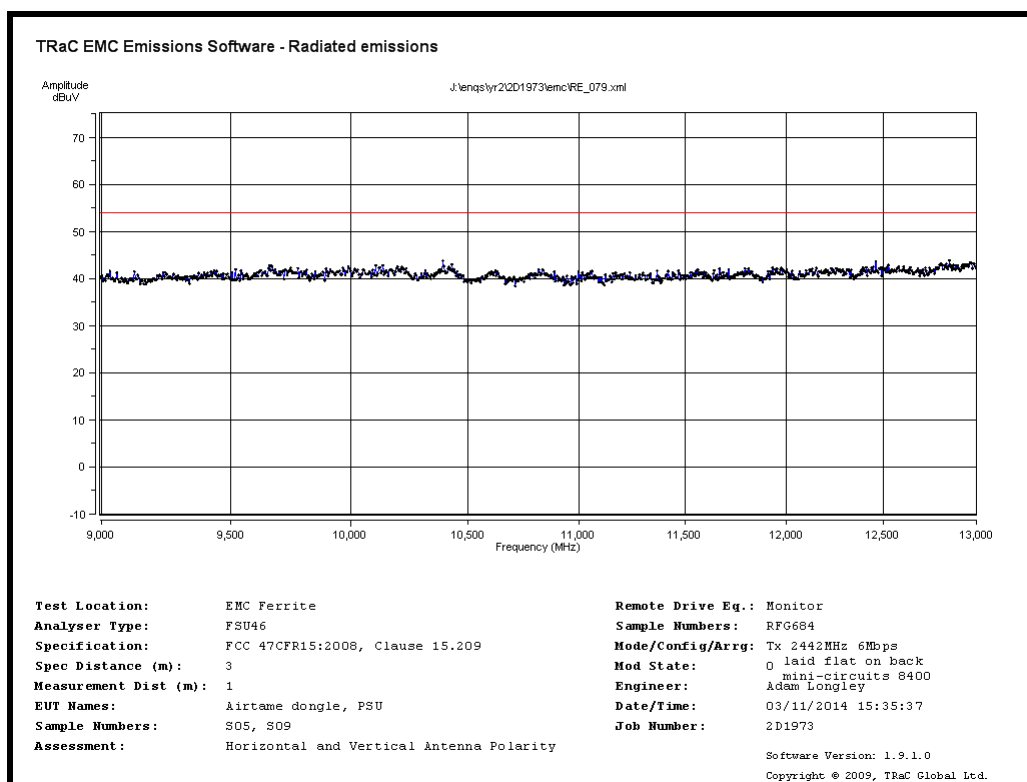
Radiated Spurious emissions 9GHz to 13GHz – 2442MHz 6Mb/s
