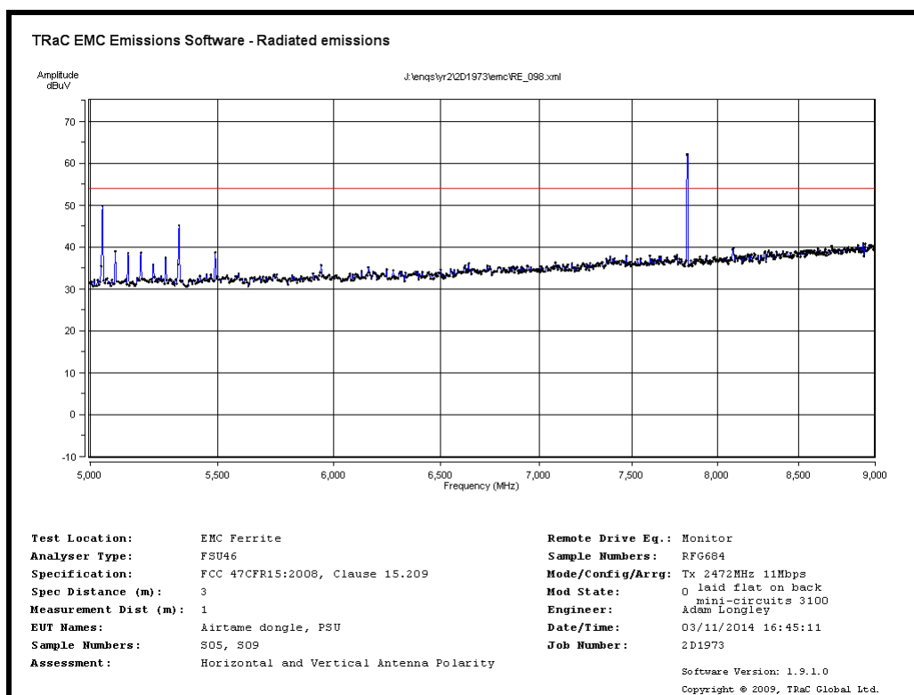
Radiated Spurious emissions 5GHz to 9GHz – 2472MHz 11Mb/s
