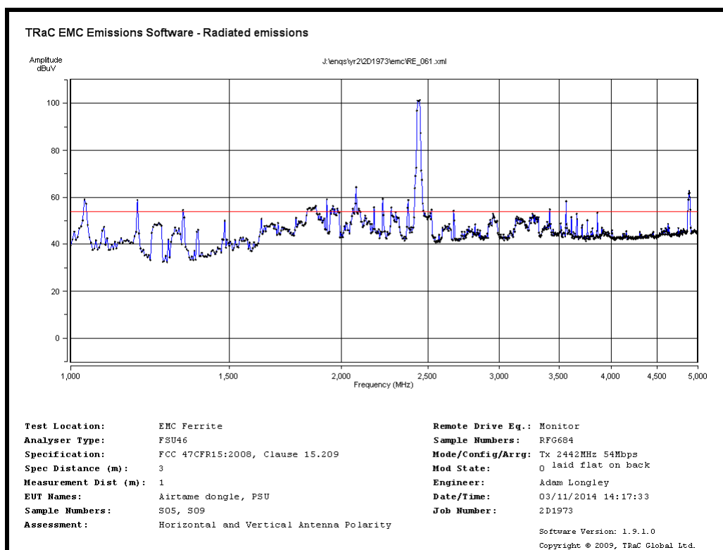
Radiated Spurious emissions 1GHz to 5GHz – 2442MHz 54Mb/s
