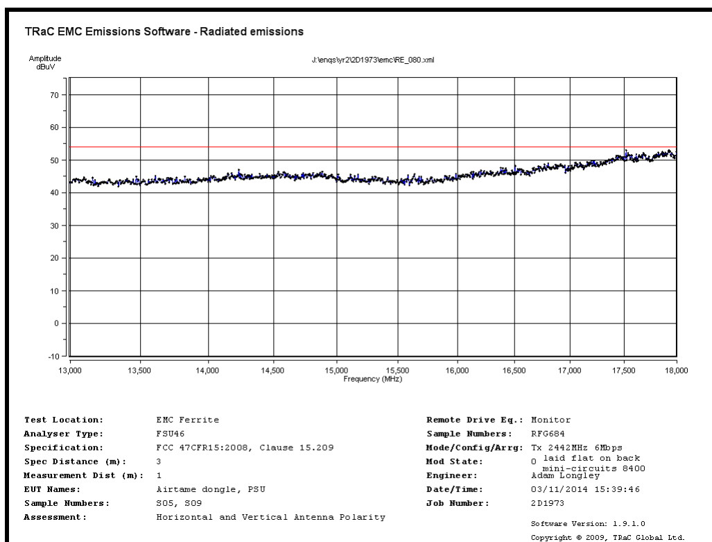
Radiated Spurious emissions 13GHz to 18GHz – 2442MHz 6Mb/s
