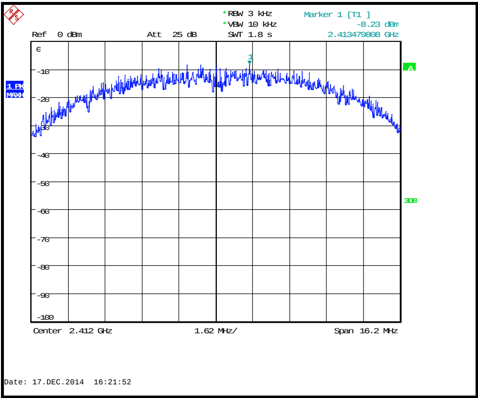
Conducted power spectral density 2412MHz 11Mb/s
