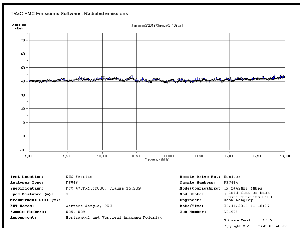
Radiated Spurious emissions 9GHz to 13GHz – 2442MHz 1Mb/s
