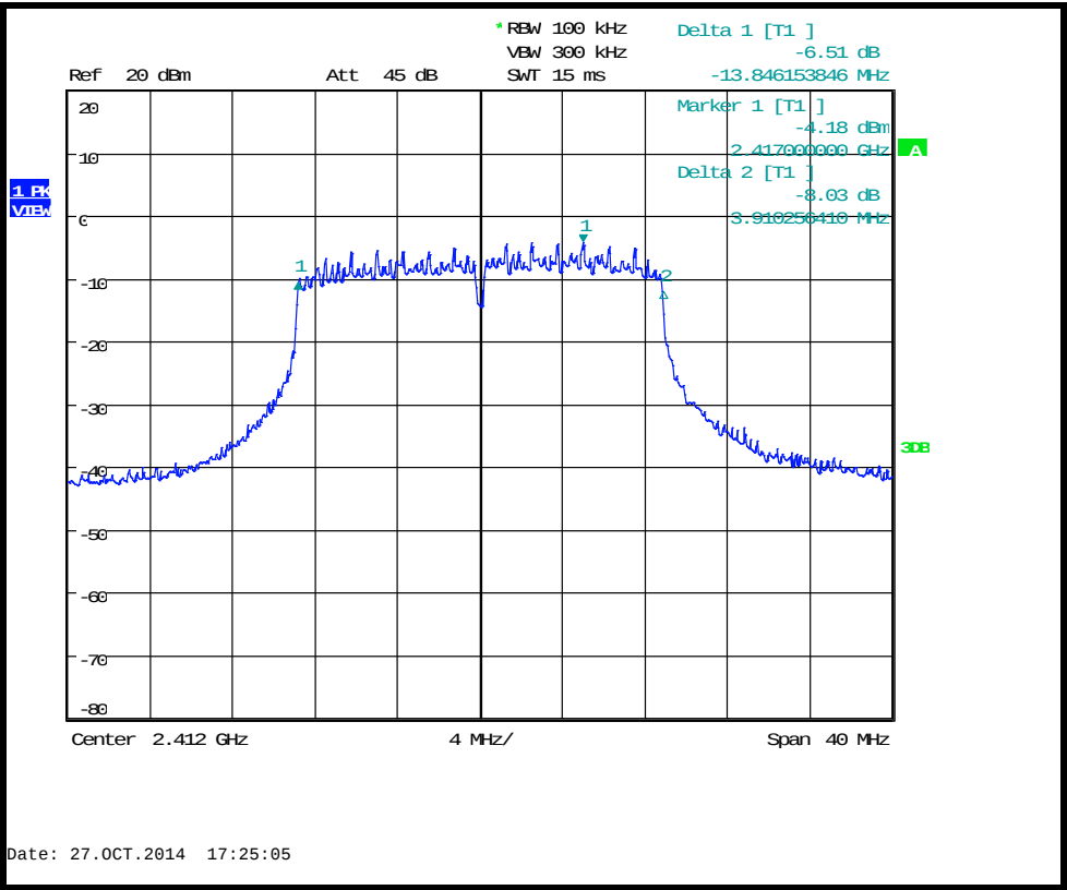
6dB Bandwidth 2412MHz MCS6
