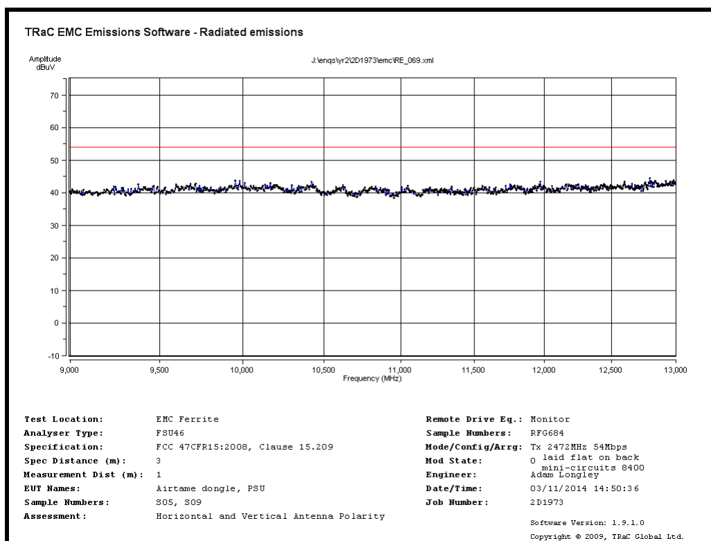
Radiated Spurious emissions 9GHz to 13GHz – 2472MHz 54Mb/s
