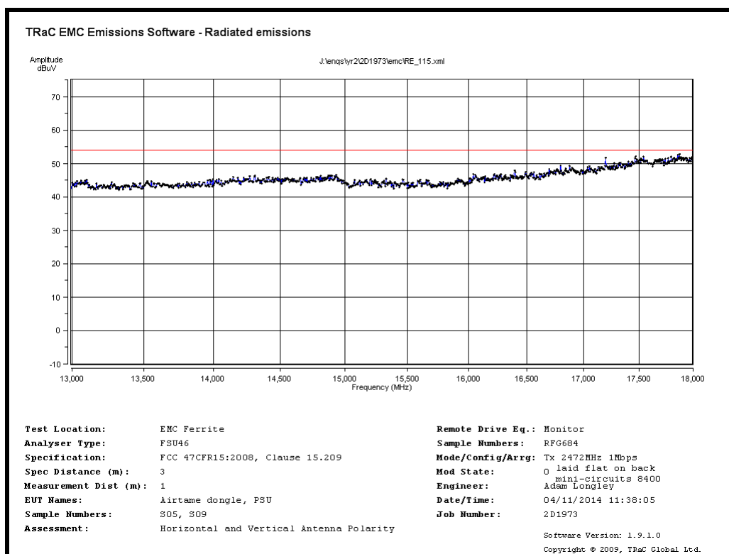
Radiated Spurious emissions 13GHz to 18GHz – 2472MHz 1Mb/s
