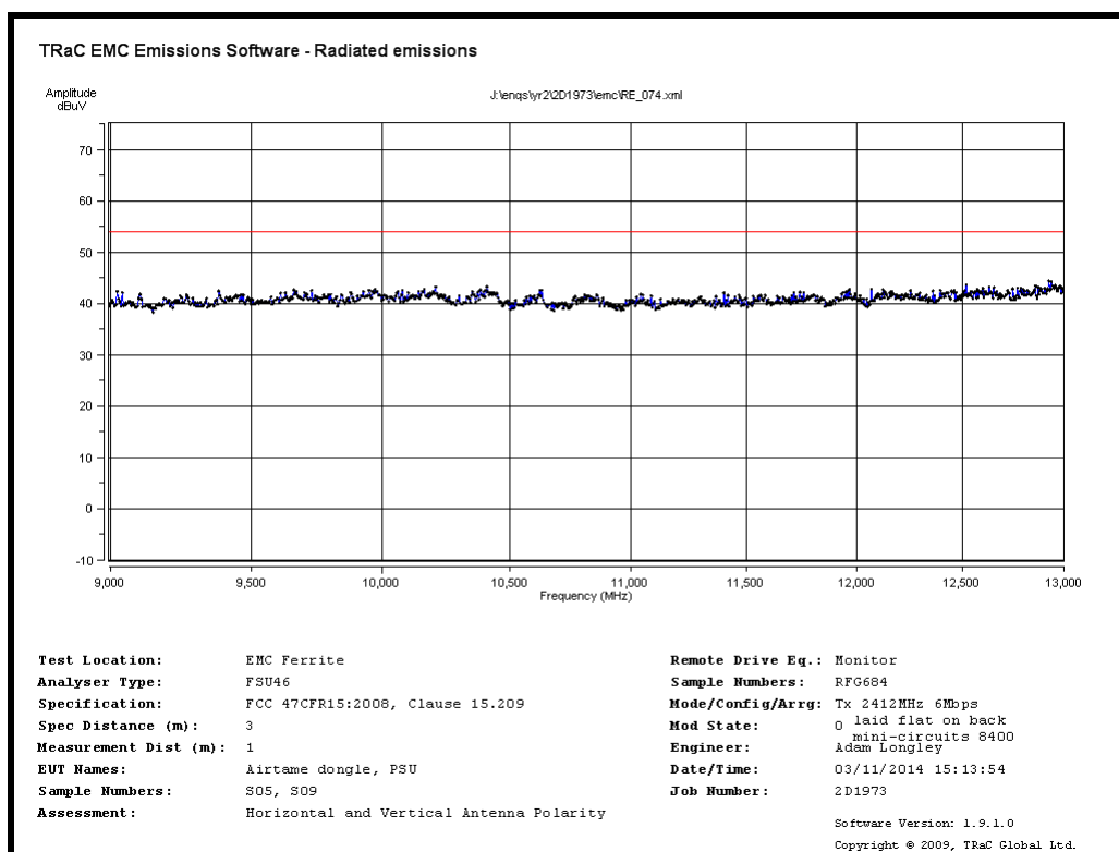
Radiated Spurious emissions 9GHz to 13GHz – 2412MHz 6Mb/s
