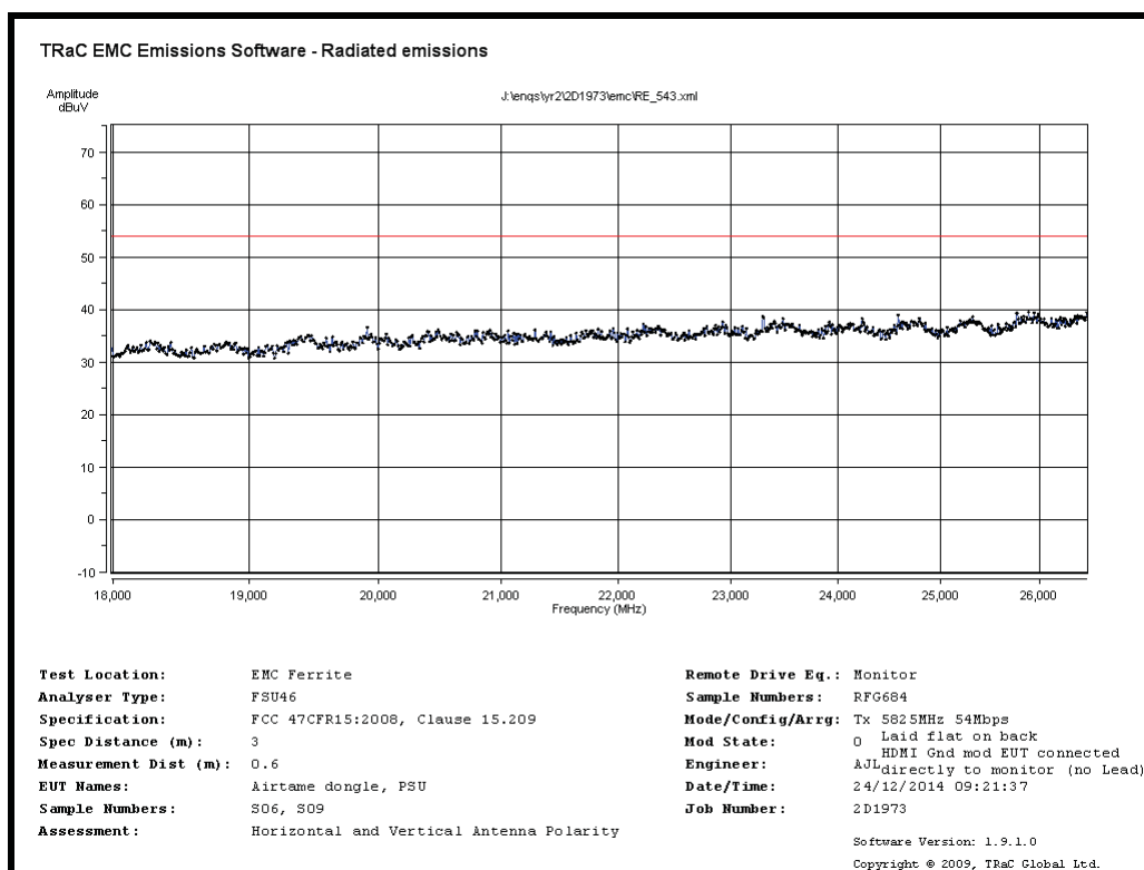
Radiated Spurious emissions 18GHz to 26.5GHz – 5825MHz 54Mb/s
