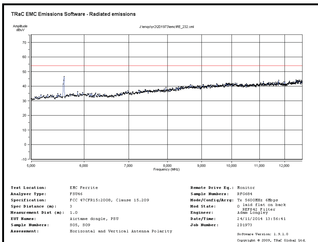
Radiated Spurious emissions 5GHz to 12.5GHz – 5600MHz 6Mb/s
