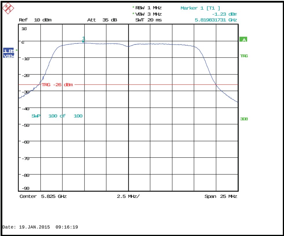
Conducted power spectral density 5825MHz 54Mb/s
