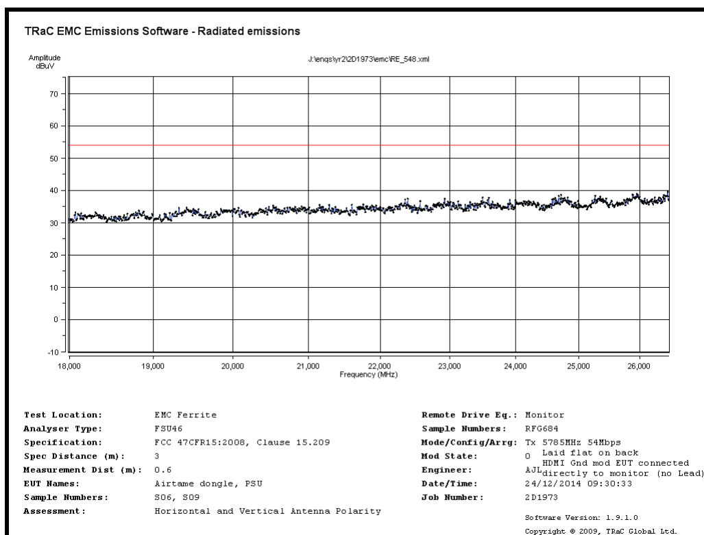
Radiated Spurious emissions 18GHz to 26.5GHz – 5785MHz 54Mb/s
