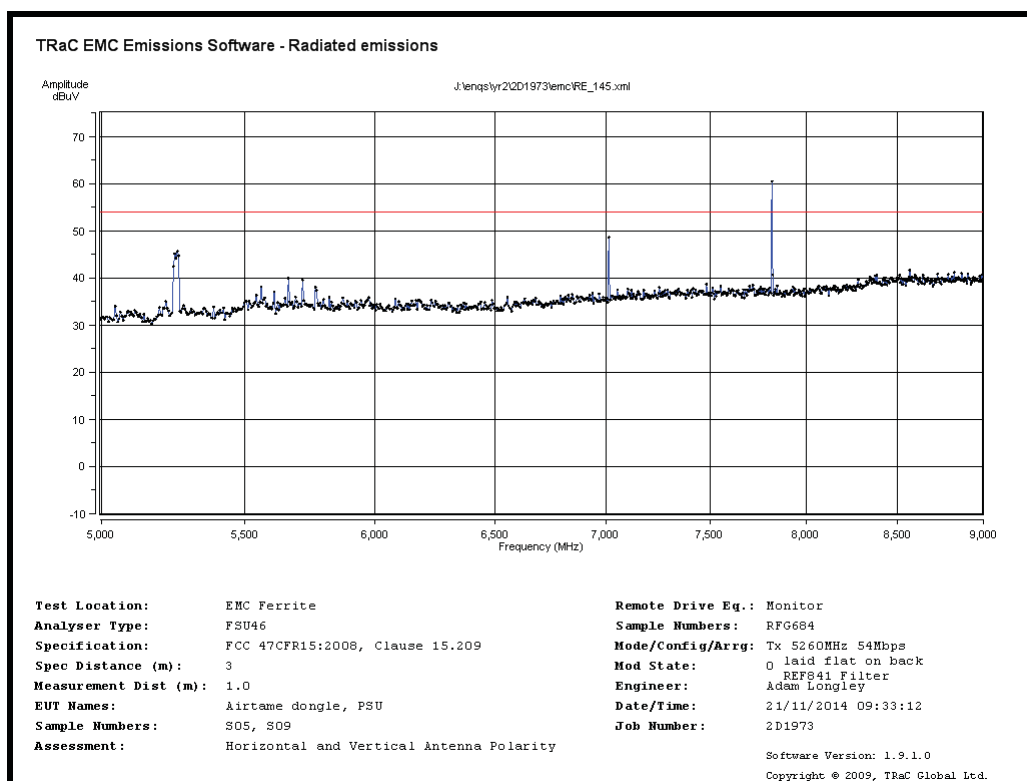
Radiated Spurious emissions 5GHz to 9GHz – 5260MHz 54Mb/s
