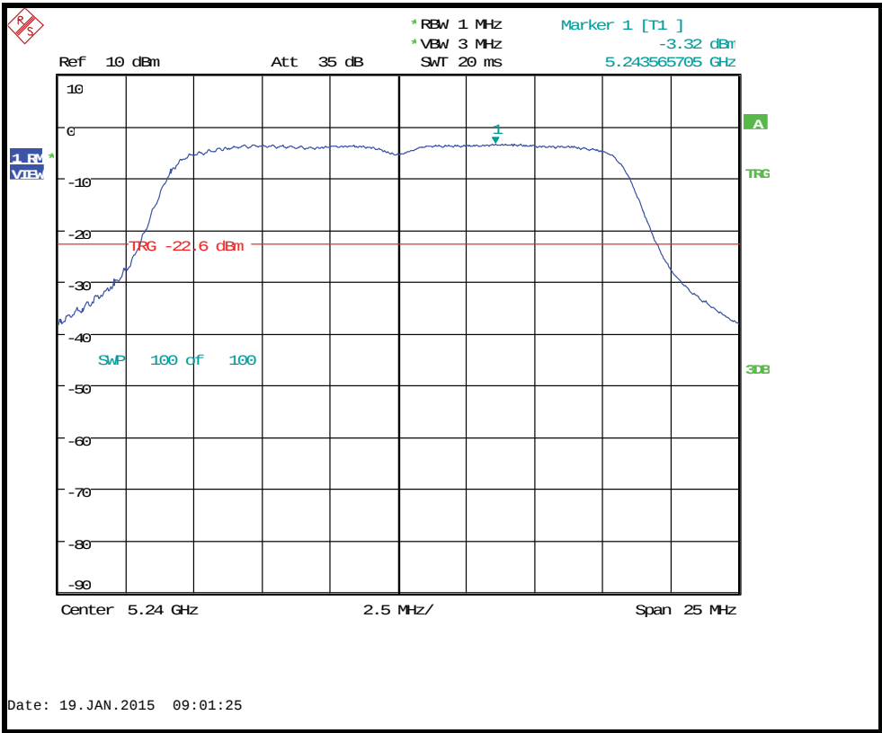
Conducted power spectral density 5240MHz 54Mb/s
