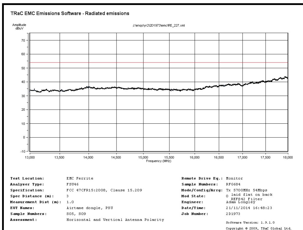
Radiated Spurious emissions 13GHz to 18GHz – 5700MHz 54Mb/s
