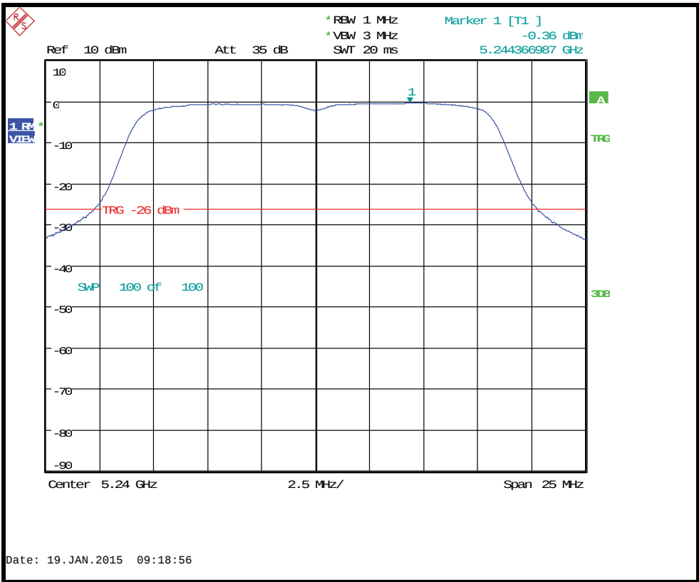
Conducted power spectral density 5240MHz 6Mb/s
