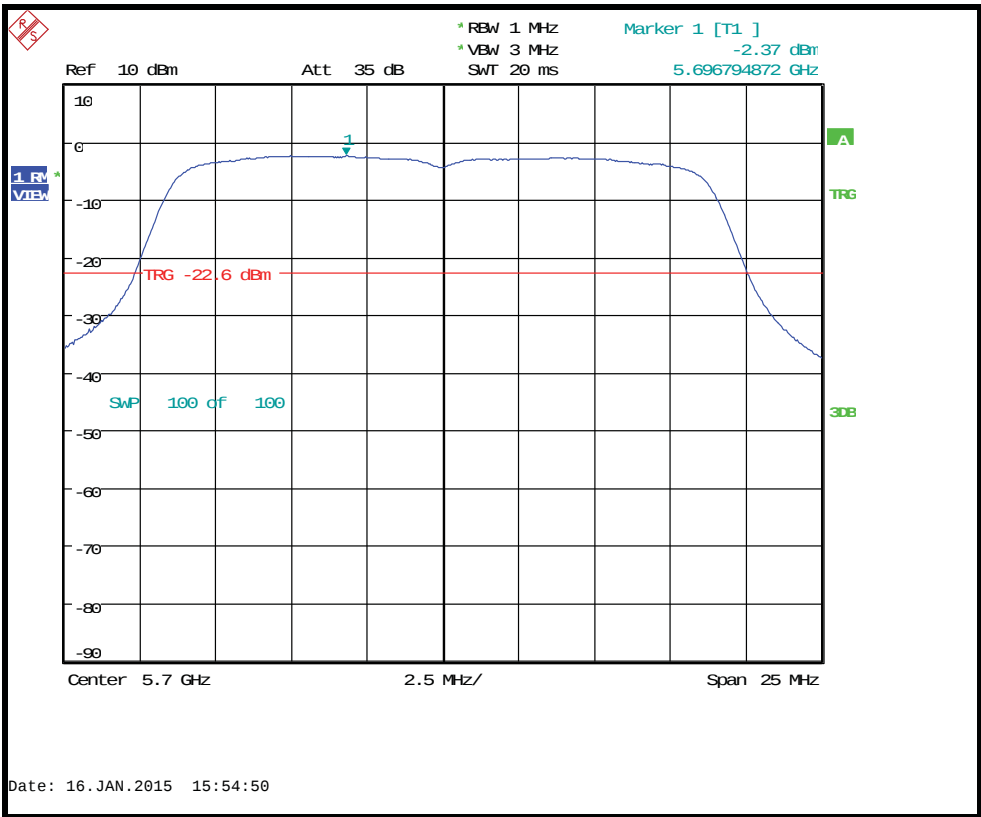
Conducted power spectral density 5700MHz MCS0
