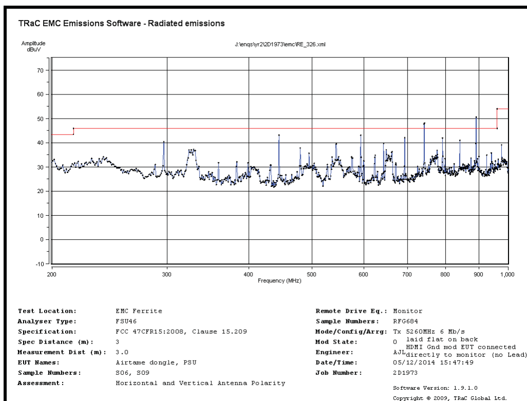
Radiated Spurious emissions 200MHz to 1GHz – 5260MHz 6Mb/s
