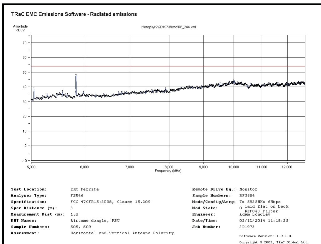
Radiated Spurious emissions 5GHz to 12.5GHz – 5825MHz 6Mb/s
