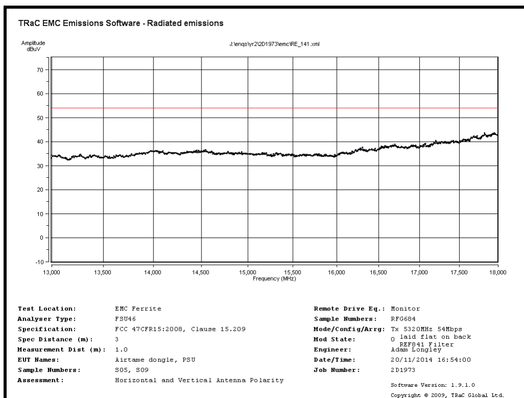
Radiated Spurious emissions 13GHz to 18GHz – 5320MHz 54Mb/s
