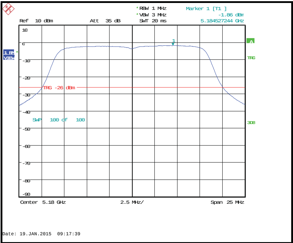
Conducted power spectral density 5180MHz 6Mb/s
