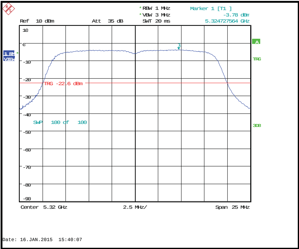
Conducted power spectral density 5320MHz MCS6
