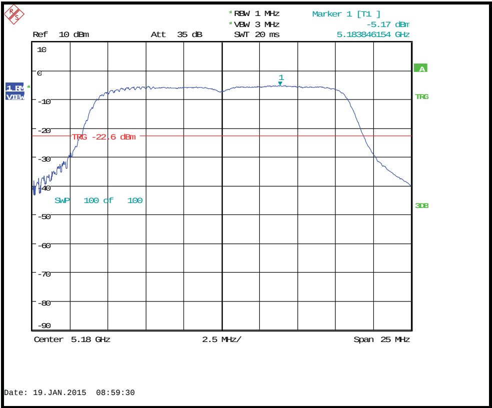
Conducted power spectral density 5180MHz 54Mb/s
