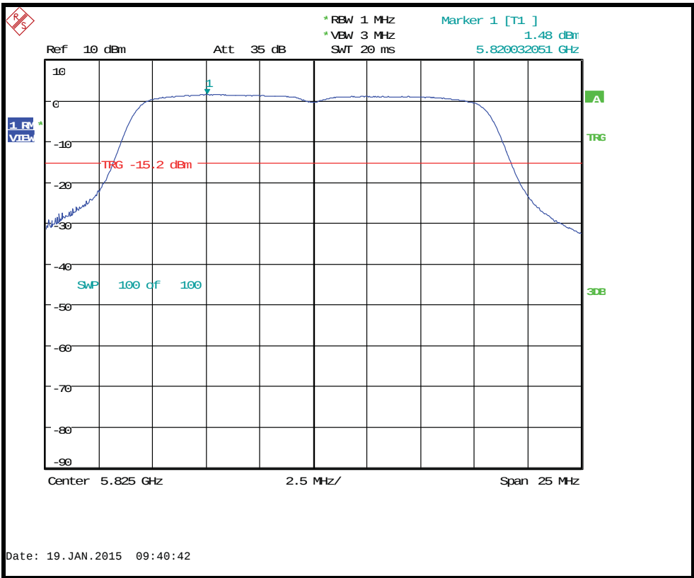
Conducted power spectral density 5825MHz 6Mb/s
