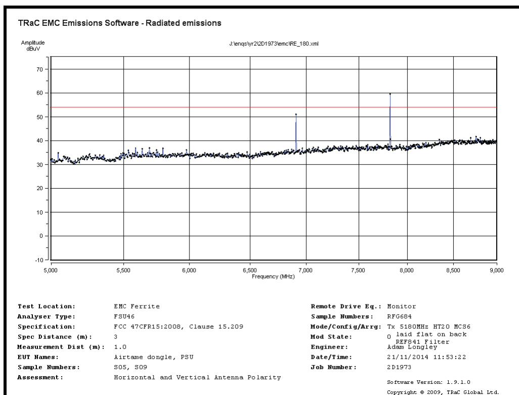
Radiated Spurious emissions 5GHz to 9GHz – 5180MHz MCS6
