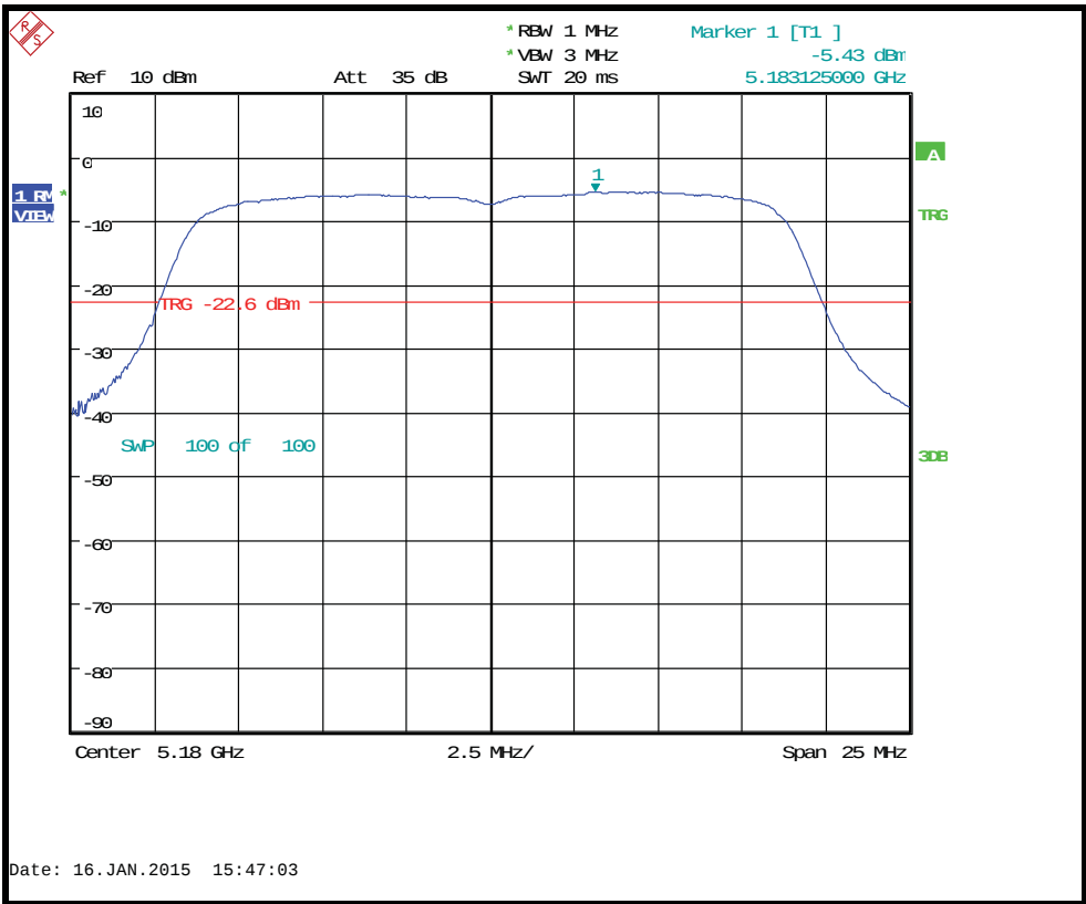
Conducted power spectral density 5180MHz MCS0
