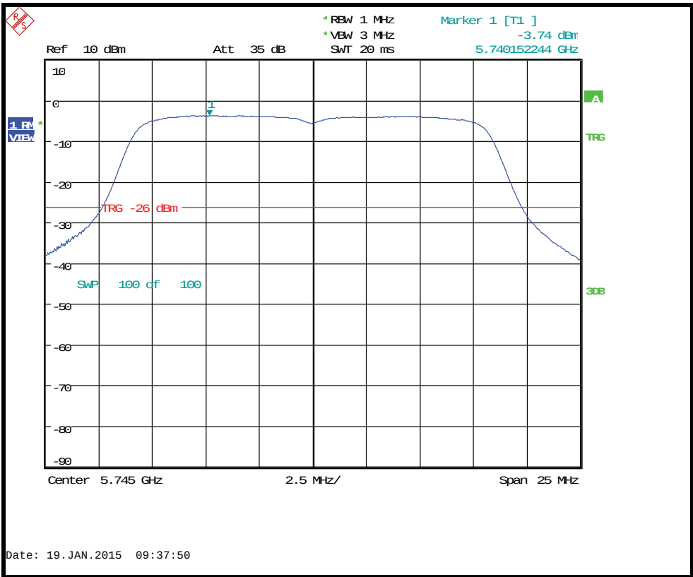
Conducted power spectral density 5745MHz 6Mb/s
