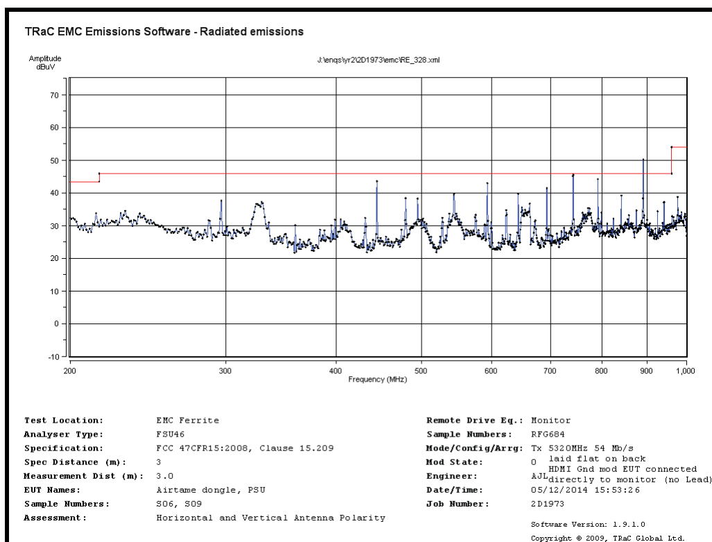
Radiated Spurious emissions 200MHz to 1GHz – 5320MHz 54Mb/s
