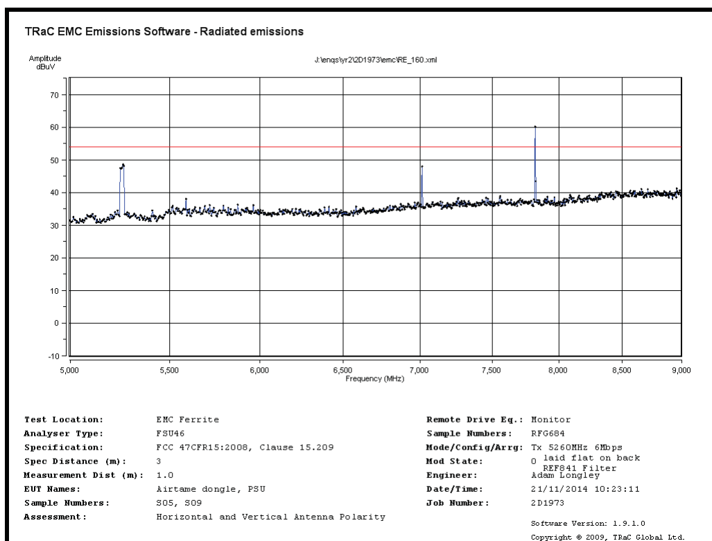
Radiated Spurious emissions 5GHz to 9GHz – 5260MHz 6Mb/s
