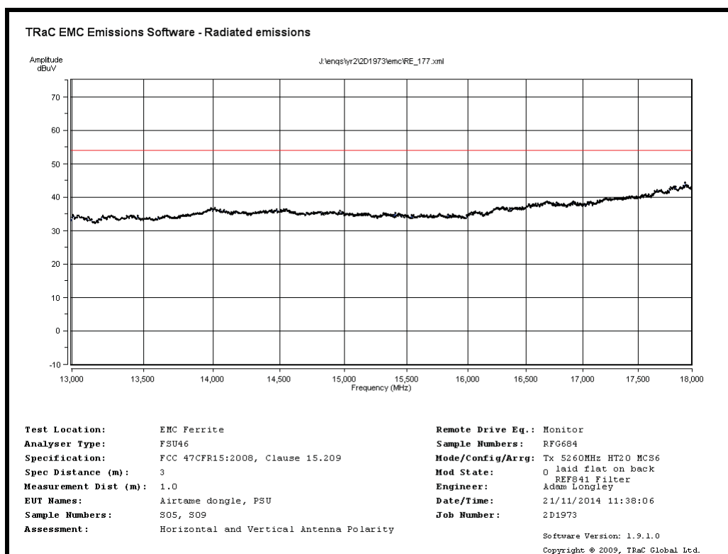
Radiated Spurious emissions 13GHz to 18GHz – 5260MHz MCS6
