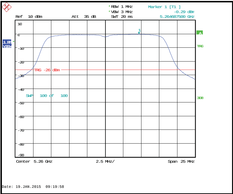
Conducted power spectral density 5260MHz 6Mb/s
