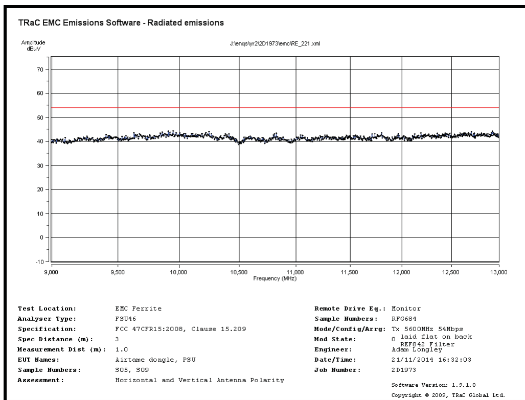
Radiated Spurious emissions 9GHz to 13GHz – 5600MHz 54Mb/s
