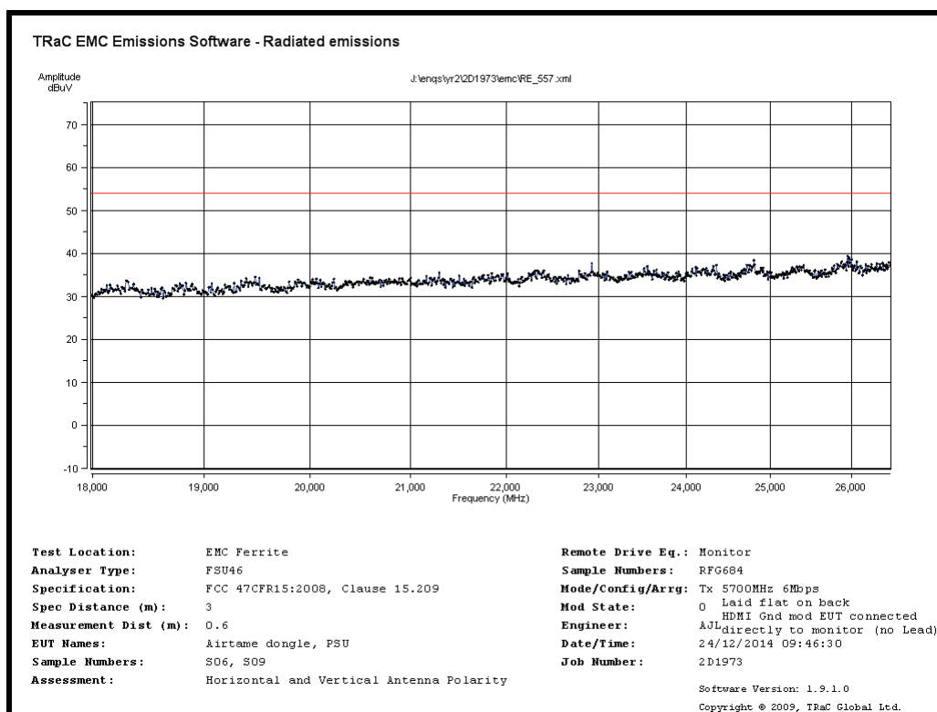
Radiated Spurious emissions 18GHz to 26.5GHz – 5700MHz 6Mb/s
