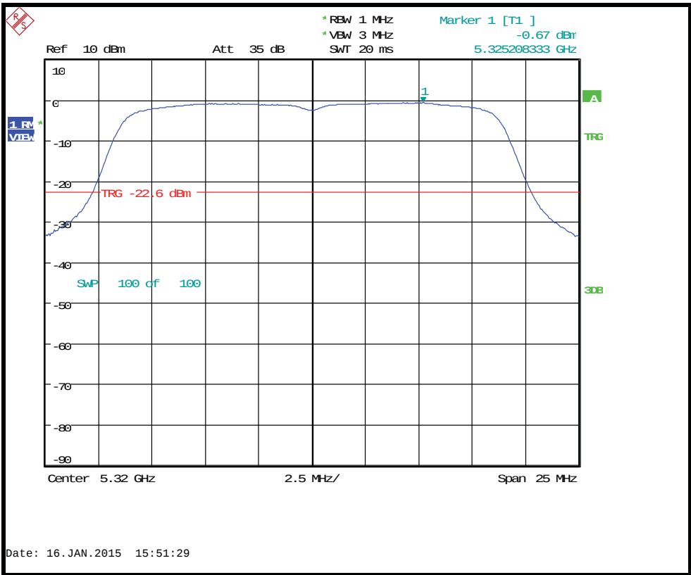
Conducted power spectral density 5320MHz MCS0
