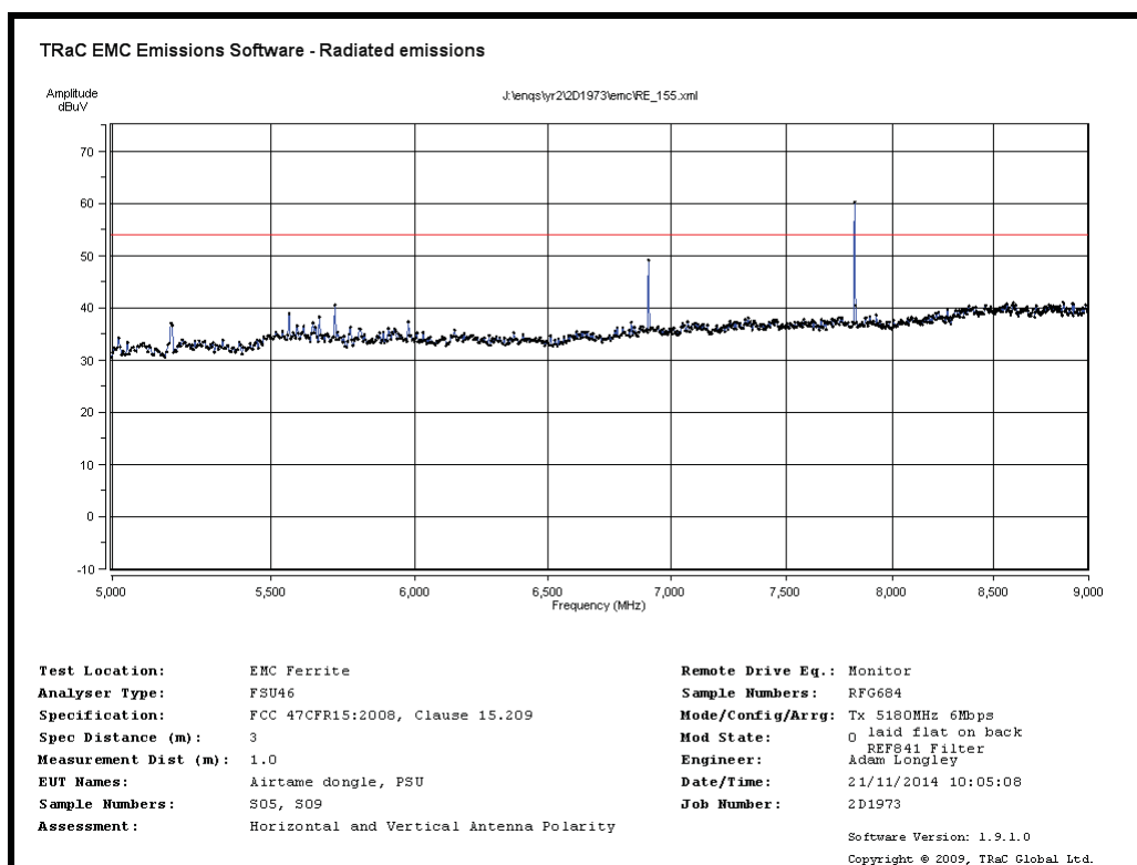
Radiated Spurious emissions 5GHz to 9 GHz – 5180MHz 6Mb/s
