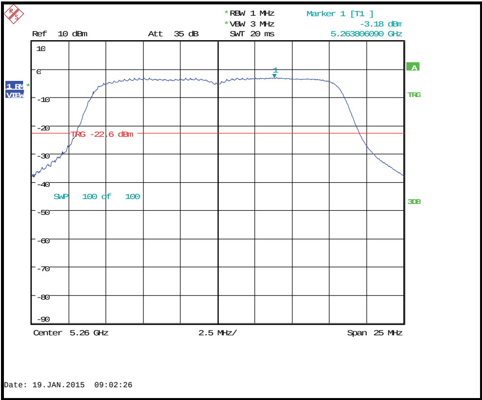
Conducted power spectral density 5260MHz 54Mb/s
