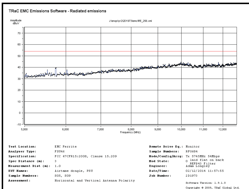
Radiated Spurious emissions 5GHz to 12.5GHz – 5745MHz 54Mb/s
