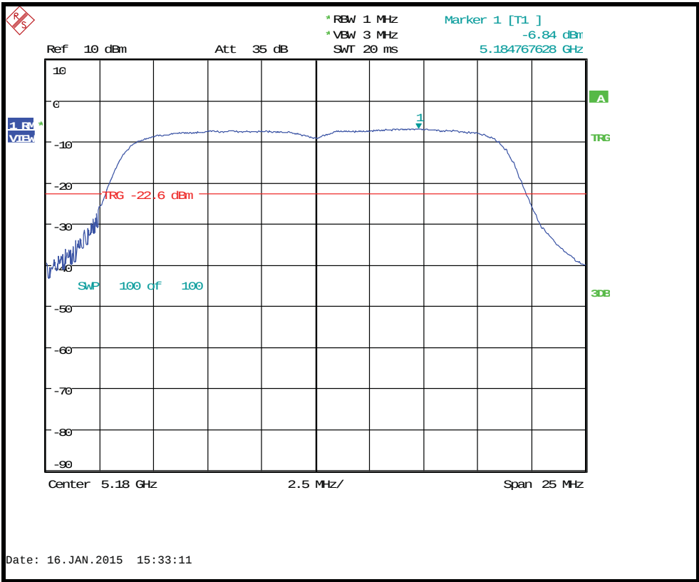
Conducted power spectral density 5180MHz MCS6
