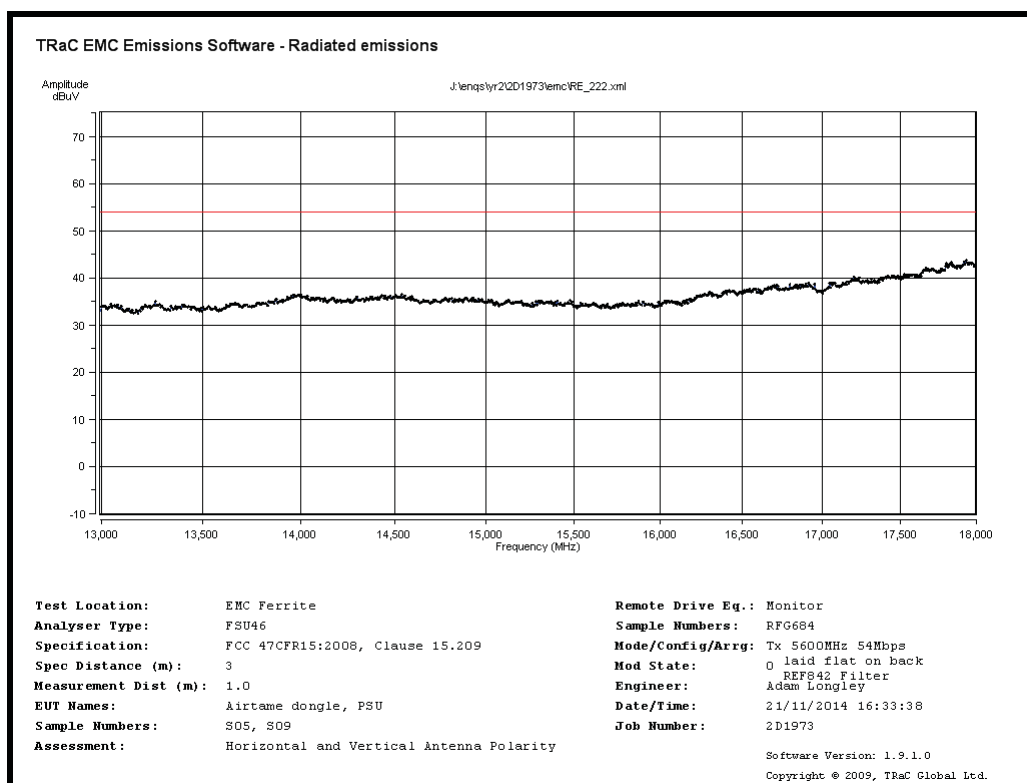
Radiated Spurious emissions 13 GHz to 18GHz – 5600MHz 54Mb/s
