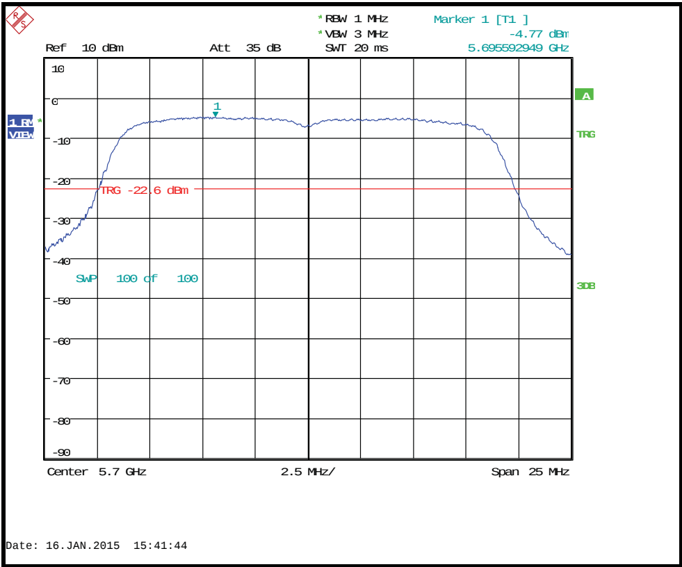
Conducted power spectral density 5700MHz MCS6
