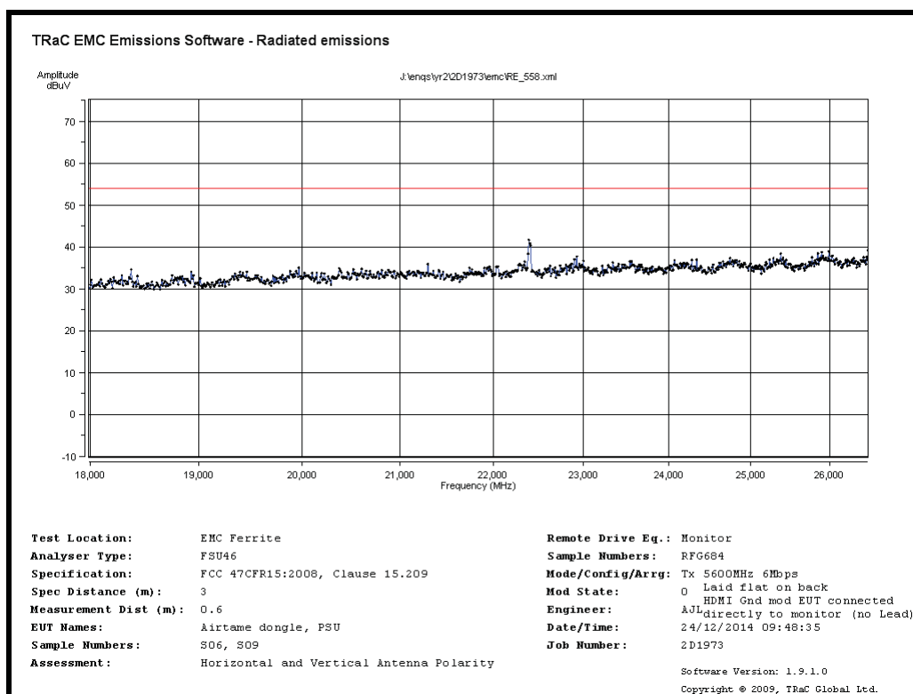
Radiated Spurious emissions 18GHz to 26.5GHz – 5600MHz 6Mb/s
