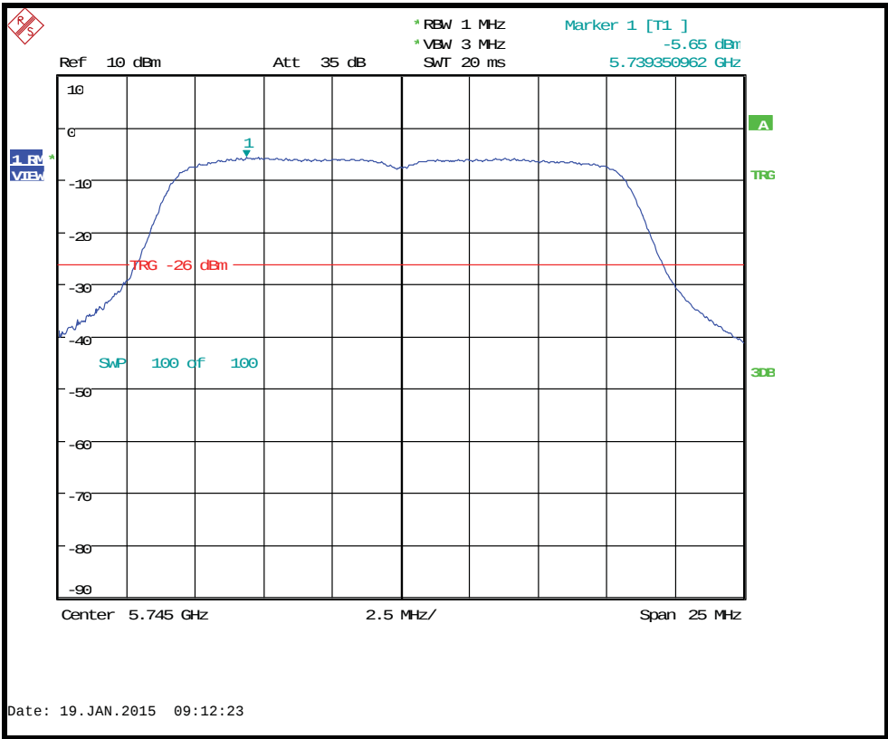
Conducted power spectral density 5745MHz 54Mb/s
