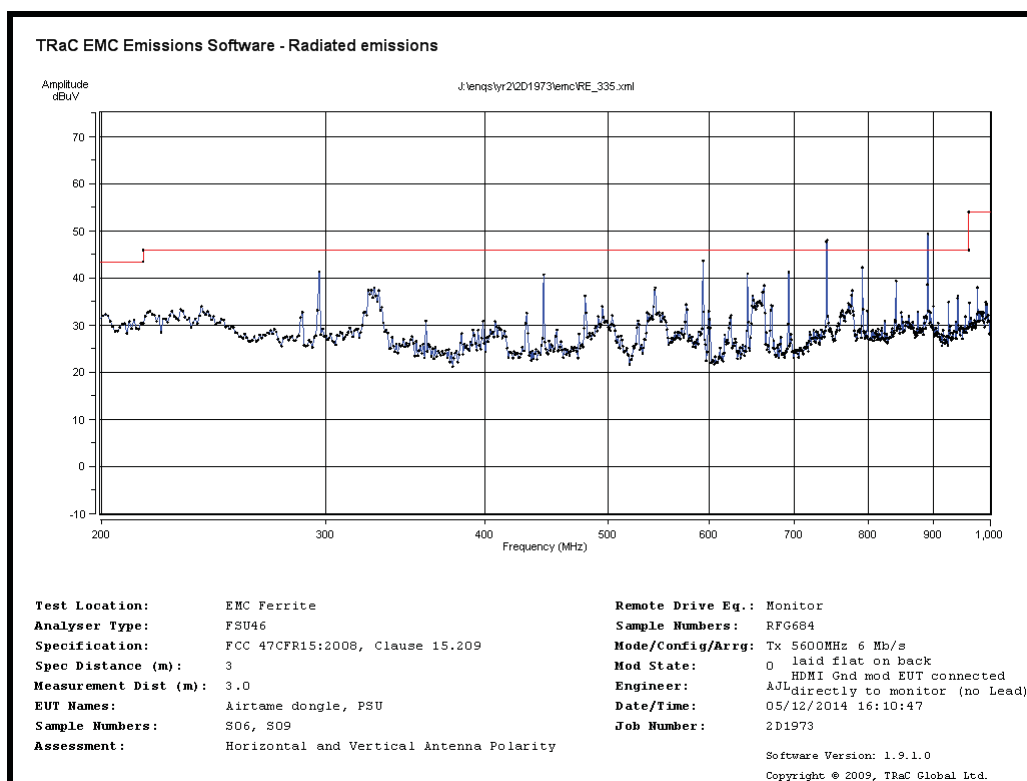
Radiated Spurious emissions 200MHz to 1GHz – 5600MHz 6Mb/s
