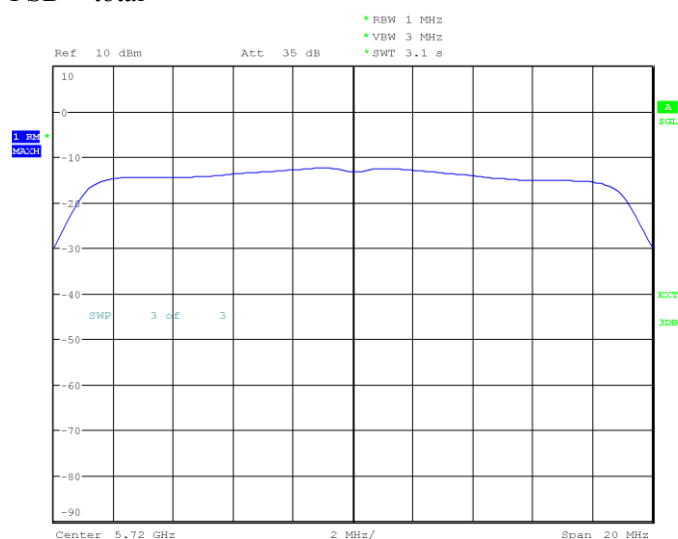
PSD – total
