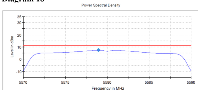
PSD – total
