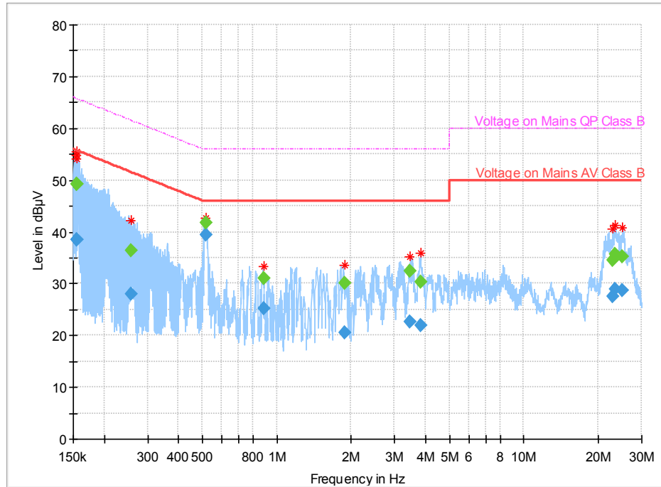
Full Spectrum
