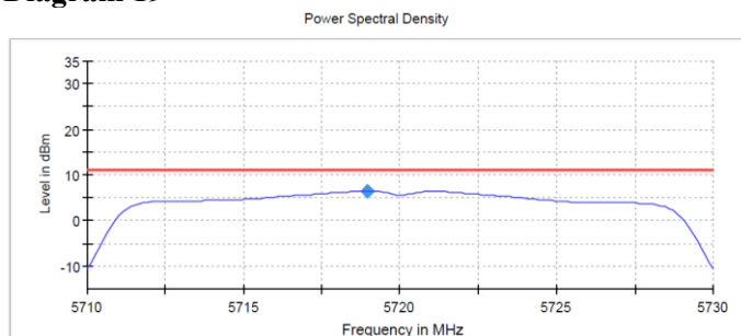
PSD – total
