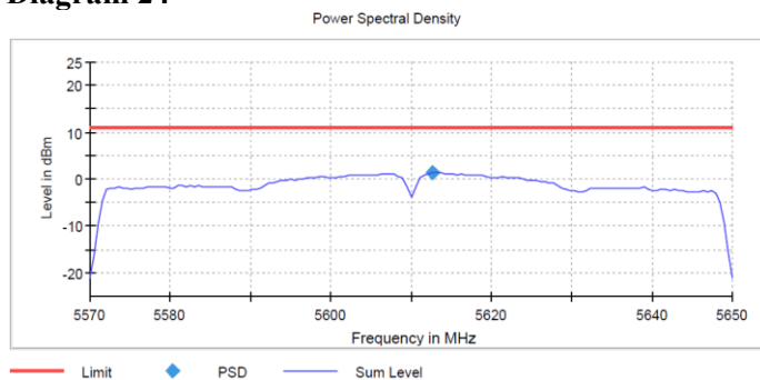
PSD – total
