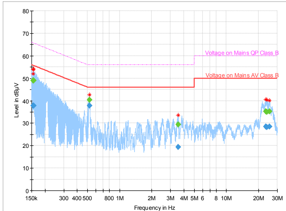
Full Spectrum
