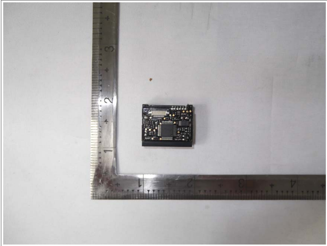
Side PCB(Top)
