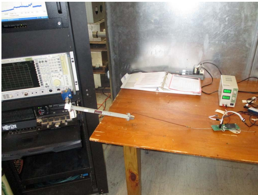
Test Setup, 18 GHz to 25 GHz
