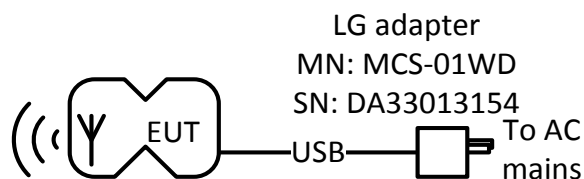
Figure 3.6-1: Setup diagram
