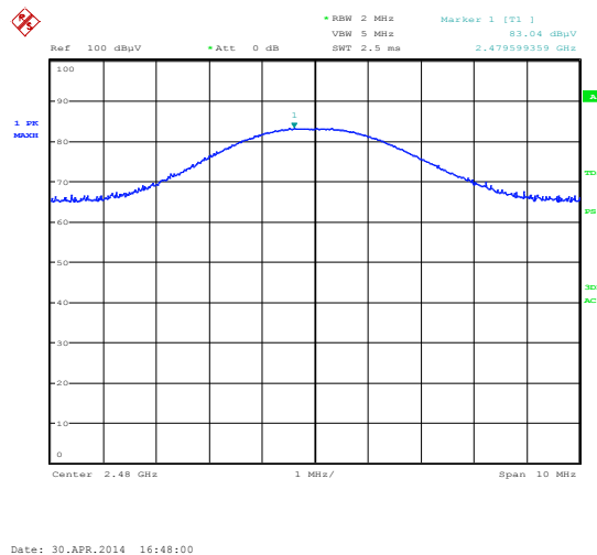
Figure 8.4-1: Field strength of fundamental, sample plot
