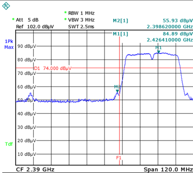
Band Edge, Left Side (Peak) - 802.11n40
