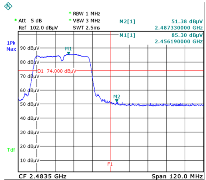
Band Edge, Right Side (Peak) - 802.11n40
