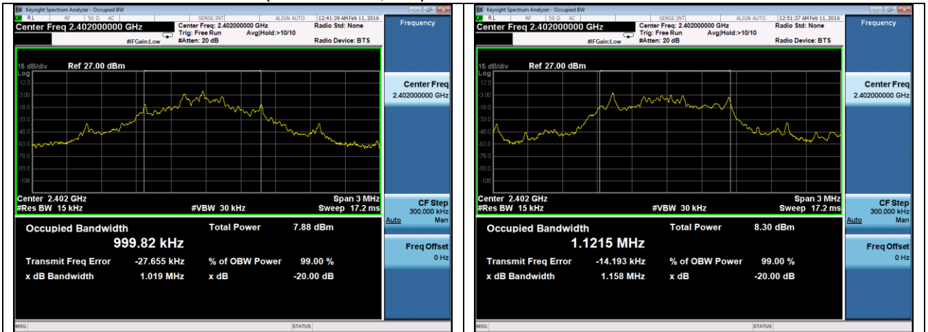
99% and 20dB BW –Bluetooth BDR 2402MHz
