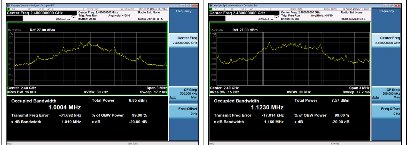
99% and 20dB BW –Bluetooth BDR 2480MHz
