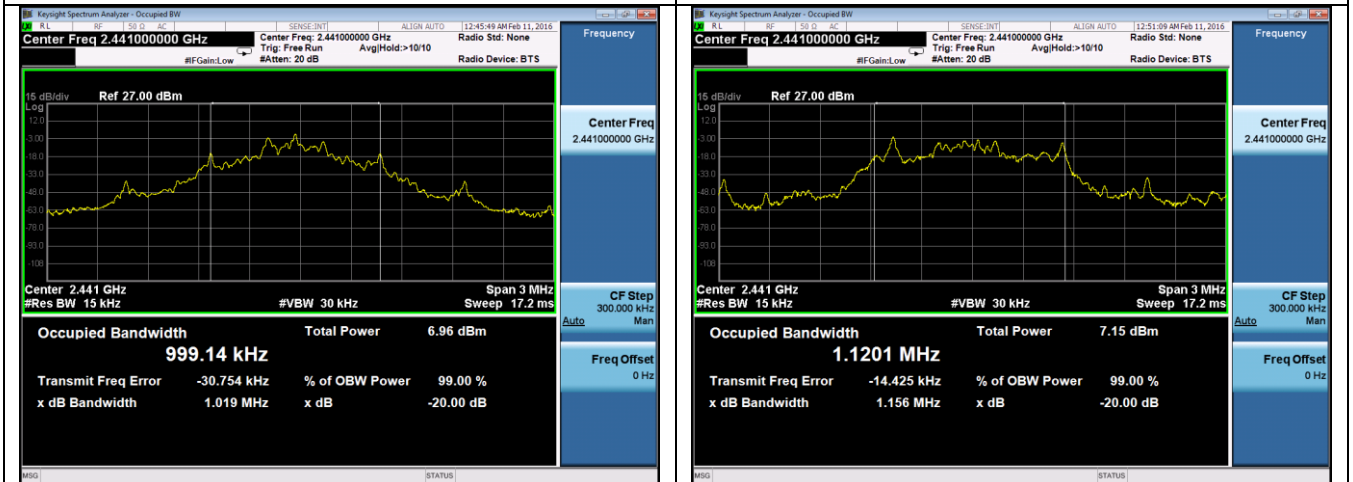
99% and 20dB BW –Bluetooth BDR 2441MHz
