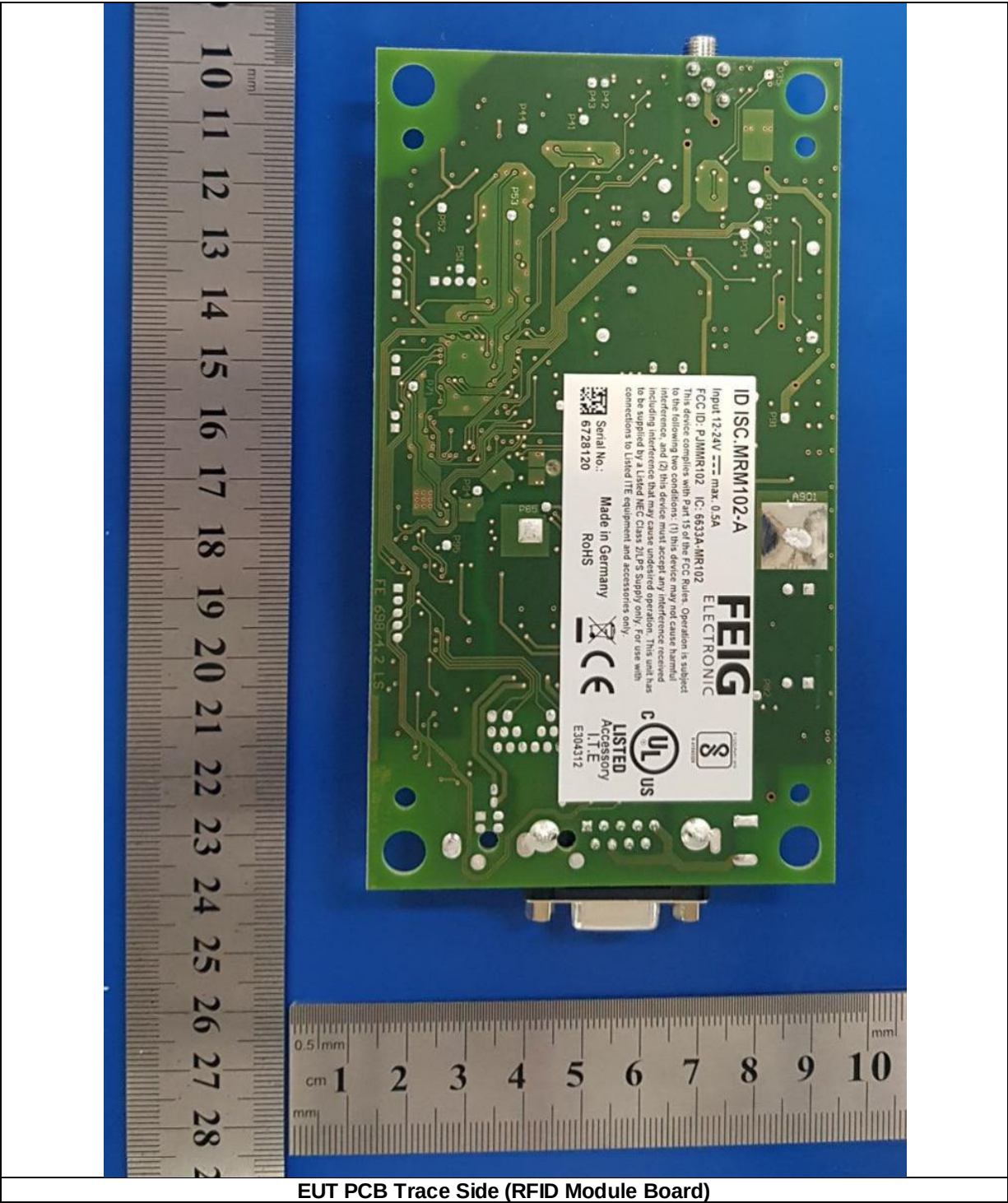
EUT PCB Trace Side (RFID Module Board)
