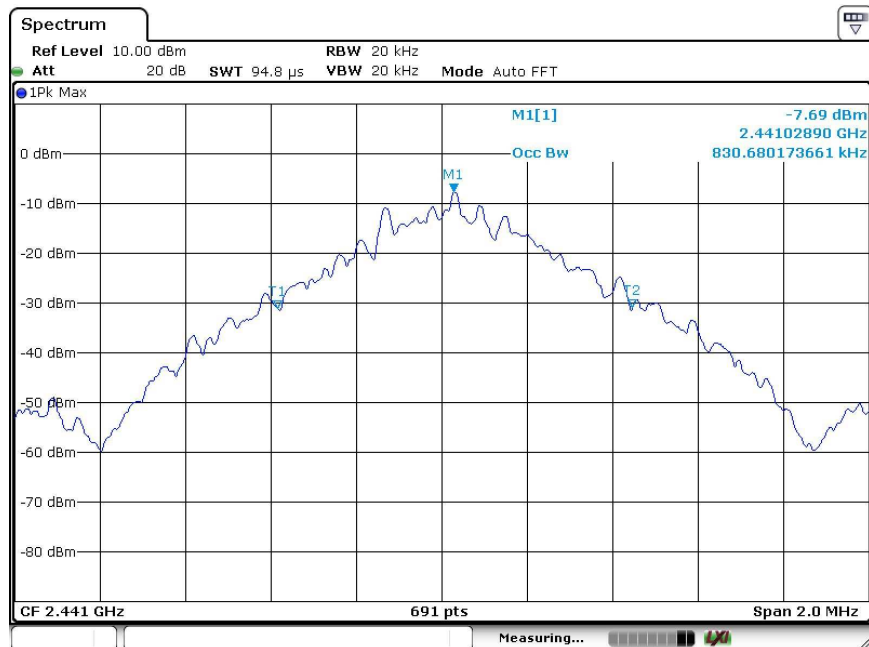
2441MHz, GFSK
