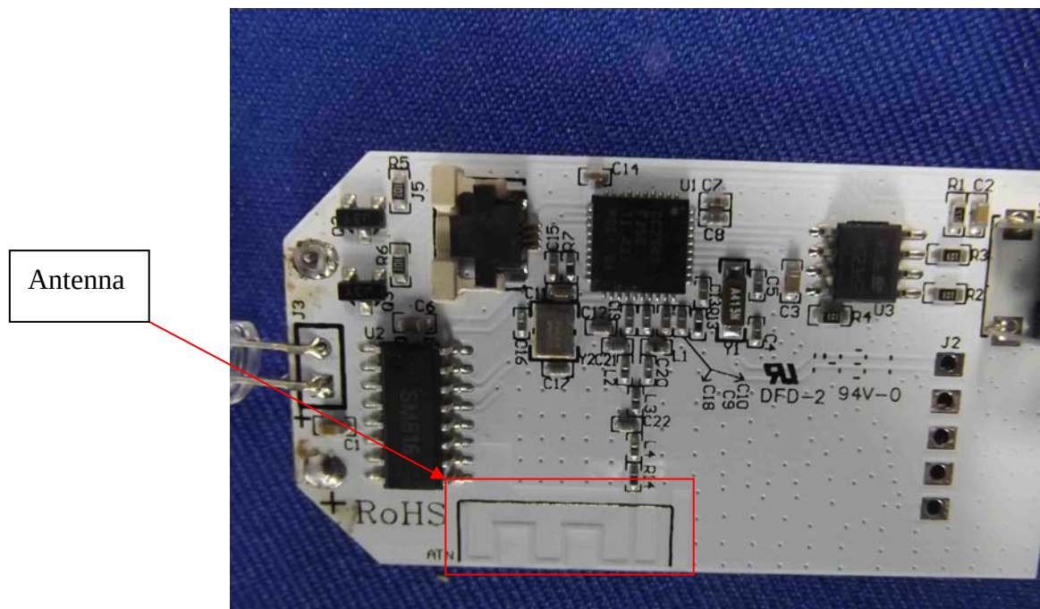
PCB of the Module View
