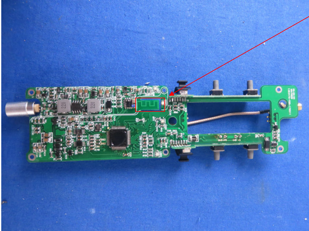
BT4.0 ANT
