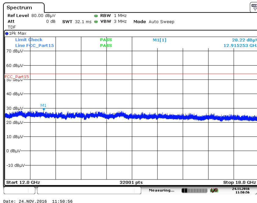
Plot 8: 12 GHz to 18 GHz, TX mode, channel 79, vertical & horizontal polarization
