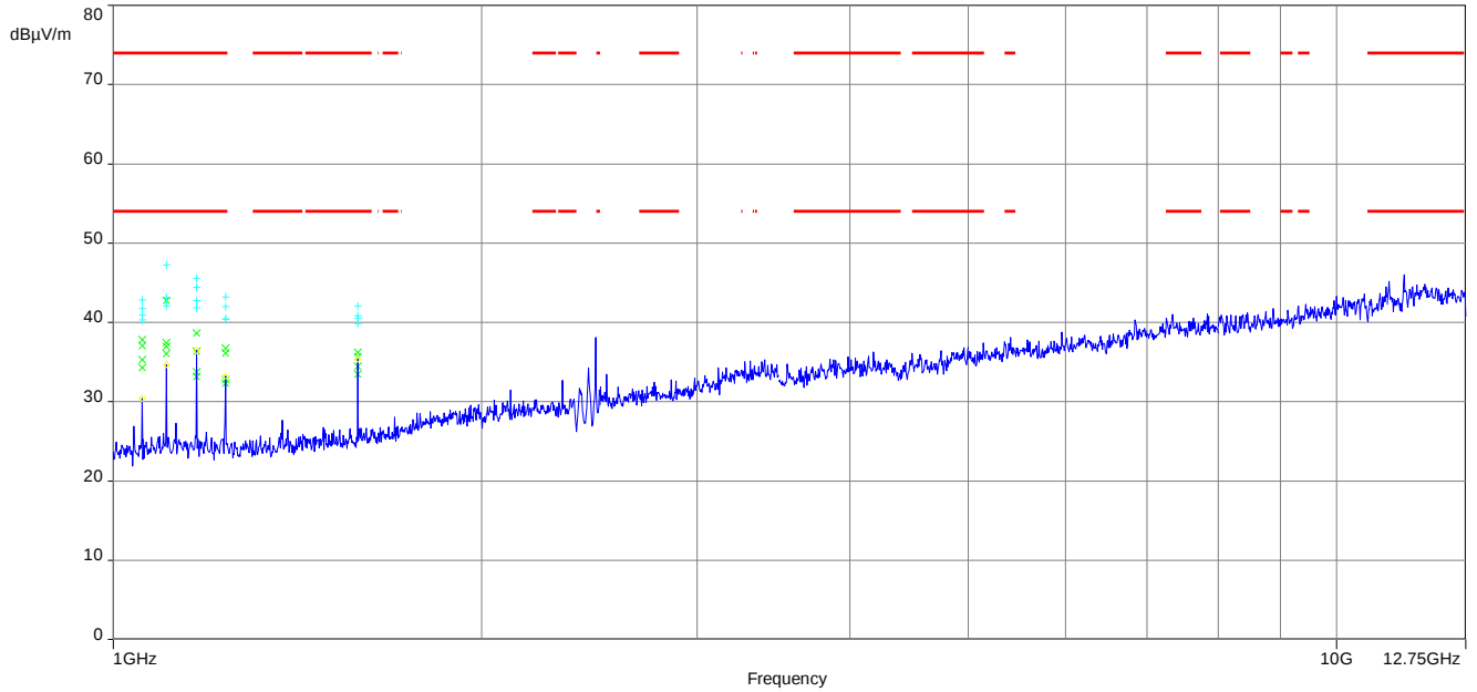
Plot 7: 1 GHz to 12.75 GHz, TX mode, channel 79, vertical & horizontal polarization
