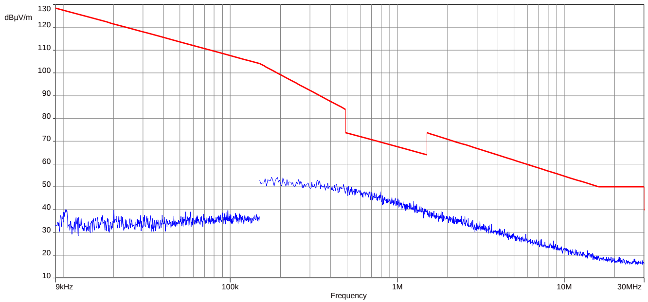
Plot 3: 9 kHz to 30 MHz, channel 79, transmit mode
