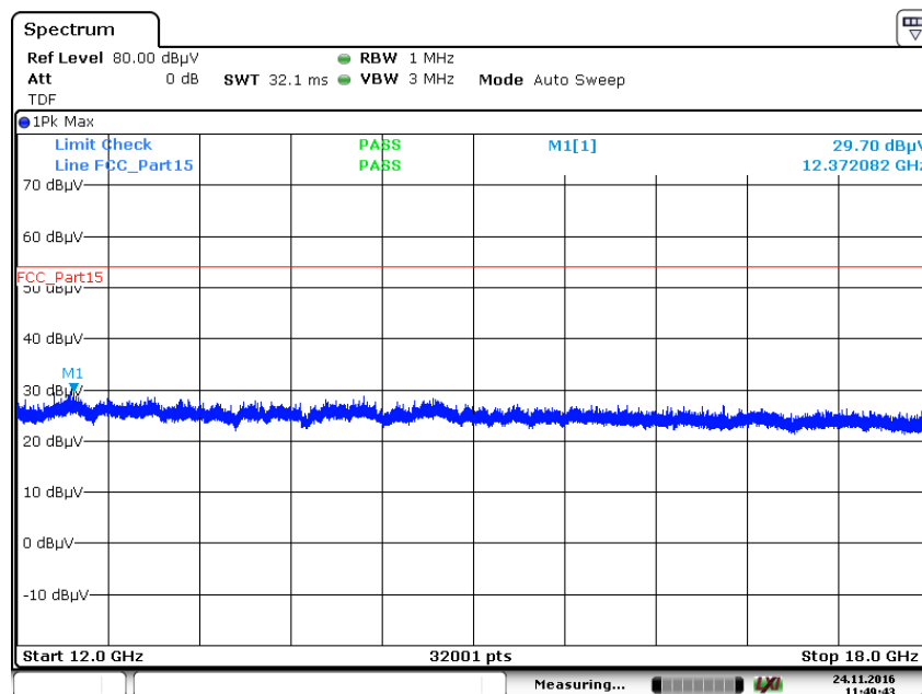
Plot 5: 12 GHz to 18 GHz, TX mode, channel 19, vertical & horizontal polarization
