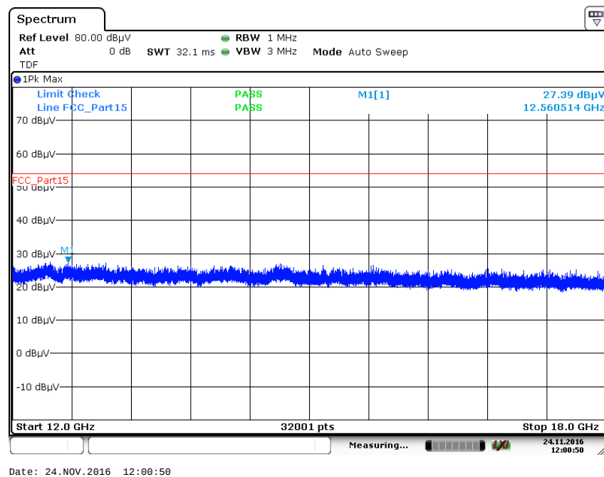
Plot 2: 12 GHz to 18 GHz, RX / idle – mode, vertical & horizontal polarization
