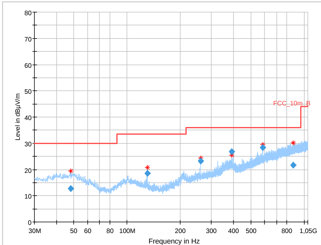
Plot 3: 30 MHz to 1 GHz, TX mode, channel 79, vertical & horizontal polarization
