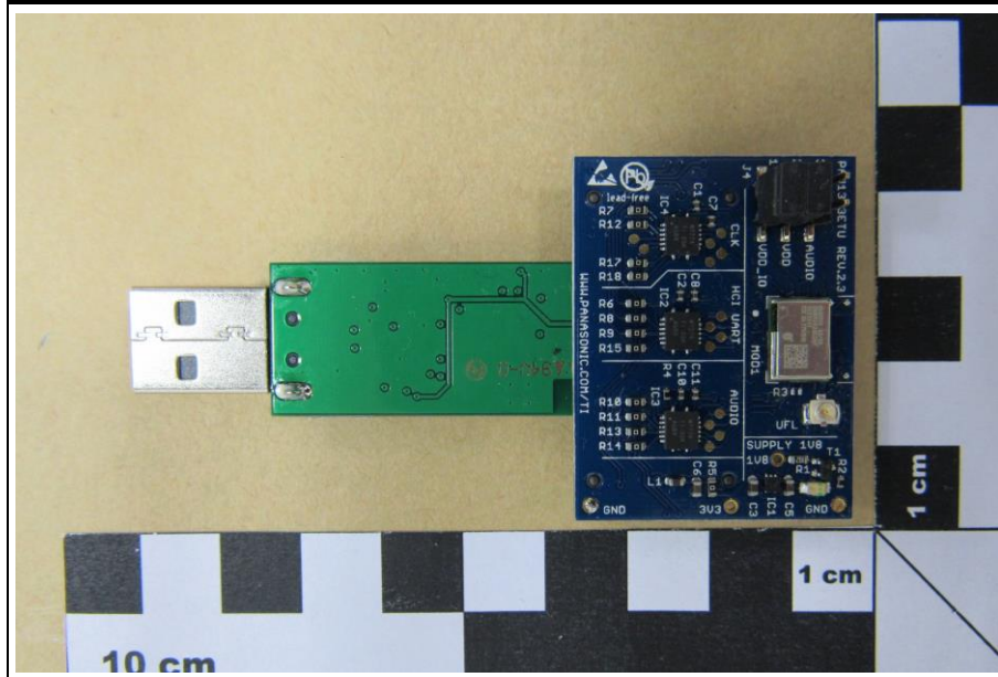
EUT (PAN 1315 - ENW89829C3KF) ON EVALUATION BOARD TOP
