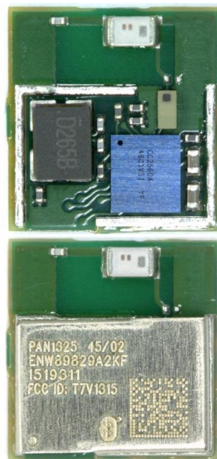
EUT (PAN 1325 - ENW89829A2KF) with and without shielding
