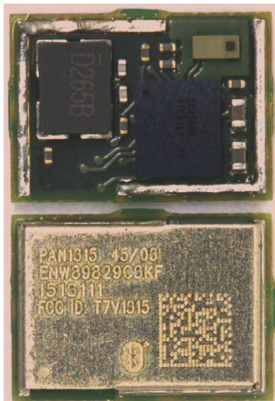
EUT (PAN 1315 - ENW89829C3KF) with and without shielding
