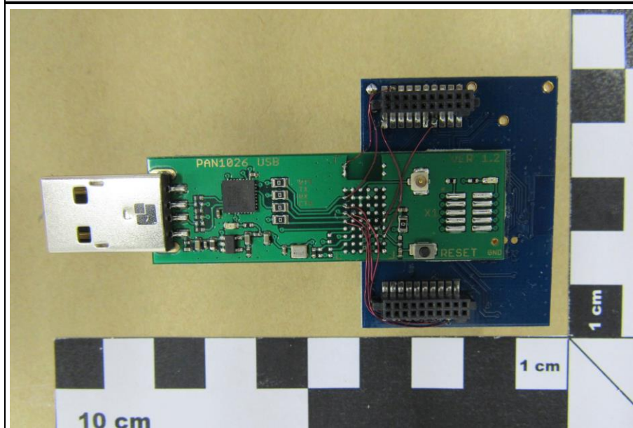
EVALUATION BOARD BOTTOM (PAN 1315 - ENW89829C3KF)
