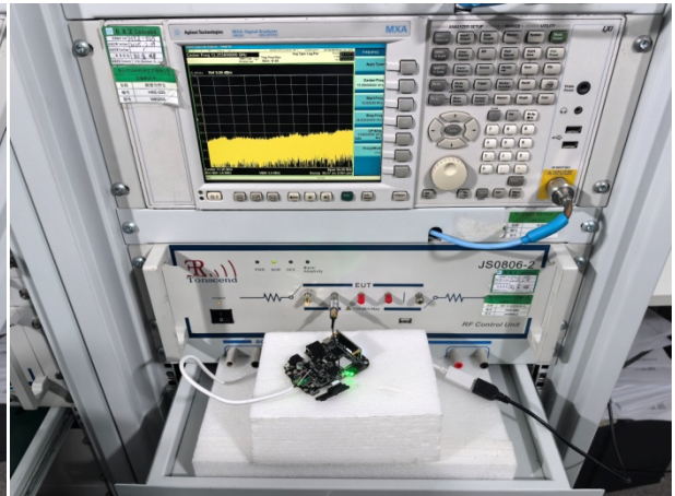
RF Conducted Emission
