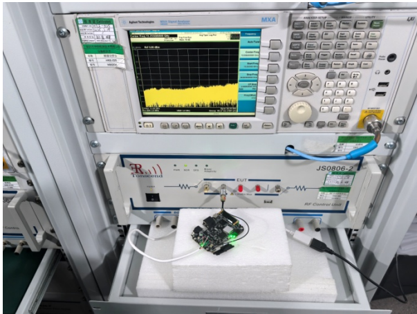
RF Conducted Emission
