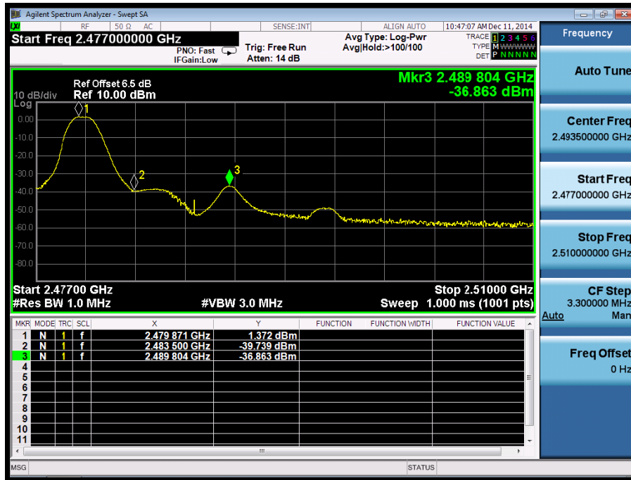
(Plot 6.5.1 A3:Channel 39: 2480MHz @ GFSK)
