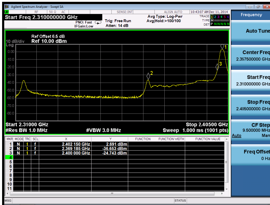
(Plot 6.5.1 A1:Channel 00: 2402MHz @ GFSK)
