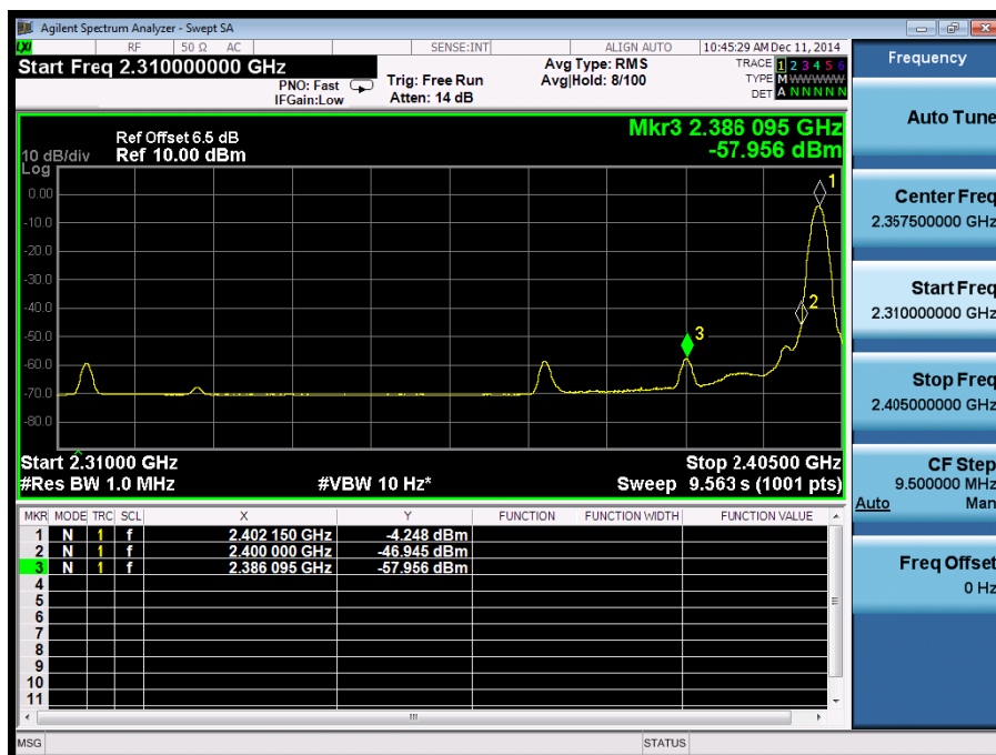
(Plot 6.5.1 A2:Channel 00: 2402MHz @ GFSK)
