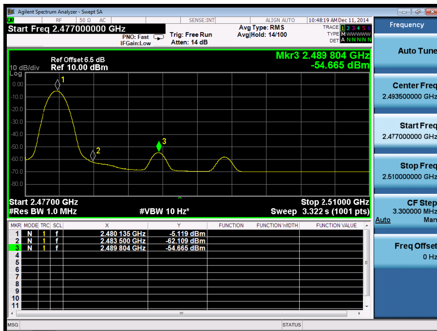
(Plot 6.5.1 A4:Channel 39: 2480MHz @ GFSK)
