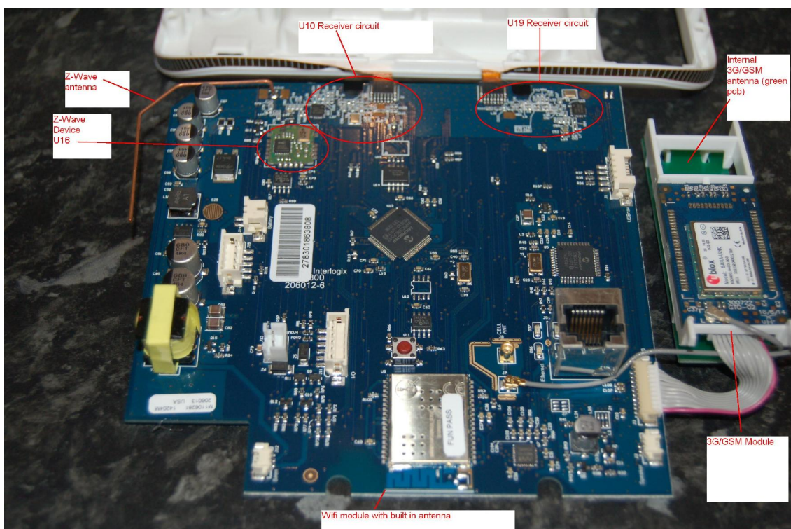
RF Circuit Locations
