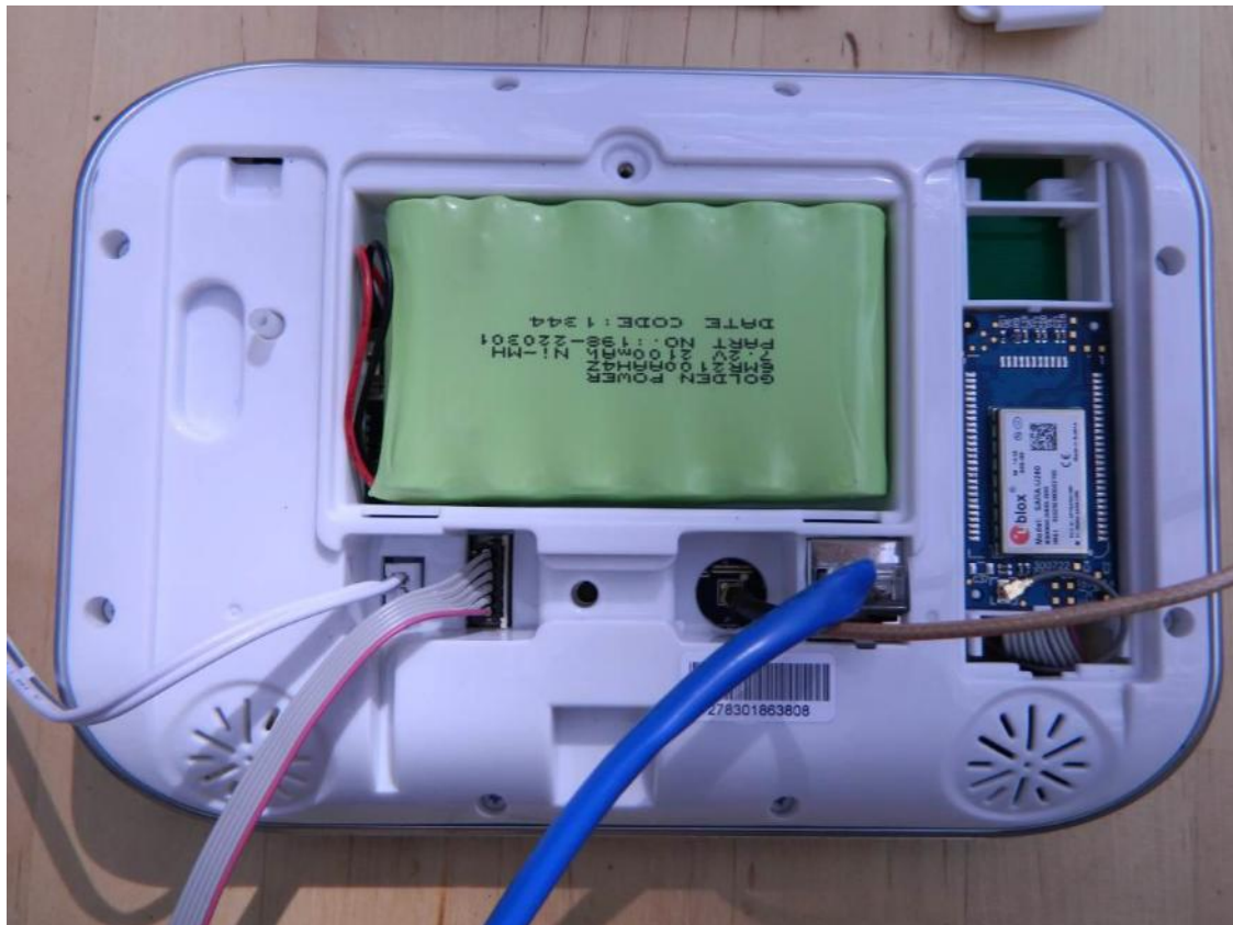
EUT with rear covers removed
