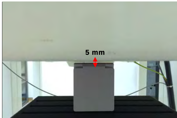
Fig.3 EUT Top side mode to flat phantom
