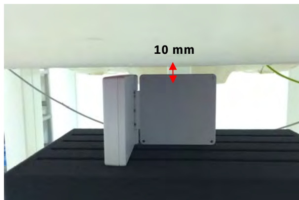
Fig.11 EUT Left side to flat phantom
