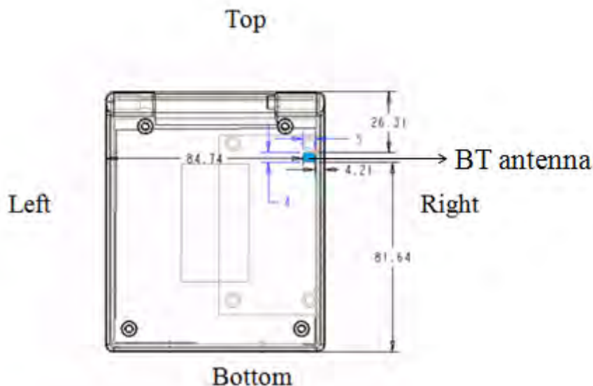
Fig.17 Antenna position of EUT (Front view / Cover closed)
