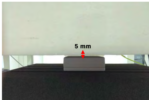
Fig.7 EUT Back side to flat phantom
