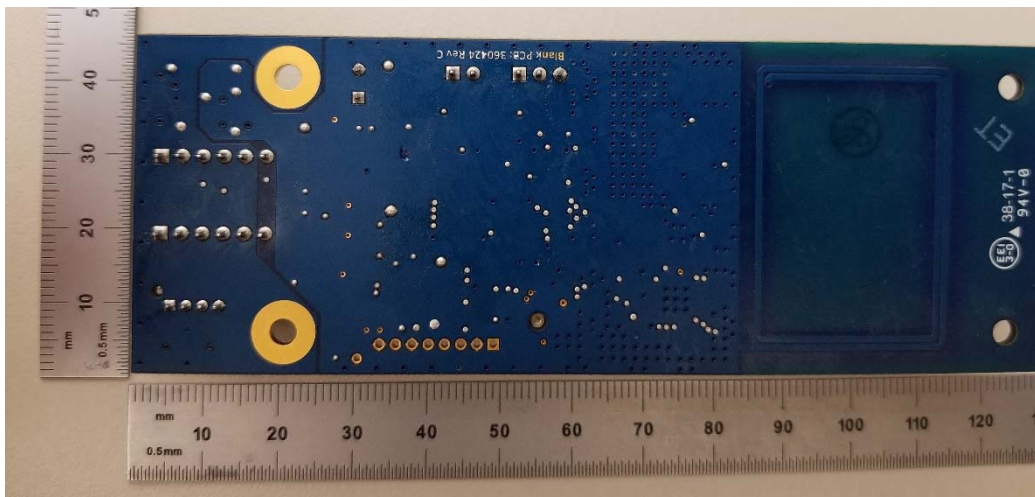
Bottom view
