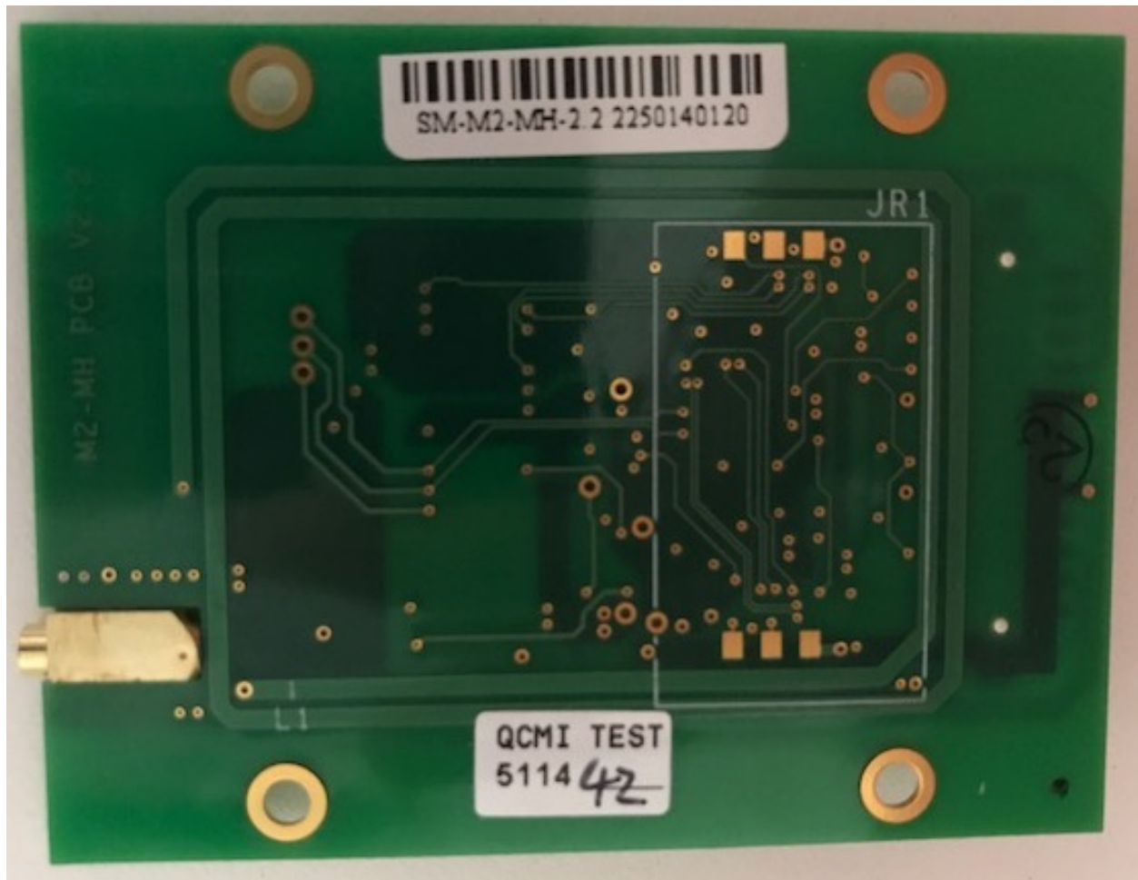
Bottom View: SkyeModule M2
