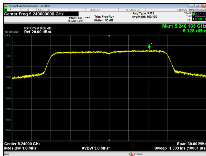
PSD NVHT n20 5240MHz Ant2
