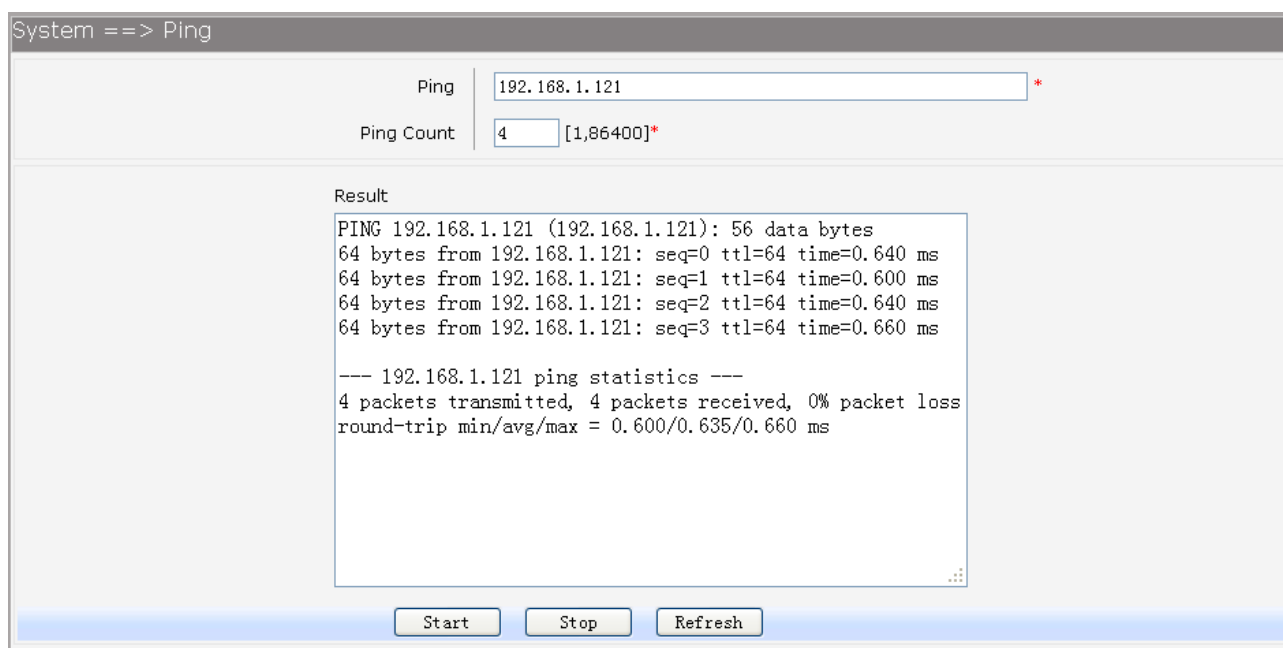
Figure 3-125 Ping Diagnostic
