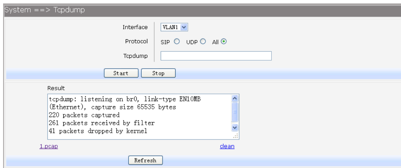
Figure 3-126 Tcpcdump Diagnostic
