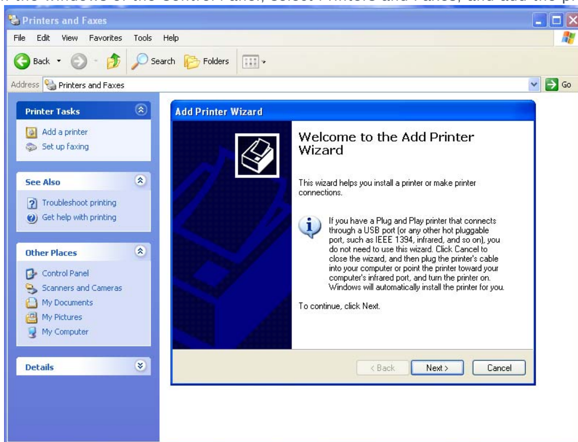
Figure 3-136 Add Printer
