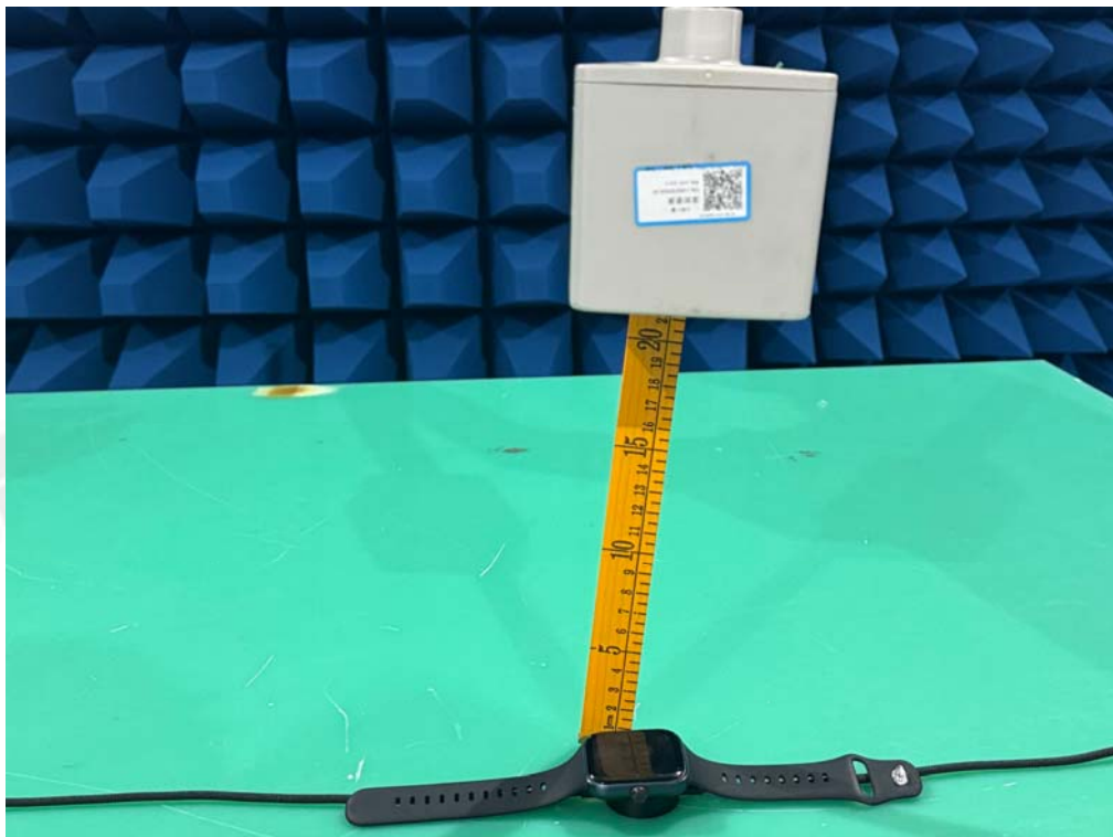
Portable exposure conditions Test Position A (20cm)
