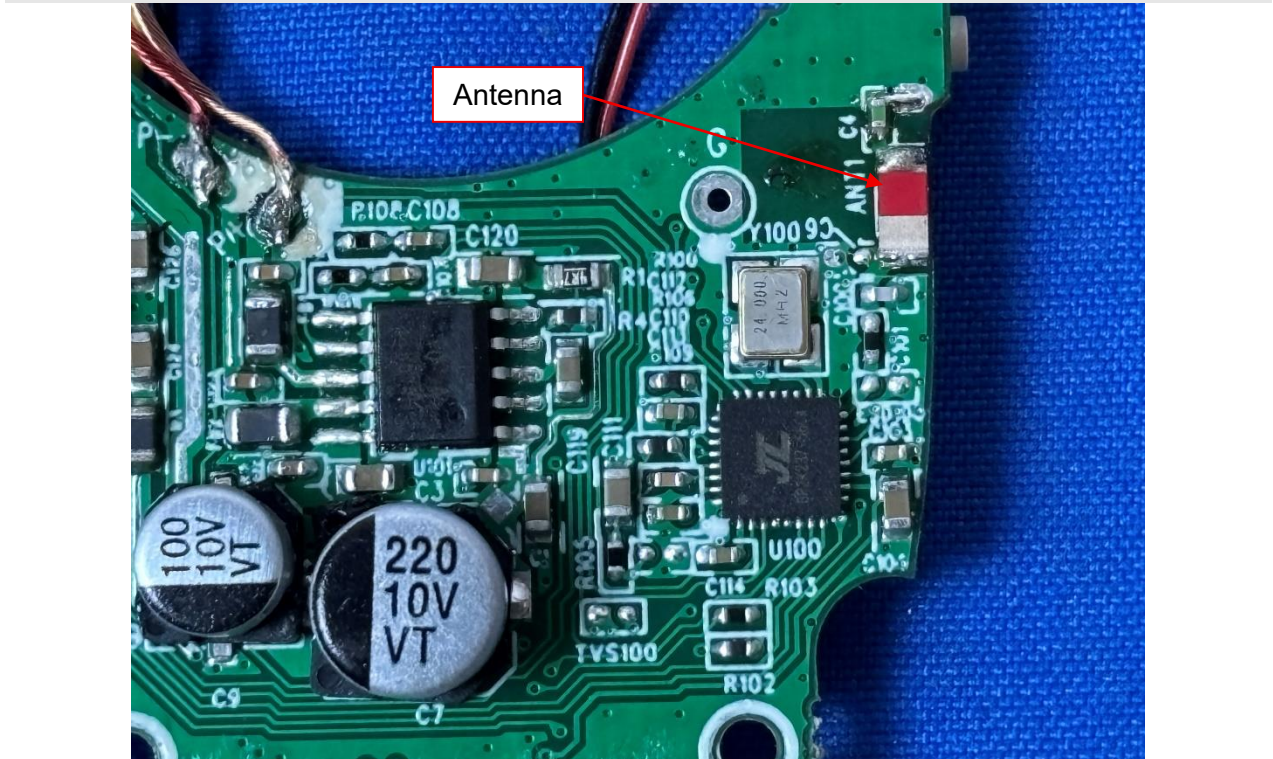
Internal View of EUT-5
