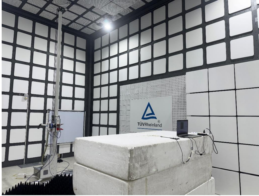
Photograph 10: Test Setup for Spurious Emissions (Back View 3)
