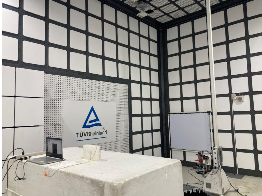
Photograph 13: Test Setup for Spurious Emissions (Back View 3)
