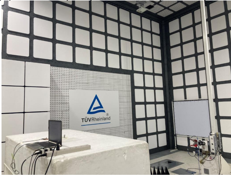
Photograph 24: Test Setup for Spurious Emissions (Back View 4)
