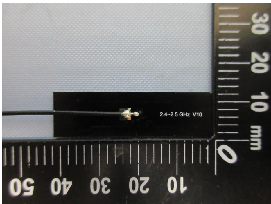
Ant 8, RFA-02-P33-D034
