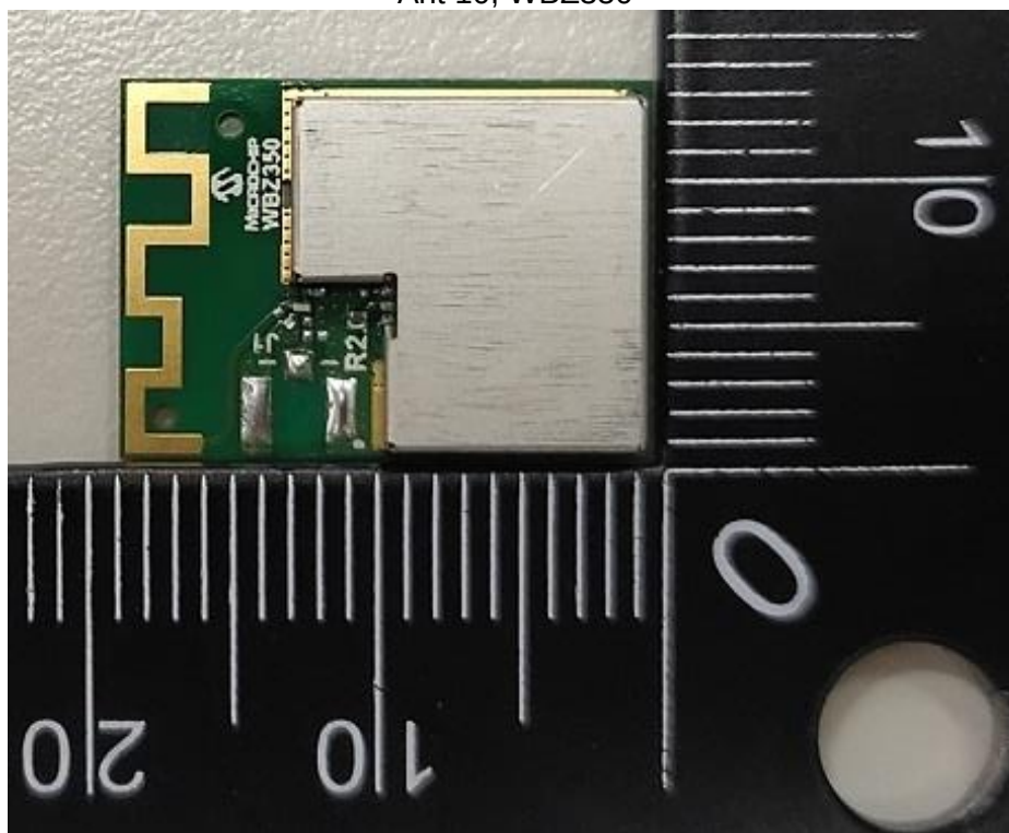
Ant 10, WBZ350
