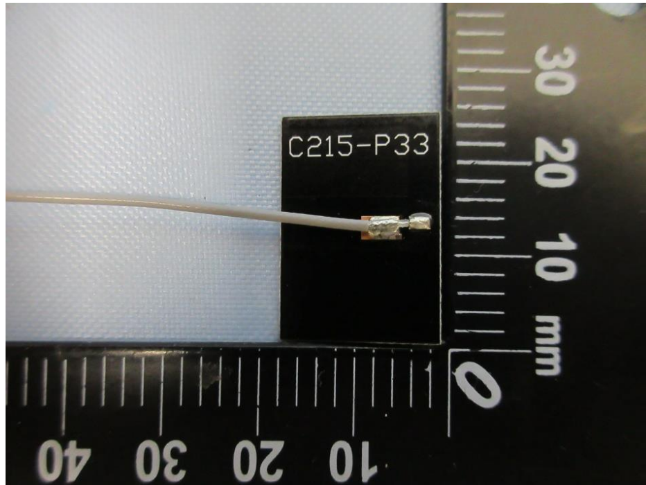
Ant 9, ABAR1504-S2450
