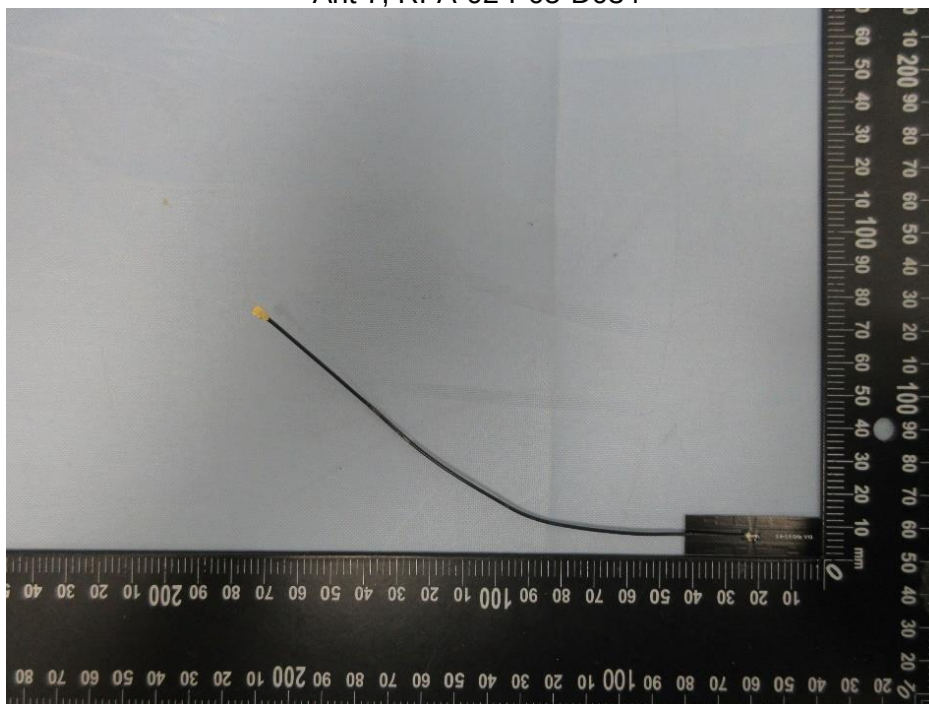
Ant 7, RFA-02-P05-D034
