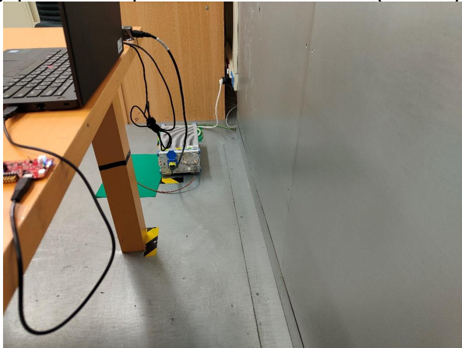
Photograph 14: Test Setup for Mains Conducted Emissions (Back View)
