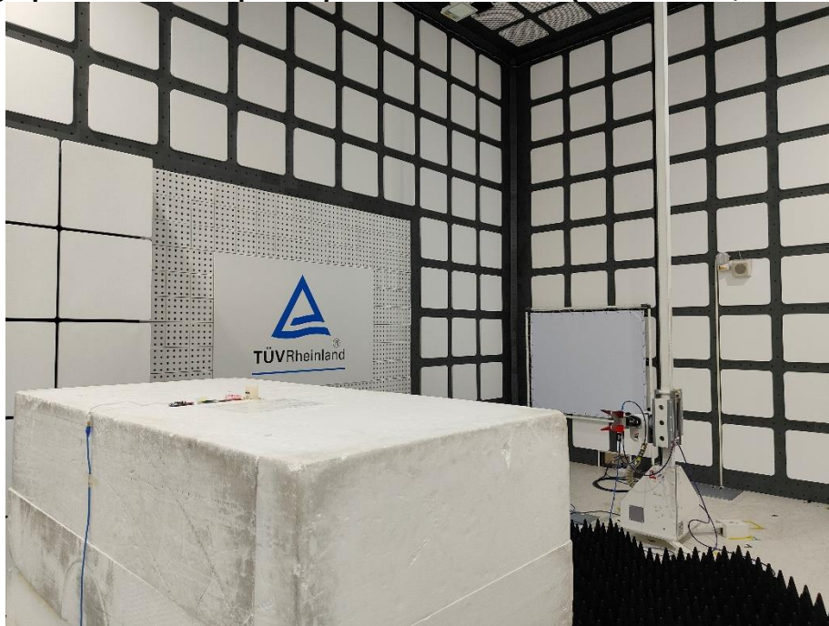
Photograph 19: Test Setup for Spurious Emissions (Back View 3, Main Source)
