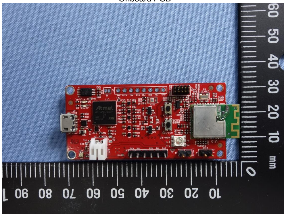
Onboard PCB
