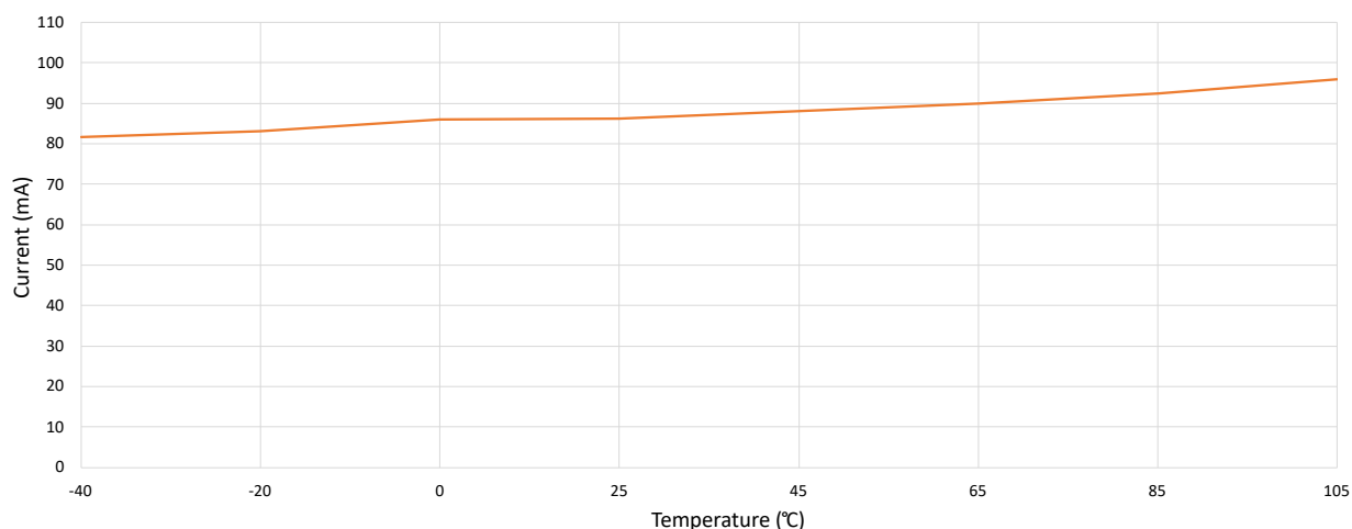
Figure 3-3. Receive Current vs Temperature, MCS7, Channel 7, 3.3V
