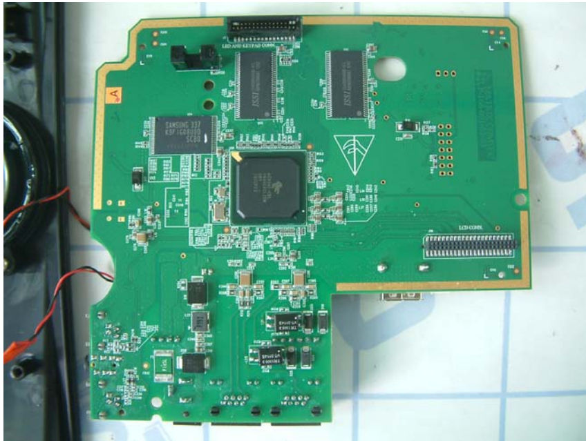
PCB 1 side 2
