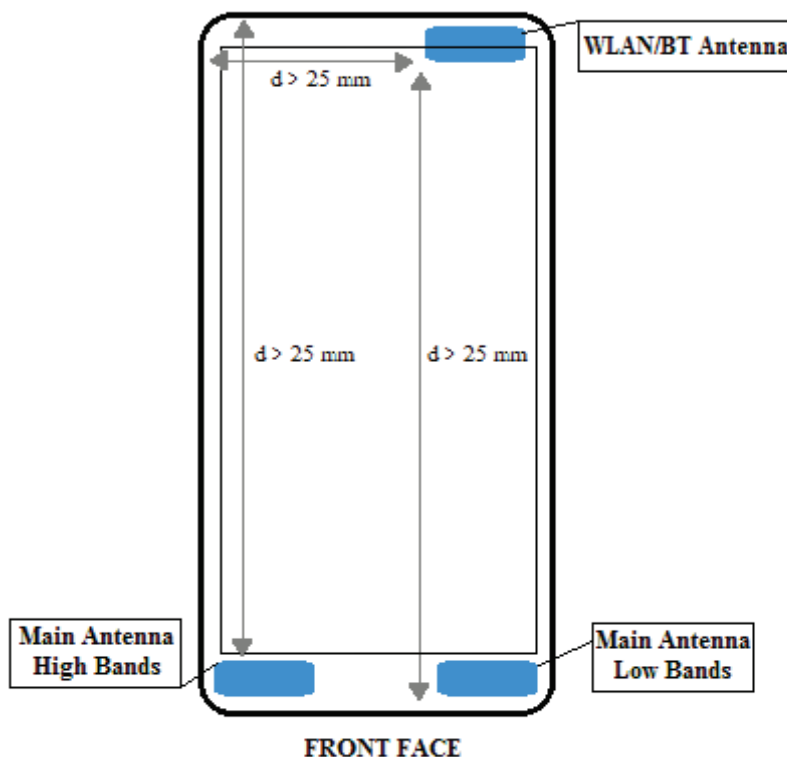
Figure 8: Antenna location.
