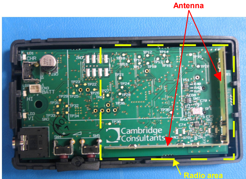
Receiver PCB Top View
