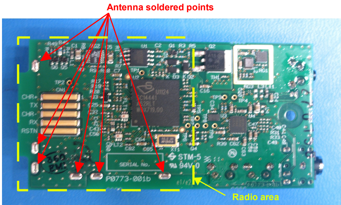
Receiver PCB Bottom View
