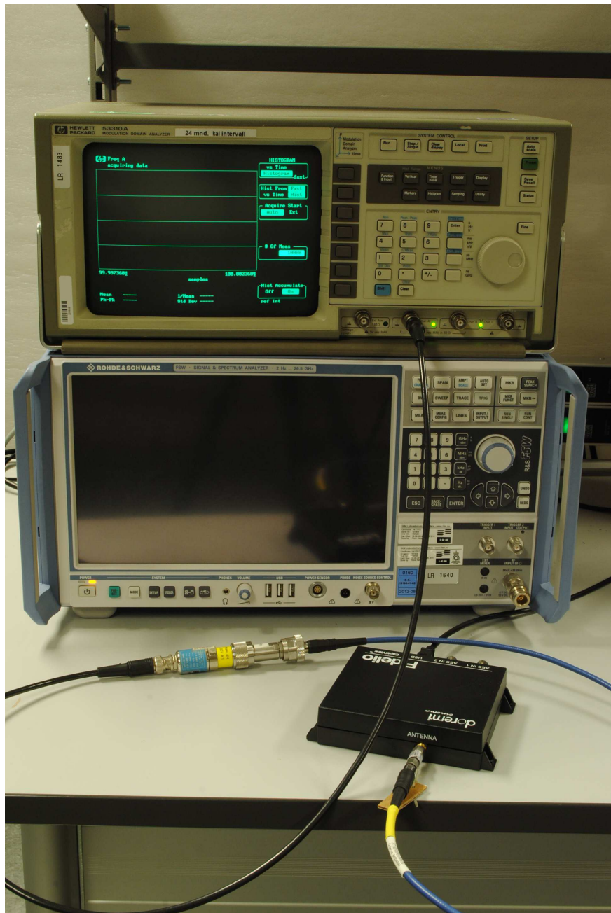
Timing Tests
