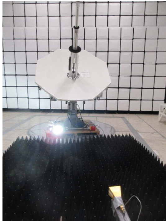
26.5 GHz to 40 GHz, Front View
