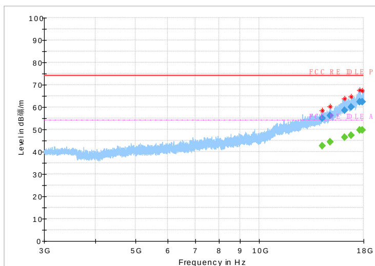
Fig.25 Radiated emission: Ch39, 3GHz~18GHz
