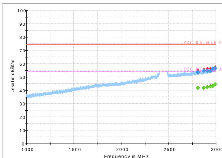
Fig.24 Radiated emission: Ch39, 1GHz~3GHz
