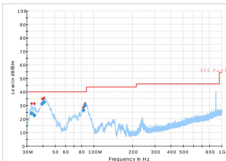
Fig.23 Radiated emission: Ch39, 30MHz~1GHz
