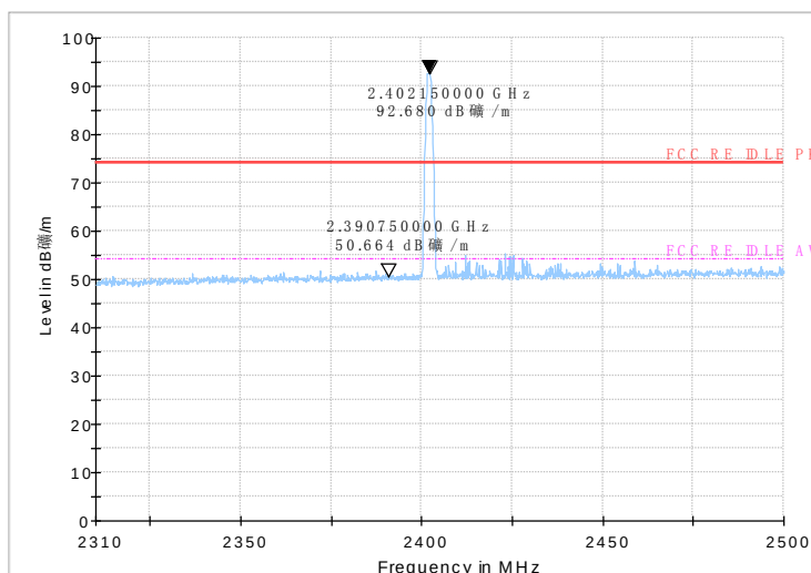
Fig.21 Radiated emission (Power): low channel
